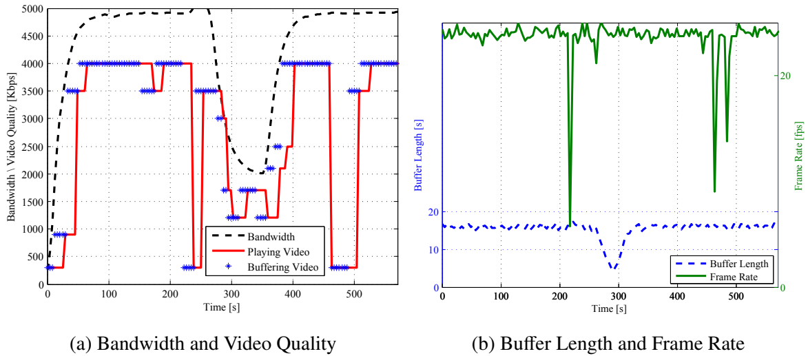
Figure 4.10 – Client Video Adaptive when Buffer=15
