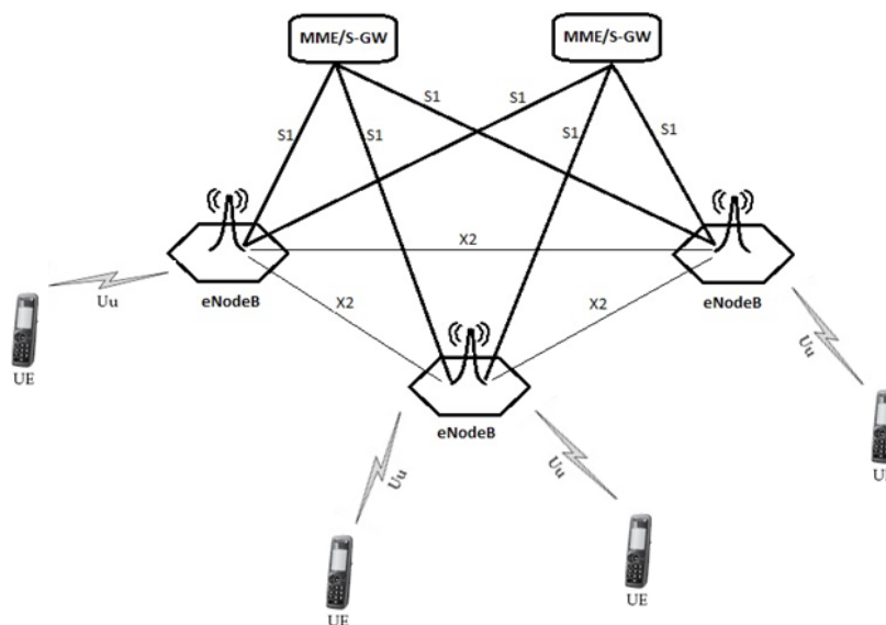
Figure 5.1 – LTE Architecture
