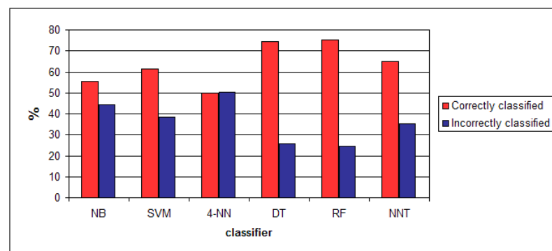
Figure 3.4 – Instance Classification
