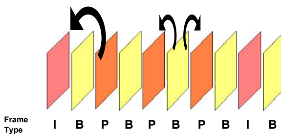
Figure 4.3 – H.264 Frame
