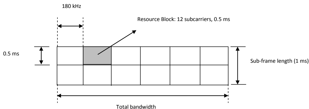
Figure 5.2 – LTE Frame Structure in Frequency Domain
