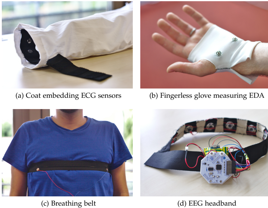
Figure 53: Wearable sensors
