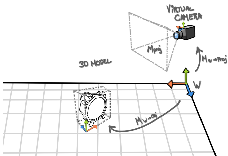
Figure 13: The virtual counterpart of the SAR pipeline shown in Figure 12. The 3D model of the real object is moved to the right location in virtual space M_{W \to Obj} as fed by the tracking solution. Then, a virtual camera is created using the parameters returned from the extrinsic ( M_{W \to Proj} ) and intrinsic ( M_{Proj} ) calibration of the projector. Finally, the image produced by the virtual camera is sent to the projector to create the augmented scene.
