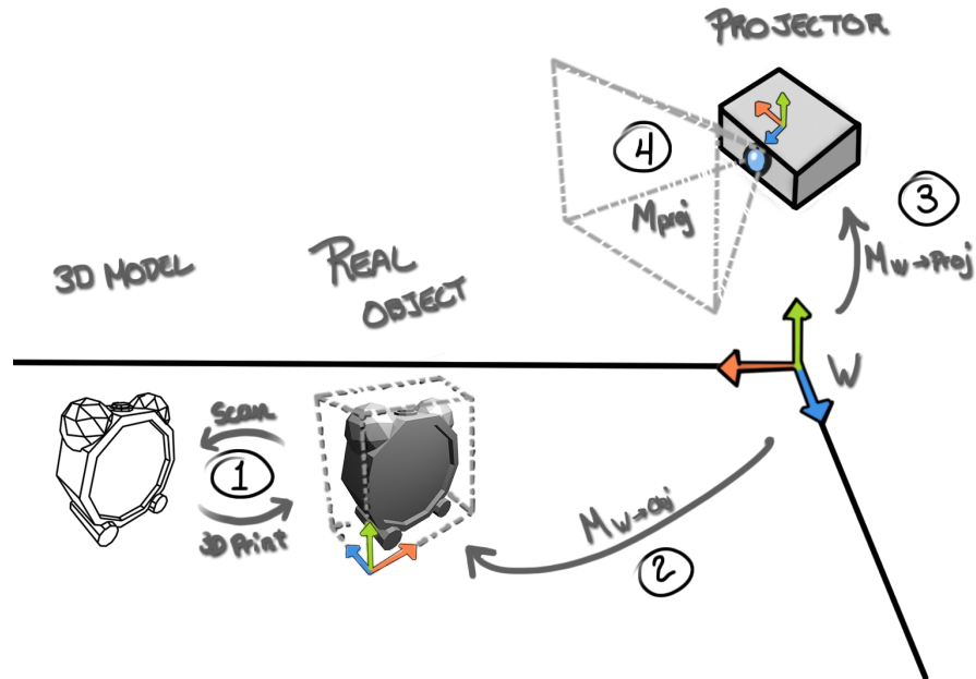
Figure 12: A summary of a SAR pipeline. W represents the world's coordinate system's origin. (1) The exact geometry of the augmented object must be known, either by using 3D scanning of an existing object or by creating a 3D model and building it using, for example, 3D printing. (2) The position and orientation of the object in world space ( M_{W \rightarrow Obj} ) must be known via a tracking solution or manual measurements. (3) The position and orientation of the projector in world space ( M_{W \rightarrow Proj} ) must also be known. (4) The intrinsic parameters of the projector ( M_{Proj} ) is required to know how the pixels are being distributed in the real-world environment.
