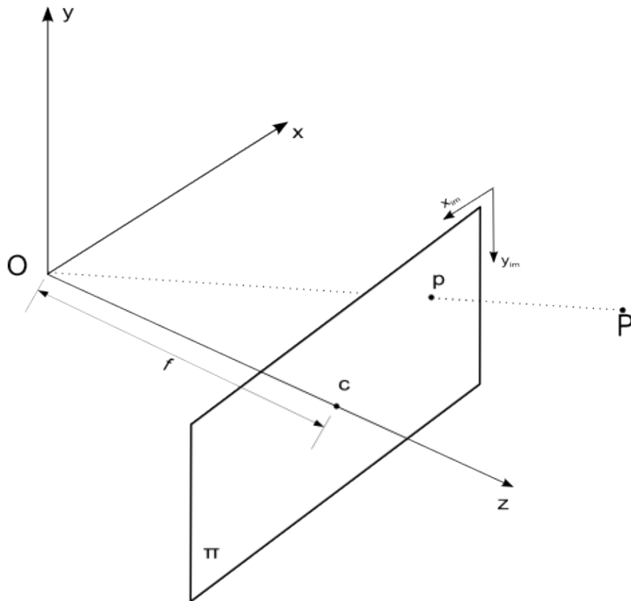
Figure 66: The pinhole or perspective camera model. The model consists of an image plane \pi and a 3D point O , representing the camera center or the focus of projection . The positive z axis that goes from O through the center c of the image plane is called the optical axis . A 3D point in the world P is projected on the image plane \pi at point p . x_{im} and y_{im} represents the coordinate system of the image.
