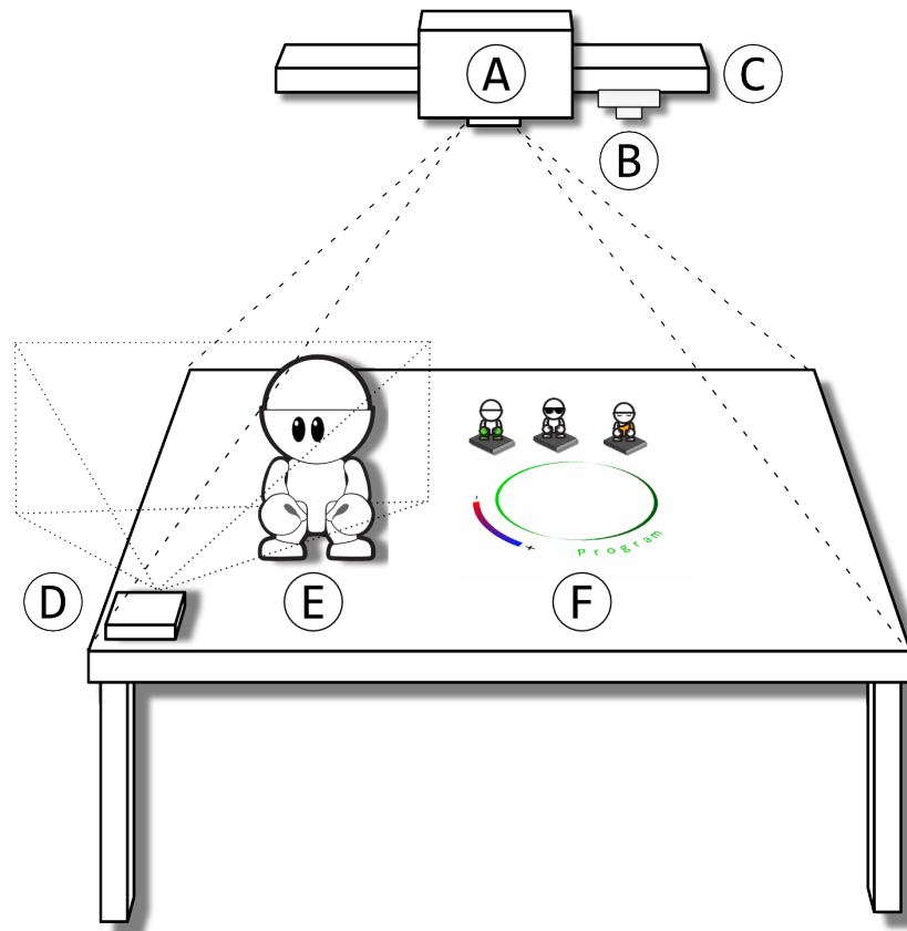
Figure 47: Diagram of the installation. (A) ProjectionDesign F2oSX projector (B) Sony PSEye web camera (C) OptiTrack V120:Trio (D) Vivitek Qumi Q2 projector (E) Teegi (F) Program selection zone and mini-Teegis.
