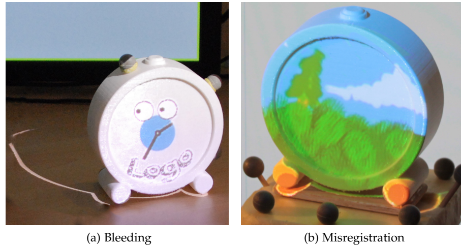
Figure 15: Typical artifacts encountered in SAR. (a) Bleeding of some of the projected pixels outside of the object’s surfaces. Here, bleeding can be seen as a white silhouette on the table. (b) Misregistration artifacts where part of the objects are clearly misaligned. The projection on the feet of the clock are offset from their intended position.
