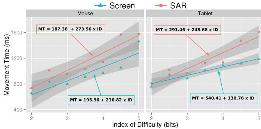
Figure 28: Fitts' law models. R^2 = 0.8479 .
