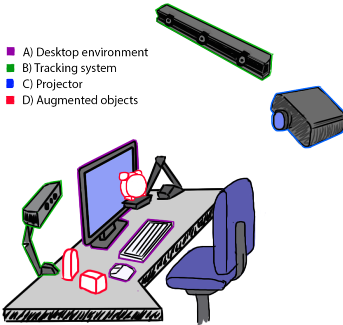
Figure 34: The SAR installation: A) The desktop environment using a standard screen and input devices, B) 6DOF tracking system (OptiTrack Trio and Microsoft Kinect v2), C) Projector and D) Physical objects that are being augmented.
