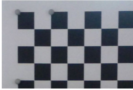
Figure 21: A chessboard pattern with reflective markers attached to it.
