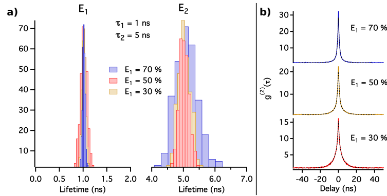
FIGURE 5.5: Monte Carlo simulations for \tau_1 = 1 ns and \tau_2 = 5 ns. a) Monte Carlo simulations for r_e = 0.3, 0.5 and 0.7 , were iterated 300 times, we show the histogram distribution of lifetimes \tau_1 and \tau_2 retrieved after a fit with equation 5.1. The time resolution was set to 100 ps, I = 5 pA, P_{int} = 1 and L/\lambda_e = 1 . b) Typical g^{(2)}(\tau) function for the three E_1/E_2 ratios presented in a).showing that measurements was done for a high signal to noise ratio.
