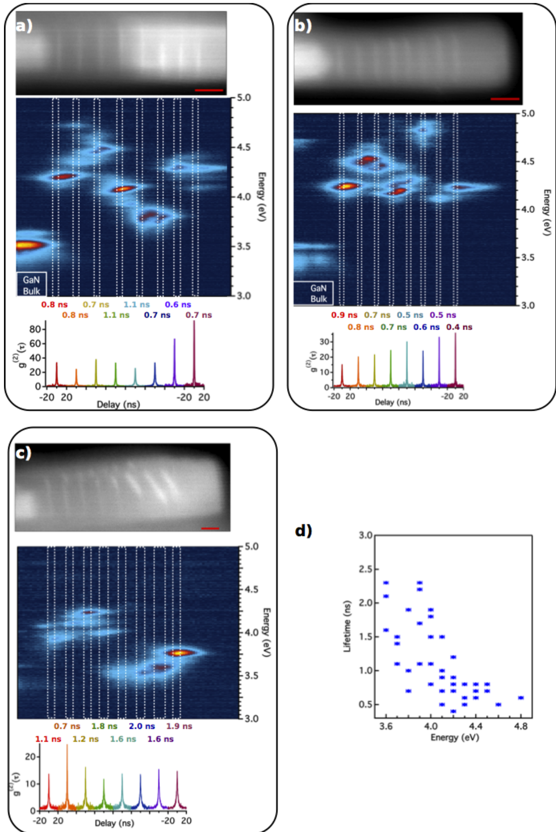
FIGURE 5.2: a), b), c) HADF image (top), projection of a SPIM (see chapter 2) along the growth direction (middle) and the correlation function g^{(2)}(\tau) taken on each QW (bottom). a: NW1; b: NW2; c: NW3. The dashed rectangles represent the QW location. Scale bar in the HADF is 20 nm. d) Lifetime as a function of the emission energy for the quantum wells taken from the fifteen nanowires studied. Only quantum wells with a clear single emission energy are reported.
