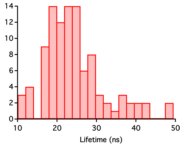
FIGURE 5.13: Distribution of the average lifetime measured on nano diamonds with about 900 centers per nanodiamond. 100 nanodiamonds have been measured with a fit accuracy better than 10 %.
