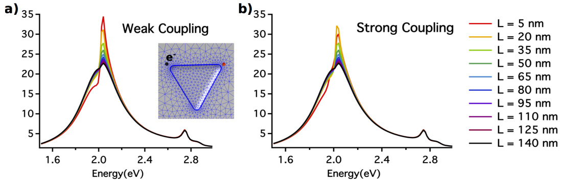
FIGURE D.3: a) weak coupling regime and b) strong coupling regime. The distance between the triangle corner and the emitter is changed (legend on the right). Insert of figure a) the simulated structure with the emitter in red and the silver nanotriangle. The emitter is put on the figure at 10 nm from the triangle corner.
