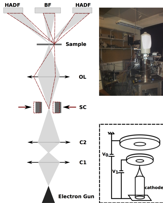
FIGURE 2.1: Sketch of an STEM VG HB 501. The electron gun at the bottom produces an electron beam at an energy between 40 and 100 keV. The sketch of the field emission (inside the electron gun) is shown at the bottom on the right. Magnetic lenses along the column are represented by horizontal arrows, C1 and C2 being the two condenser lenses and OL the objective lens. The beam is focused thanks to these three lenses on the sample in a probe of about 1 nm, the transmitted electrons are collected on the High Angular Dark Field (HADF) and Bright Field (BF) detectors. Thanks to the scanning coils (SC) the sample is scanned with the probe and a HADF and BF signals are recorded at each point. HADF and BF images are obtained after reconstruction of the image with the contrast in each points. Top right of the image, picture of the STEM VG HB 501. The white cylinder is a Deware for liquid nitrogen to cool down the microscope at 100 K.
