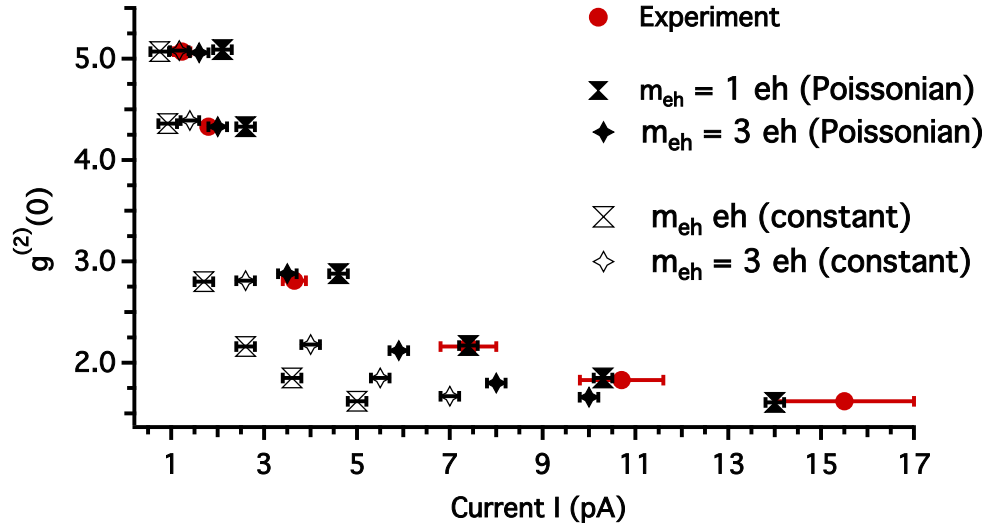
FIGURE 4.15: Comparison between the different Monte Carlo models for NV^0 . g_{CL}^{(2)}(\tau) calculated from Monte Carlo simulations within the two different models for the decay mechanism compared to experimental data points extracted from figure 4.14. For all the simulations, all parameters are fixed except the current. Error bars in the simulations are generated by introducing a \pm 1 ns error in the estimate of \tau_e and a very conservative \pm 10\% error on L/\lambda_e . The bunching effect is qualitatively reproduced by both models.
