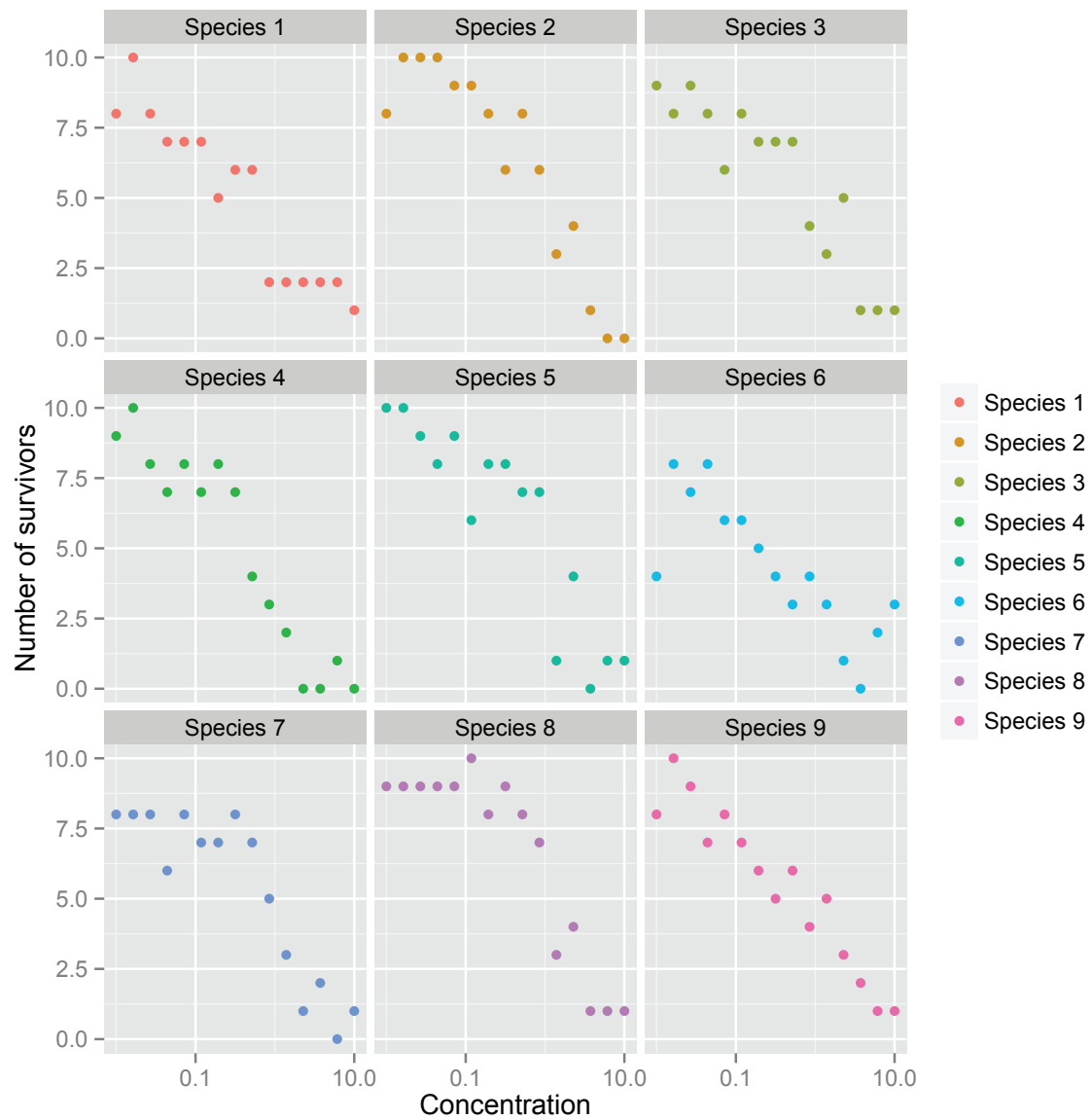
Figure 1.2: Survival as a function of the concentration in contaminant for 9 simulated species.
