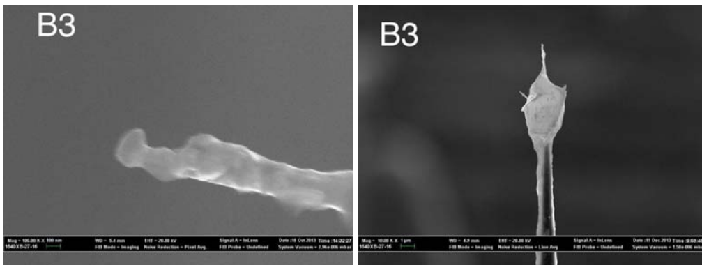
Figure B.11 – Left: SEM image of tip B3 before laser irradiation. Right: SEM image of tip B3 after laser irradiation.
