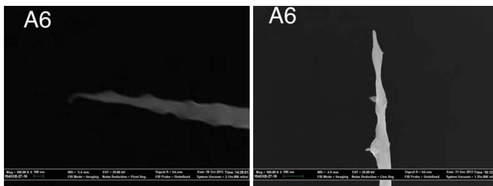
Figure B.7 – Left: SEM image of tip A6 before laser irradiation. Right: EM image of tip A6 after laser irradiation. Notice the new shape that is much blobbier than before.
