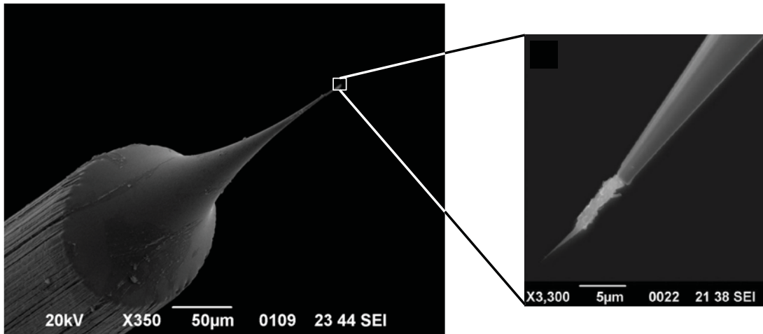
Figure 3.10 – SEM images showing a finished CCnT welded onto a tungsten tip.
