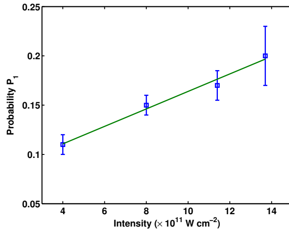
Figure 7.2 – The linearity of the probability of photon absorption with the applied intensity of the laser.
