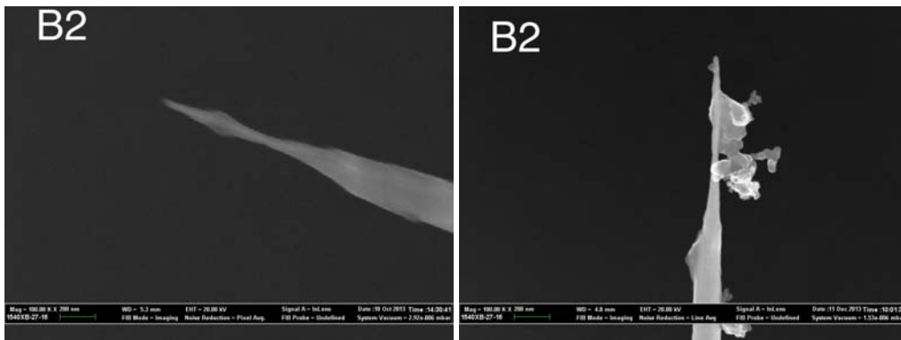
Figure B.10 – Left: SEM image of tip B2 before laser irradiation. Right: SEM image of tip B2 after laser irradiation.
