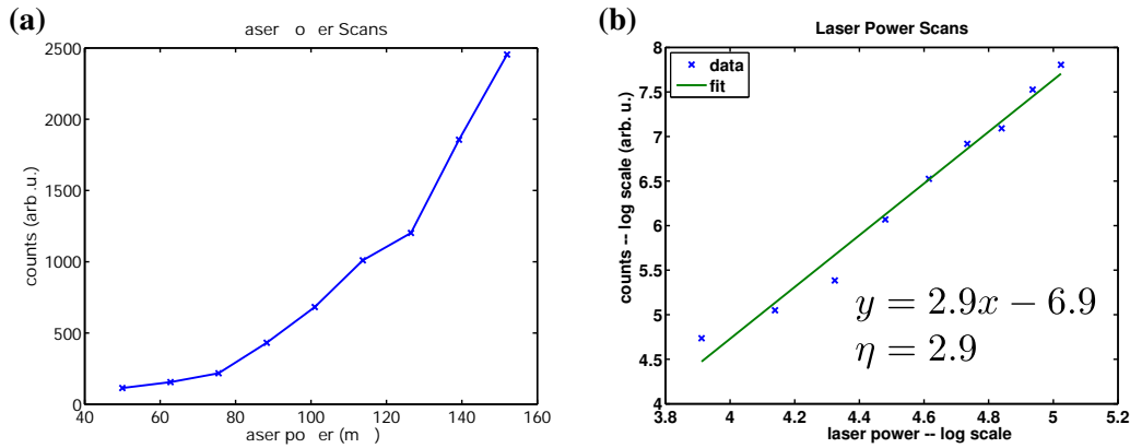
Figure 4.8 – (a) This shows the electron yield as a function of laser power for V_{\text{tip}} = 50 V. (b) This shows the same yield on a log-log scale. We can fit this curve to a linear equation from which the slope is the power exponent we wish to extract.
