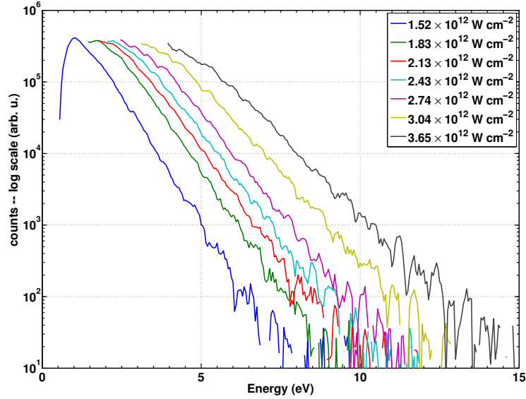
Figure 6.9 – Photoelectron spectra for laser intensities of \{1.52, 1.83, 2.13, 2.43, 2.74, 3.04, 3.65\} \times 10^{12} \text{ W cm}^{-2} , with V_{\text{tip}} = 20 \text{ V} . The spectra are narrower than those from equivalent intensities from tungsten nanotips, but the electron yield reached saturation on the MCPs. These saturation effects have been removed from the spectra.
