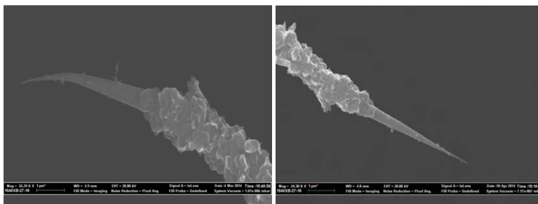
Figure C.7 – Tip 3 was illuminated with 9.0 \times 10^{11} \text{ W cm}^{-2} for 1 hour with no bias. Note the curved structure of the CCnT before irradiation. Left: Tip 3 before irradiation. Right: after irradiation. No signs of damage.
