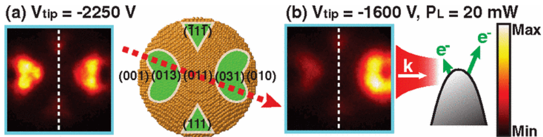
Figure 1.13 – (a) This shows emission sites from a (011) oriented W nanotip illustrating that the (310) facet has the most intense electron emission. The schematic shows the crystal facet orientations of the nanotip. (b) This shows the emission patterns with laser irradiation. The schematic shows the side view of the laser-induced field-emission geometry. Reprinted figure with permission from H. Yanagisawa et al. Phys. Rev. Lett. 103 (25) 257603, 2009. © (2009) by the American Physical Society. [Yanagisawa09]
