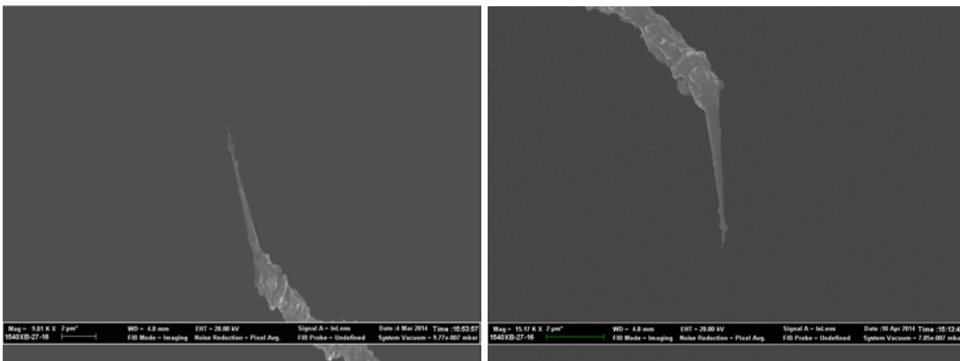
Figure C.8 – Tip 4 was illuminated with 2.7 \times 10^{11} \text{ W cm}^{-2} for 1 hour with no bias. Note the dust on the CCnT before and after irradiation. Left: Tip 4 before irradiation. Right: after irradiation. No signs of damage.
