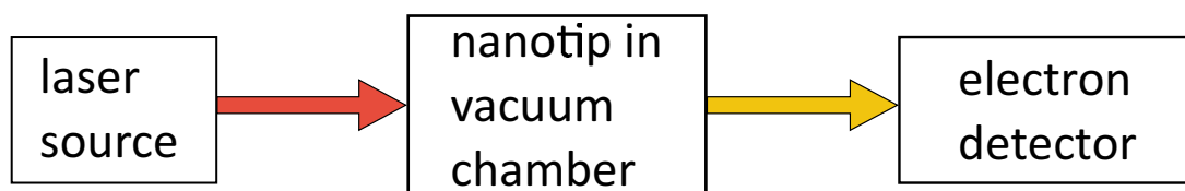
Figure 3.1 – This shows the basic flow of the experiment. A sharp nanotip placed in a vacuum chamber is illuminated by a laser source. The resulting electron emission is then detected by an electron spectrometer.
