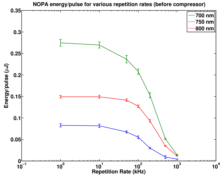
Figure 2.13 – NOPA energy measurements for different repetition rates at 700 nm, 750 nm and 800 nm.
