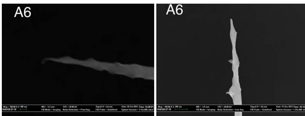
Figure B.7 – Left: SEM image of tip A6 before laser irradiation. Right: SEM image of tip A6 after laser irradiation. Notice the new shape that is much blobbier than before.
