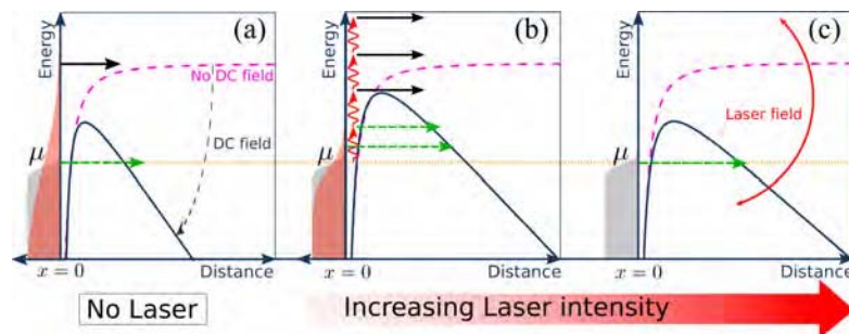
Figure 1.15 – Schematic showing the mechanisms behind laser induced electron emission from a system. The Fermi energy level, \mu , and distribution is shown in gray, with the redistribution of the energies due to thermal effects shown in red. The metal/vacuum interface is located at x = 0 . (a) This shows cold field tunneling (green dashed arrow) and thermal emission (black arrow) that take place without laser illumination. (b) This shows emission processes for low laser illumination. The laser pulses can be thought of from the photon point of view. If a sufficient number of photons are absorbed, an electron can escape over the potential barrier (black arrows), if not an electron can be emitted via assisted tunneling by absorption of a photon or thermal absorption of the energy of a photon (green dashed arrows). (c) At high laser intensities, the laser field modifies the potential barrier itself and electrons can emit via optical tunneling.
