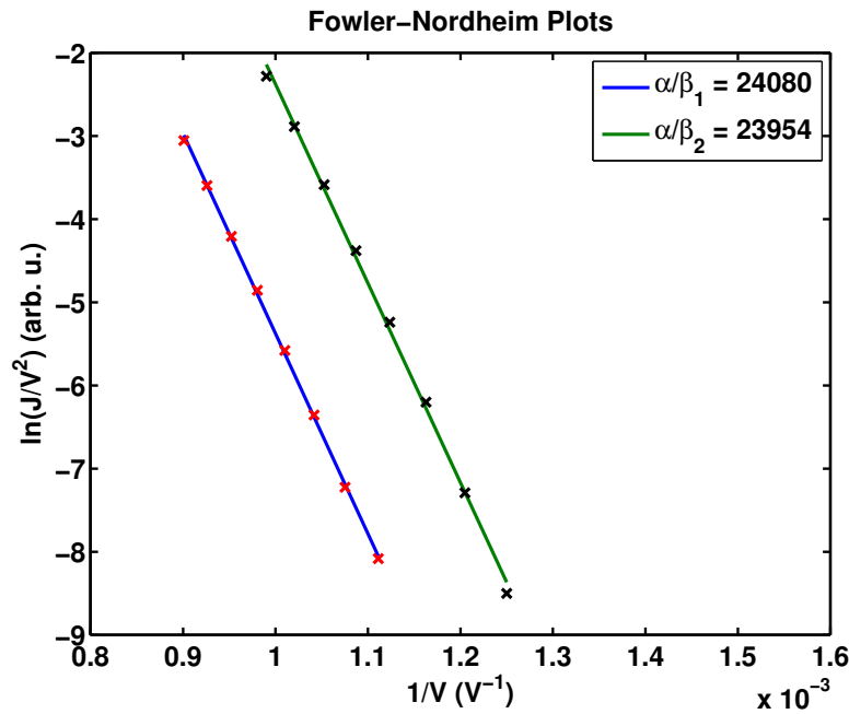
Figure 6.5 – This shows FN curves for two facets from polycrystalline silver.
