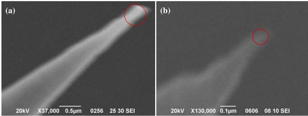
Figure 4.2 – This shows SEM images of the tips whose FN plots are given in Fig. 4.1 (a) This shows an SEM of a PCW nanotip. The tip apex is measured to be r < 250 \text{ nm} (red circle) in agreement with the FN calculations. (b) This shows the SEM of the apex of a SCW(310) nanotip. The tip apex is measured to be r < 50 \text{ nm} (red circle) as given by the FN calculations.
