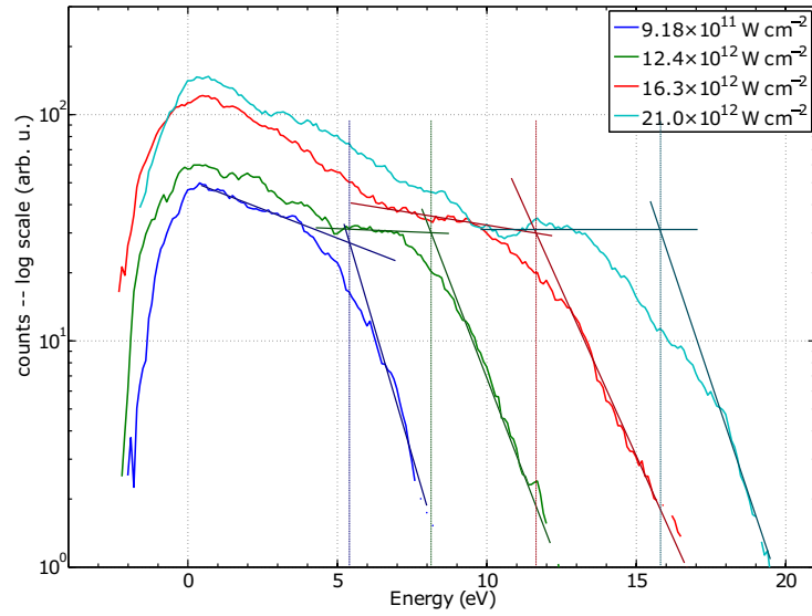
Figure 6.13 – Photoelectron spectra from Fig. 6.12 measured relative to the Fermi energy, eV_{\text{tip}} + U_p (from Tab. 6.2). The energy cutoff energy can be determined by the dropoff from the plateau at the for the higher energy electrons.
