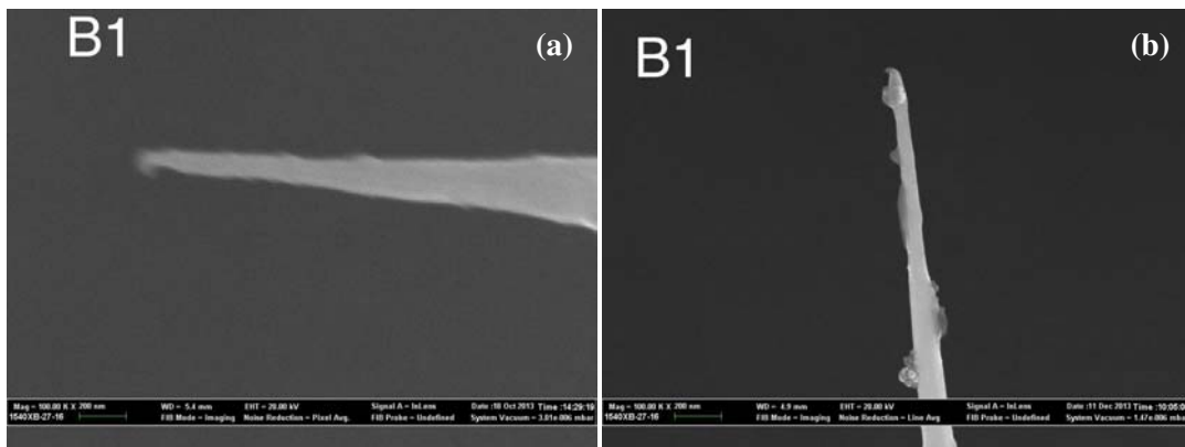
Figure 4.4 – (a) A SEM of tip B1 before laser irradiation. (b) SEM of the same tip after irradiation with 200 mW of average power for 24 hours with a focal spot size of \sim 25 \mu\text{m} , corresponding to a peak intensity of 3.29 \times 10^9 \text{ W cm}^{-2} . No visible damage is seen.
