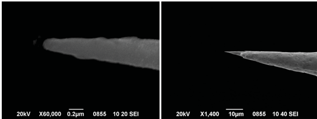
Figure 6.2 – SEM images of the first Ag tip after laser irradiation. No indications of damage or oxidation.
