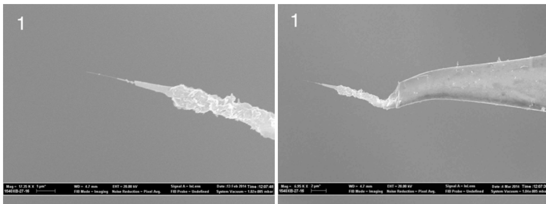
Figure C.1 – Tip 1 was not illuminated with any laser. Note the incomplete structure of the CCnT and the protruding central CNT. Left: Tip 1 before test. Right: after tests. No signs of damage
