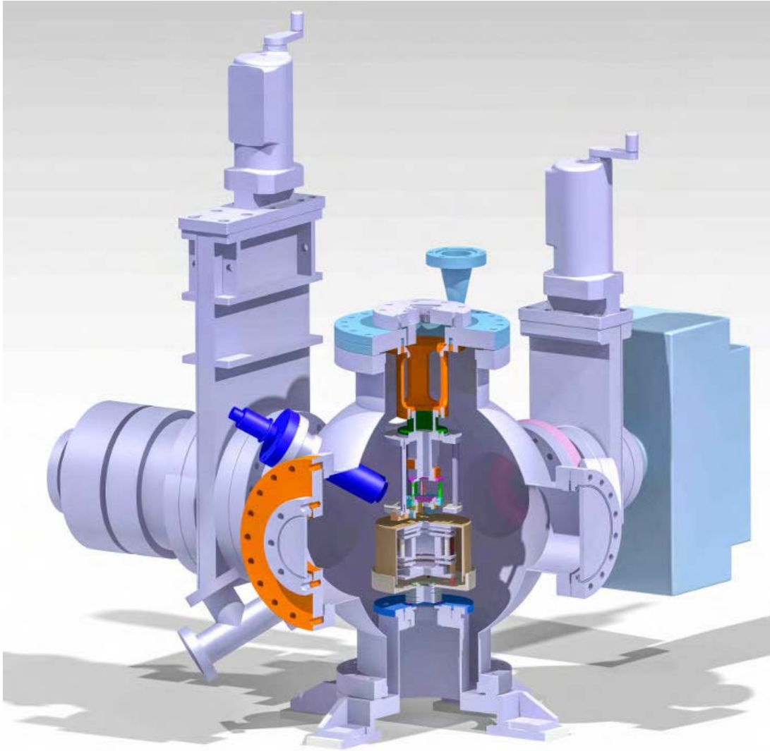
Figure 3.12 – Schematic of the UHV chamber and components used for our experiments.
