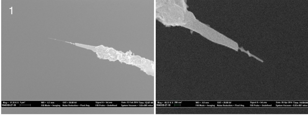
Figure 5.10 – The left panel shows the CCnT nanostructure before laser irradiation. The right panel shows the SEM inspection of the tip after 2.7 \times 10^{11} \text{ W cm}^{-2} with a 50 V bias. The protruding central CCnT is no longer observable possibly due to damage caused by irradiation of the laser.
