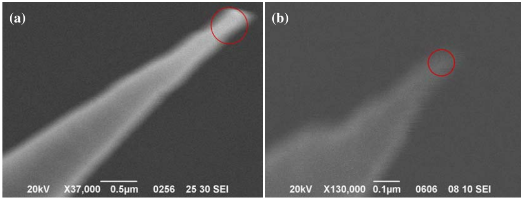
Figure 4.2 – This shows SEM images of the tips whose FN plots are given in Fig. 4.1 (a) This shows an SEM of a PCW nanotip. The tip apex is measured to be r < 250 nm (red circle) in agreement with the FN calculations. (b) This shows the SEM of the apex of a SCW(310) nanotip. The tip apex is measured to be r < 50 nm (red circle) as given by the FN calculations.
