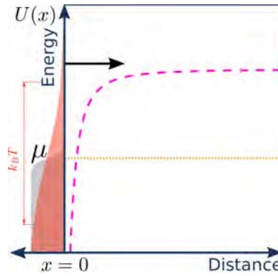
Figure 1.4 – This shows the thermionic emission process where the system is heated enough that some of the excited electrons have enough energy to overcome the work function and classically escape. Note there is no externally applied DC field.
