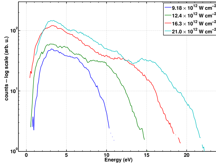
Figure 6.15 – Photoelectron spectra from Fig. 6.12 measured relative to the corrected Fermi energy, U_p (from Tab. 6.2) + eV_{tip} + 2.59 eV.
