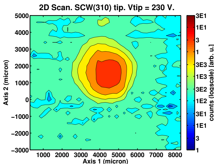
Figure 4.3 – This shows FEM (spatially resolved emission) for a single crystal tip, with r = 50 nm. The W(310) facet has the lowest work function of all so emits at the lowest threshold and has a higher electron yield than the other facets.
