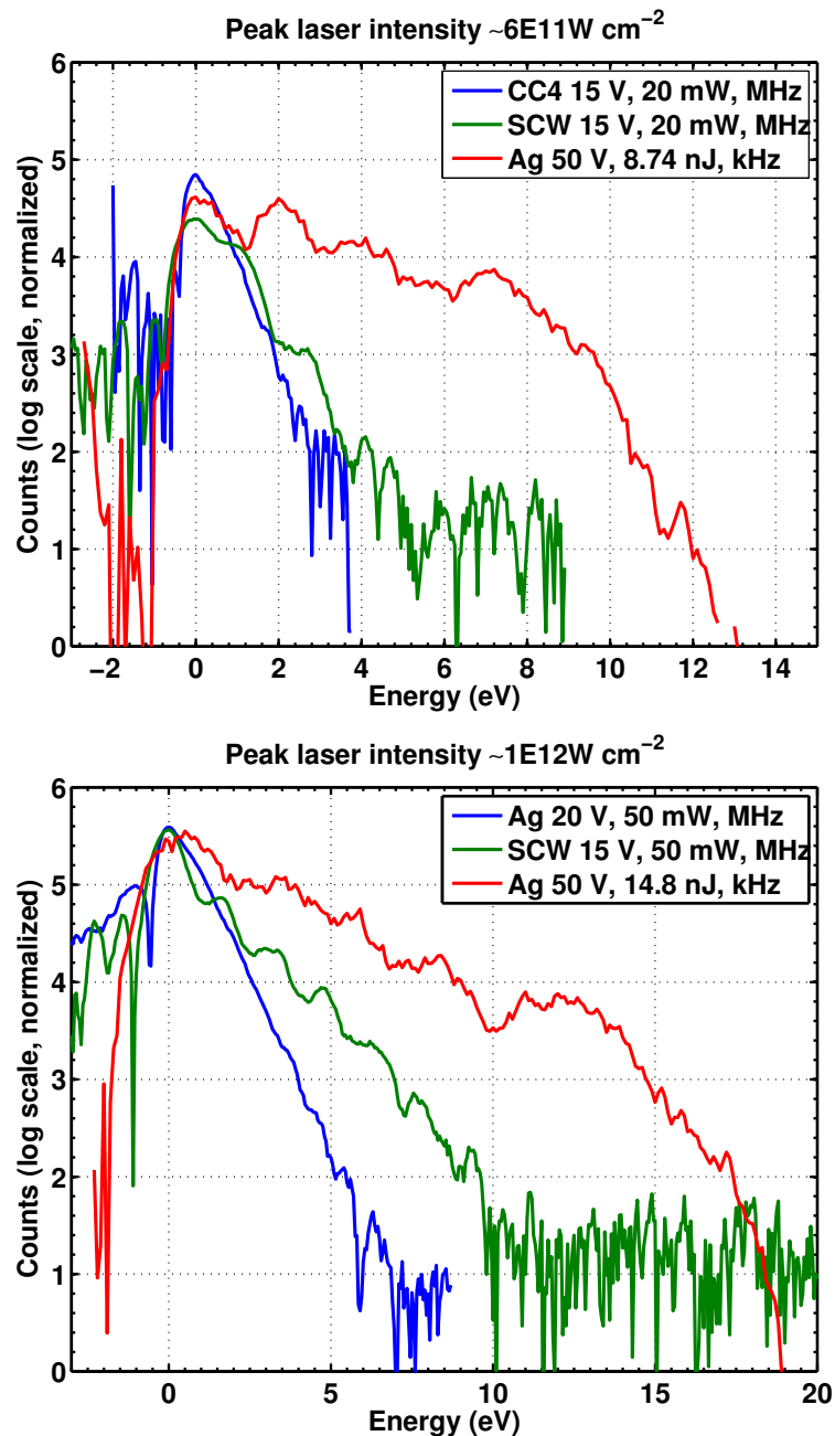
Figure 7.4 – Each set of spectrum were taken with the same applied peak laser intensity: top 6 \times 10^{11} W cm^{-2} , bottom 1 \times 10^{12} W cm^{-2} . Changing the tip material or laser repetition rate (mean power) changes the dominant emission mechanism. The blue spectra show narrower spectra indicating thermally enhanced field emission. The green spectra show multiphoton emission characterized by ATP peaks separated by the photon energy. The red spectra show much broader energies indicating a transition into the optical tunneling regime and the emergence of a spectral plateau for high intensity evidencing electron recollision and rescattering.
