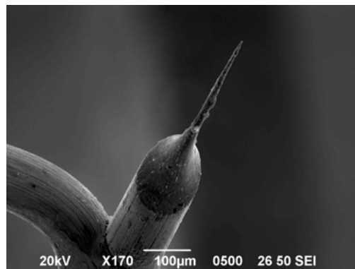
Figure 3.6 – This shows an example of a failed etch of W tip.
