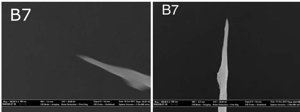
Figure B.15 – Left: SEM image of tip B7 before laser irradiation. Right: SEM image of tip B7 after laser irradiation.
