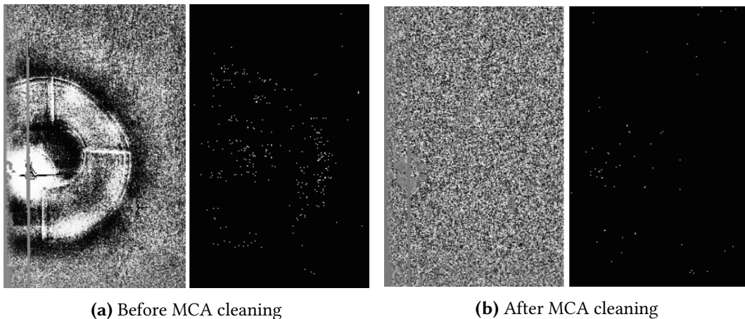
Figure A.1: Image stack for field D 4 (left) and its corresponding detection map (right) before (a) and after (b) MCA cleaning. Before cleaning, detections clearly follow the shadow of the star while after cleaning most of these spurious detections are eliminated.
