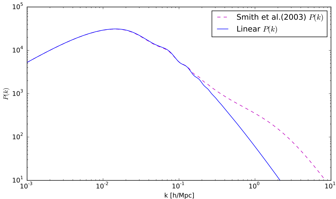
Figure 2.4: Matter power spectrum as a function of scale factor. The linear power spectrum computed with the fitting formula from Eisenstein and Hu (1998) is compared to the non-linear power spectrum computed following Smith et al. (2003). In both cases, BAOs are causing characteristic wiggles on the power spectrum.
