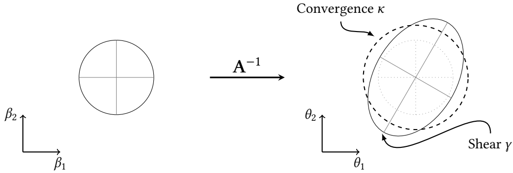
Figure 6.3: Deformation of a circular source under the effect of the amplification matrix \mathbf{A} . The effects of the anisotropic shear and isotropic convergence are separated.
