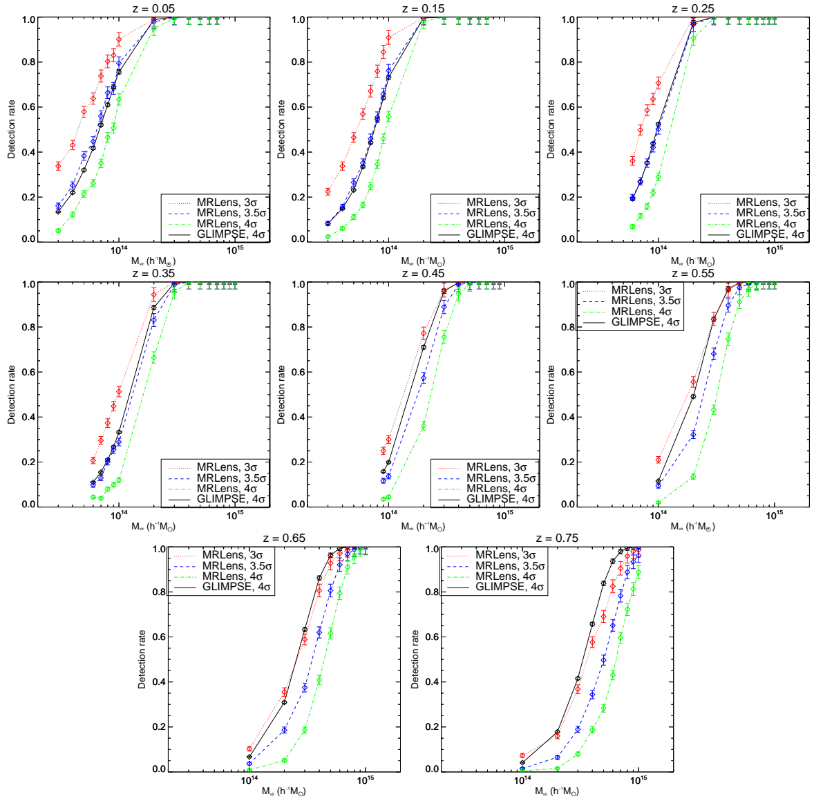
Figure 8.14: Detection rate of the central cluster using MRLens (blue) and GLIMPSE (black) for different cluster redshifts. The parameters of the two methods are calibrated to yield a similar false detection rate. At low redshift, the detection rates are similar but at high redshift, GLIMPSE clearly outperforms MRLens.
