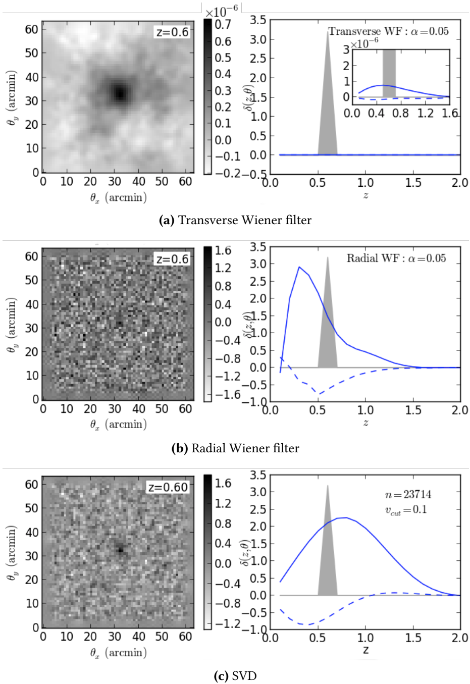
Figure 6.11: Reconstruction of a 10^{15} M_{\odot} cluster at redshift z = 0.6 using the 3 linear inversion methods. The noise level corresponds to a survey with n_{gal} = 30 \text{gal/arcmin}^{-2} and \sigma_{\epsilon} = 0.25 . The left panels show a slice in the 3D reconstructed density contrast at z = 0.6 . The right panels show the central line of sight in the reconstruction. The gray wedges show the input density contrast and the solid blue lines show the E-mode signal and the dashed line show the B-mode signal.
