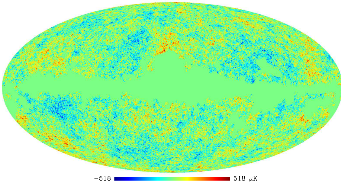
Figure 5.1: A simulated noisy CMB map at 15 arcmin resolution obtained from LGMCA and masked with the WMAP kq85 mask. The noise level corresponds to the WMAP nine-year data. This map was generated from a CMB power spectrum for a primordial spectrum with n_s = 0.972 and \alpha_s = 0 .
