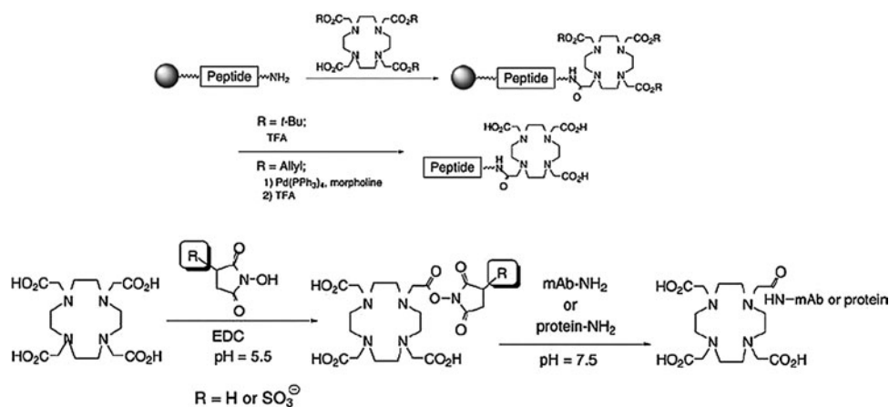
FIG. 3. (Up) Pathways of synthesis using tris-tert-butyl-DOTA and tris allyl-DOTA. (Down) Reaction using DOTA-OSSU. Image taken from Tanaka and Fukase. Reproduced by permission of The Royal Society of Chemistry.
