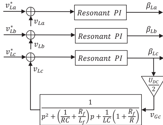
Figure IV.14: Load-connected converter low level control scheme.
