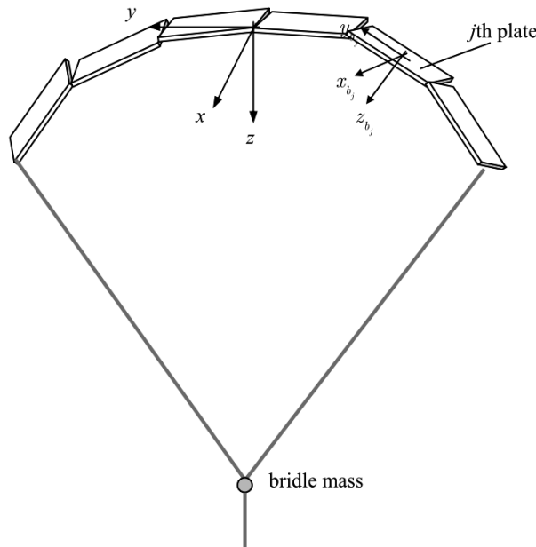
Figure II.6: Presentation of the kite's multi-body model [WLR08].
