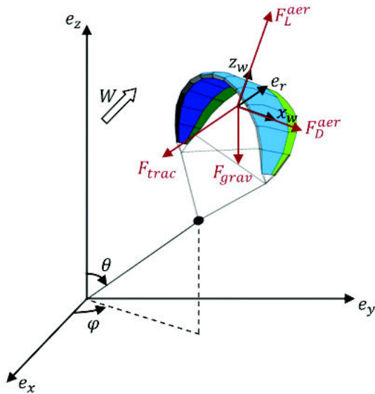
Figure II.8: Kite's main forces.
