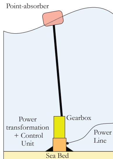
Figure V.1: The HPS simplified structure.
