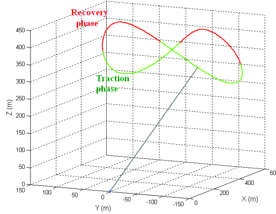
Figure I.19: Closed-orbit mode.
