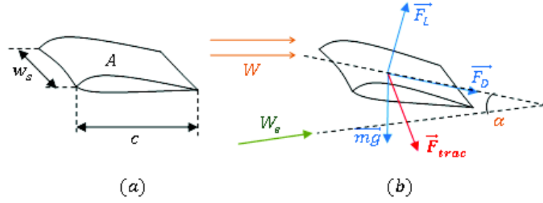
Figure II.2: Kite's main parameters and forces.
