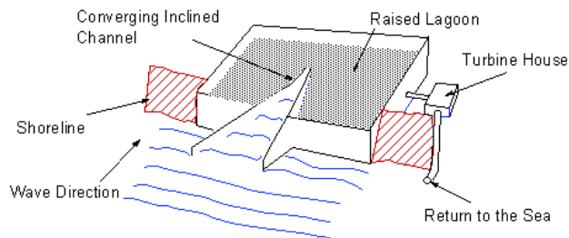
Figure I.25: TAPCHAN: Tapered Channel wave energy.
