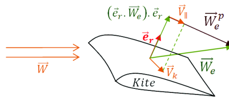
Figure I.16: Refined crosswind law.
