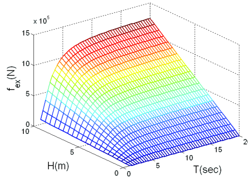
Figure II.16: The resulted excitation force as a function of the wave parameters.
