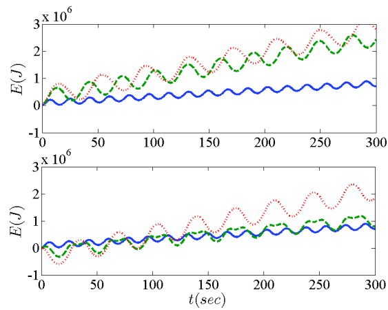
Figure III.7: KGS energy generation. Reference orbit (1): continuous. Upper plot: orbit (2) energy profile in dotted line, orbit (3): dashed. Lower plot: orbit (4) energy profile in dotted line, orbit (5): dashed.
