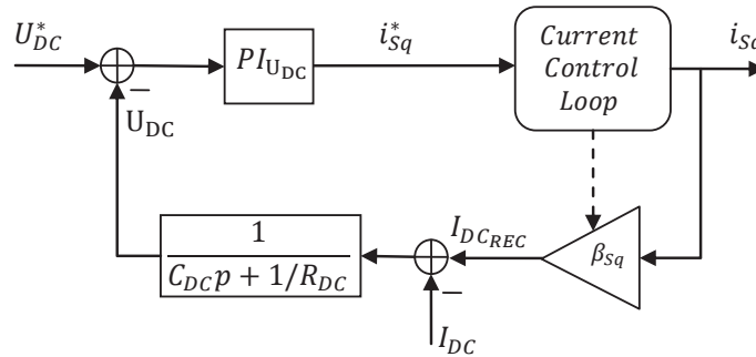
Figure IV.15: Machine-connected converter Intermediate level control scheme.
