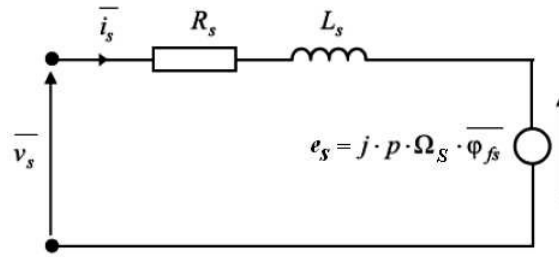
Figure IV.3: PMSM's Behn-Eschenburg equivalent electrical model.
