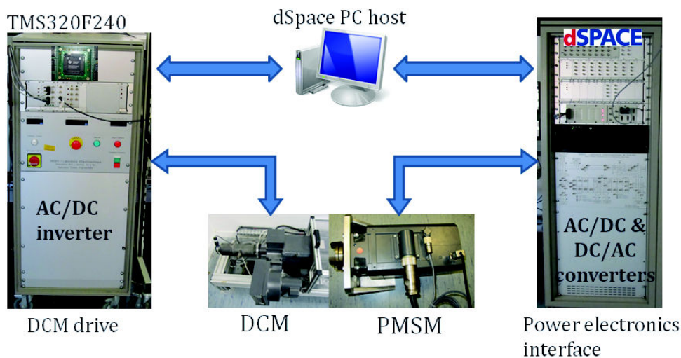
Figure IV.16: PHIL Simulator
