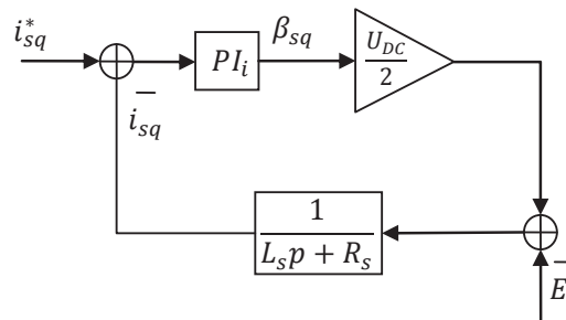
Figure IV.7: Low level control scheme for the machine-side converter.
