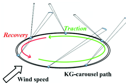
Figure I.20: Simplified presentation of the carousel of Kite-GEN
