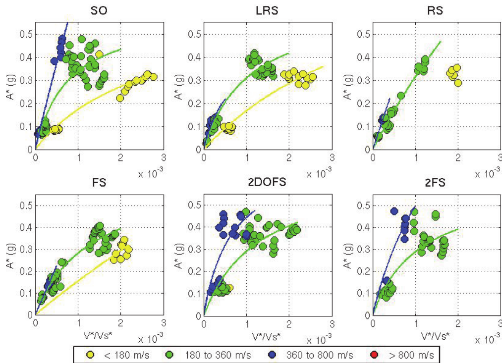
Figure 4.6. A^*-V^*/V_s^* curves for different velocity groups and type of structures. (SO: Soil Only; LRS: Low Rigid; RS: Rigid; FS: Flexible; 2DOFS: Two degree-of-freedom flexible; 2FS-1 and 2FS-2: two adjacent flexible).
