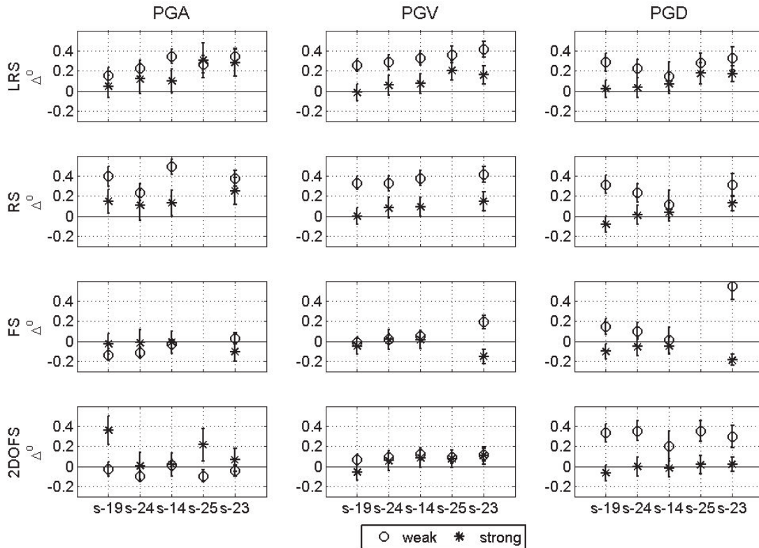
Figure 4.21. \Delta^o of the PGA, PGV, and PGD of the free-field sensors for LRS, RS, FS, and 2DOFS. Vertical lines are the standard derivation of the \Delta^o . The black line indicates the zero value. The circle shows the weak excitation and asterisk shows the strong excitation
