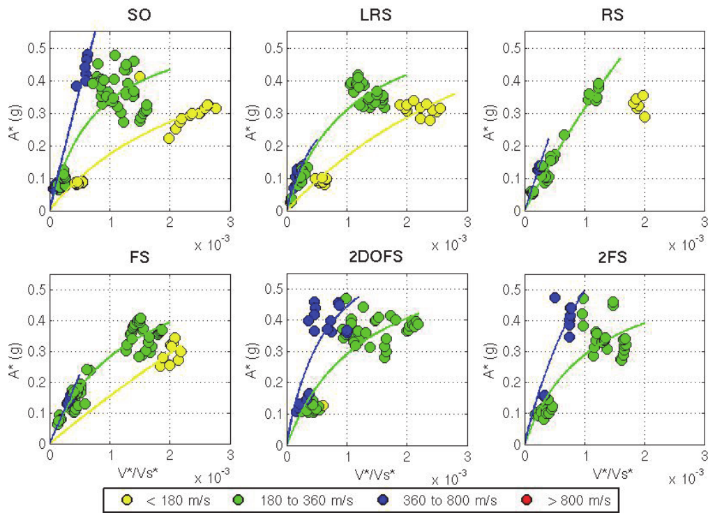
Figure 4.6. A^*-V^*/V_s^* curves for different velocity groups and type of structures. (SO: Soil Only; LRS:Low Rigid; RS: Rigid; FS: Flexible; 2DOFS: Two degree-of-freedom flexible; 2FS-1 and 2FS-2: two adjacent flexible ).
