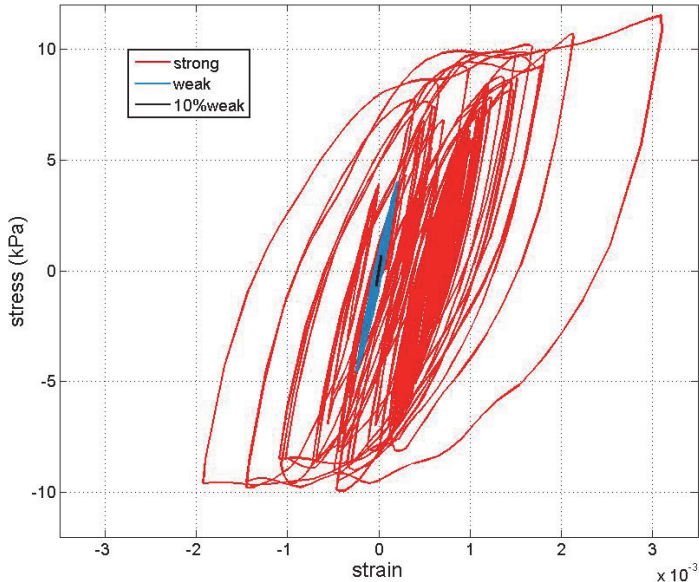
Figure 2.4. Stress Strain Relationship of loose cohesionless soil response computed by CYCLIC 1D at a depth of 1.15m for strong, weak and 10% weak input motions.
