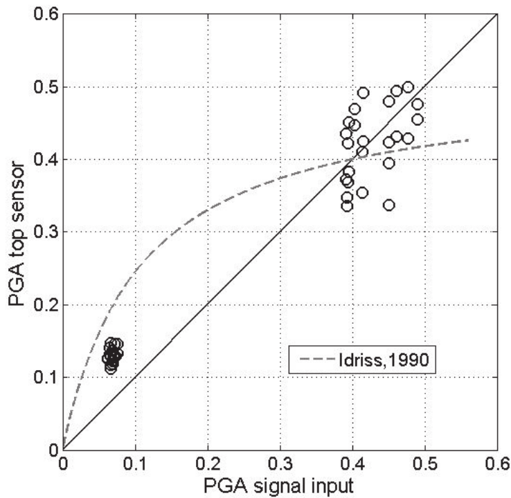
Figure 2.11. Approximate relationship between the PGA of signals recorded by top sensors and the PGA of signals recorded by the sensor located at the bottom of the container. Black circles show the results obtained from centrifuge test with the black dashed line as the approximate relationship, and gray dashed line as the approximate relationship from Idriss (1990).
