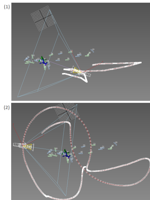
Figure C.2: Camera trajectories in straight walking and ( 180^\circ ) turning behaviors; 1) without keeping the same viewpoint (Synchronized non uniform semi-linear style), 2) while keeping the same viewpoint (Synchronized non uniform non linear style). The screen shot corresponds to the same frame in the animation.
