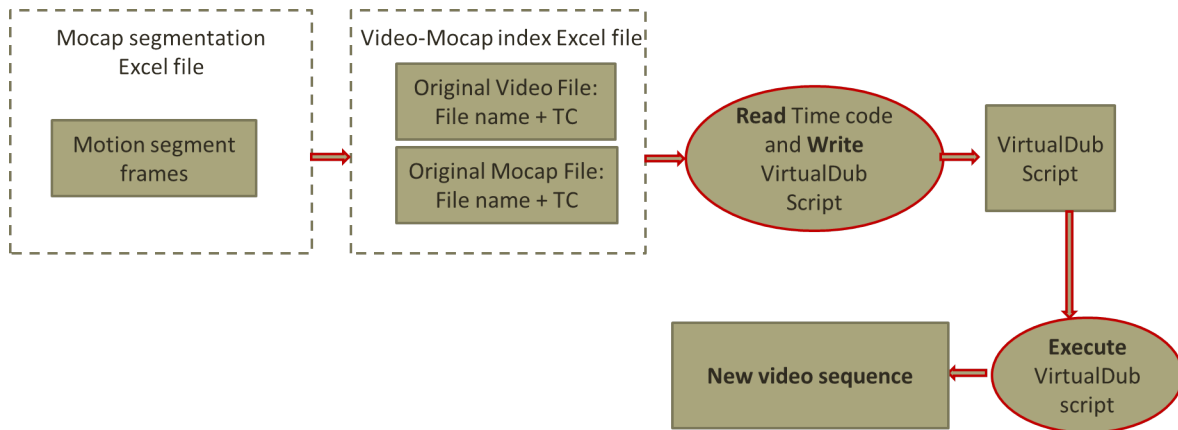
Figure 7.4: Automatic video files segmentation based on TC and motion-capture files segmentation frames
