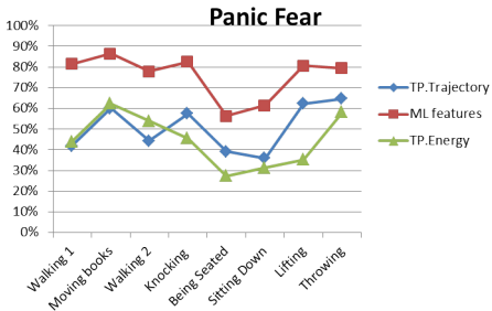
(e) Contribution of Temporal Profile features for Panic Fear classification per action
