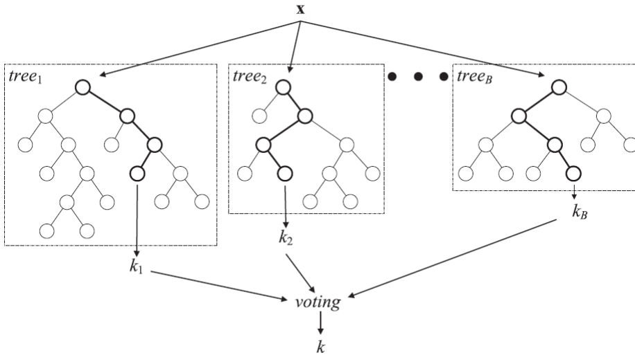
Figure D.1: A general architecture of a Random Forest [Verikas et al., 2011].
