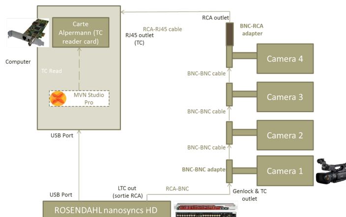
Figure 7.3: Synchronization of video and 3D motion capture data
