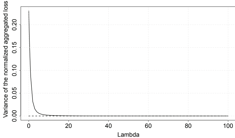
Figure 4.6: The solid line corresponds to the evolution of R_2(\lambda A) with respect to \lambda in the case of the tube model, with R_b = 1 and A being a disk. The dashed line represents the limiting risk measure.
