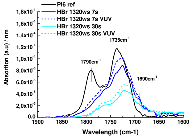
Figure III-22 C=O region FTIR spectra of a photoresist exposed to an HBr cure (Full plasma and VUV) at 1320w during 7s and 30s
