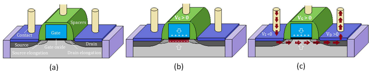
Figure I-1 Schematic representation of n-MOS transistor operating principle. (a) Illustration of the MOS components at V_G=0 , (b) Formation of the conduction channel with a V_G>0 and (c) conduction of electrons at V_D>0 [3].
