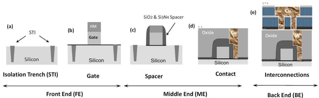
Figure I-5 Five main sections involved in the 14FDSOI integrated circuit manufacturing: (a) STI formation, (b) Gate formation (c) Spacer deposition and implantation of source and drain electrodes, (d) Contact of all Source, drain and gate electrodes by a first W metal layer (To simplify, only the drain contact is shown) and (e) Interconnection of all the transistors by the formation of 9 different metal levels using Copper (Cu) as connection metal.
