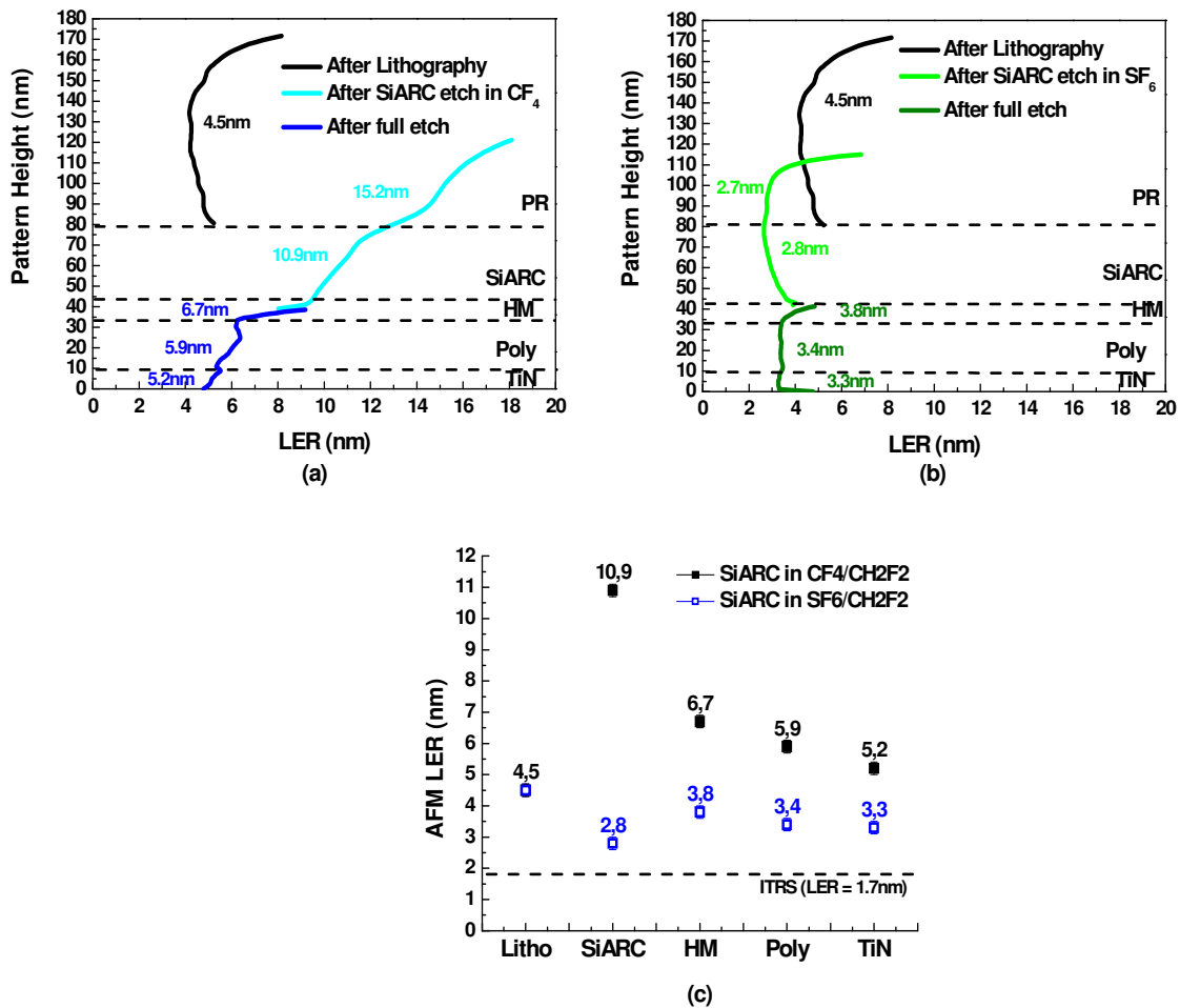
Figure IV-33 Comparison of the LER evolution during gate patterning for the two different gate etch processes: (a) SiARC etch in CF_4/CH_2F_2 and (b) SiARC etch in SF_6/CH_2F_2 . The remaining gate etch process remains the same for both samples. (c) Comparison of LER values obtained in (a) and (b) after each process step is shown.
