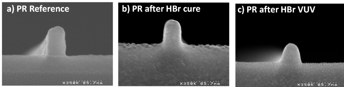
Figure I-24 SEM observation of Resist pattern: (a) after lithography, (b) after HBr plasma treatment, (c) VUV light treatment [17][80]
