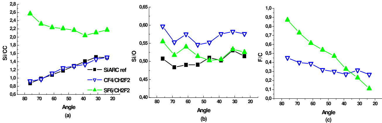
Figure IV-27 (a) Si/CC (measured with equation 3), (b) Si/O and (c) F/C ratios (equation 4) of SiARC samples after exposure to \text{CF}_4/\text{CH}_2\text{F}_2 plasma (at 600V) and \text{SF}_6/\text{CH}_2\text{F}_2 plasma (at 70V) conditions during 10s.
