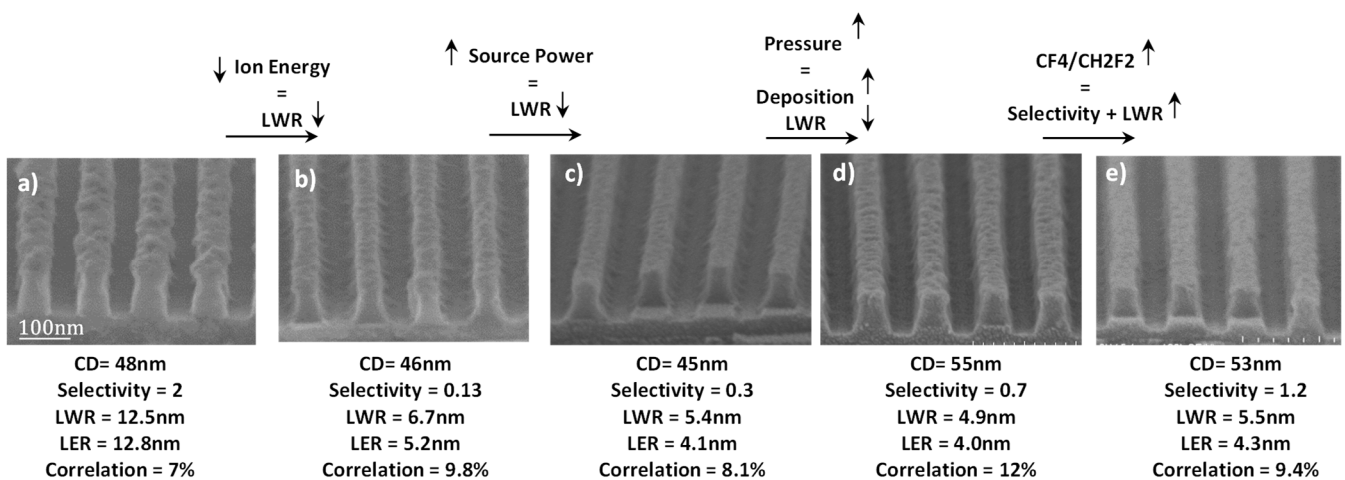
Figure 1 Pattern CD, roughness and correlation evolution with process conditions
