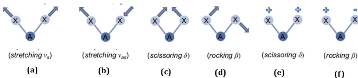
Figure II-10 Elongation and deformation vibration modes of an \text{AX}_2 molecule
