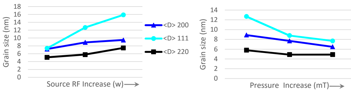
Figure V-15 TiN grain size (<D>) evolution as a function of the applied source power and Pressure for an RF-PVD deposition process
