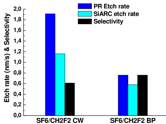
Figure 3 Etch rate and Selectivity of Photoresist and SiARC samples exposed to a SF_6/CH_2F_2 plasma in a CW and BP (200Hz, DC25%)
