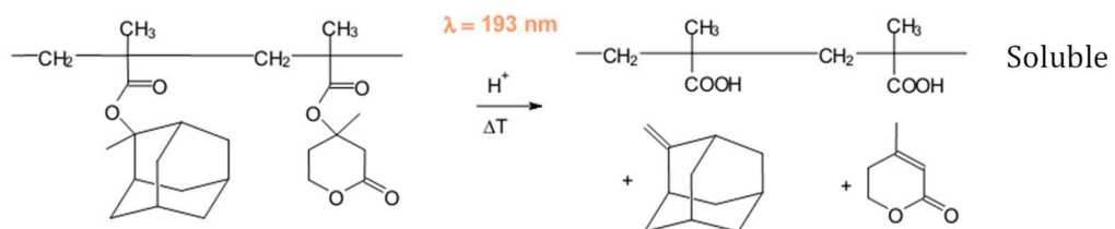
Figure I-9 Example of the deprotection reaction of a AZ/Clariant193nm Photoresist in presence of an acid ( \text{H}^+ ). Ester hydrolysis leads to a detachment of monomers active groups and the formation of a soluble polymer backbone in basic solution [13].
