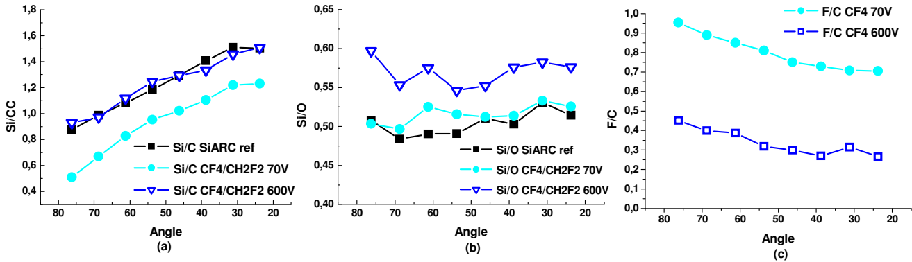
Figure IV-13 (a) Si/CC (b) Si2p/O1s and (c) F1s/C1s ratio evolution with scanning angle for an SiARC layer before and after exposure to a CF_4/CH_2F_2 plasma at 70V and 600V. \theta = 76^\circ refers to extreme surface while \theta = 23^\circ is relative to SiARC bulk. The Si/CC and F/C ratios are calculated following equations 3 and 4
