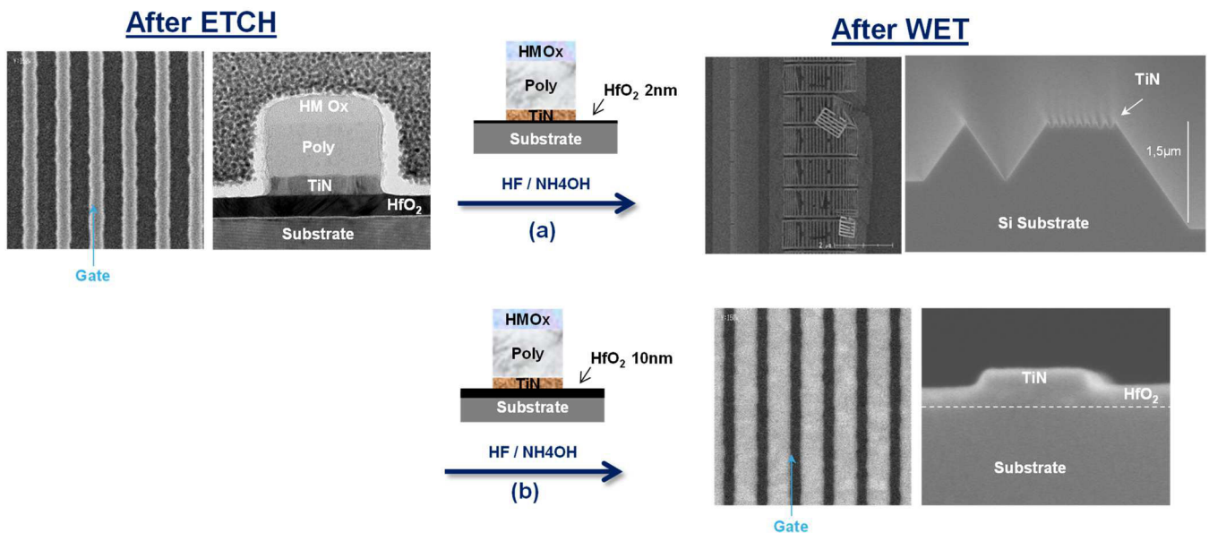
Figure V-2 Gate patterns exposed to the polysilicon wet removal chemistry (HF 1%, NH 4 OH 5%). (a) TiN patterns deposited over thin HfO 2 films (2nm) are removed by lift-off due to HfO 2 etch in HF chemistries and subsequent silicon bulk etch in NH 4 OH. (b) Increasing the HfO 2 thickness to 10nm promotes HfO 2 crystallization and HfO 2 dissolution in HF solutions is avoided.
