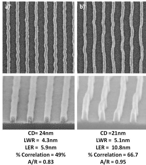
Figure IV-39 Comparison of the Correlation factor and wiggling effect observed over silicon patterns as a function of the gate pattern aspect ratio for two gates etched using the SiARC etch condition in \text{CF}_4/\text{CH}_2\text{F}_2
