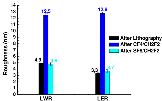
Figure IV-22 Comparison of the SEM roughness values LWR and LER for both SiARC etch conditions, CF 4 /CH 2 F 2 at 600V and SF 6 /CH 2 F 2 at 70V.
