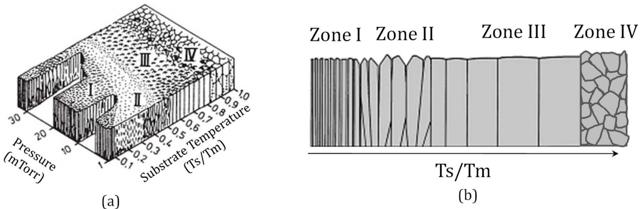
Figure 2. Morphology of PVD deposited films as a function of the working pressure and substrate temperature [1] and a cross section illustration reprinted from Petrov et al [2]
