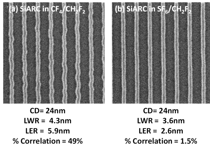
Figure IV-40 SEM top view images of 24nm Silicon gate patterns carried out with SiARC etch chemistries in (a) CF_4/CH_2F_2 and (b) SF_6/CH_2F_2 .
