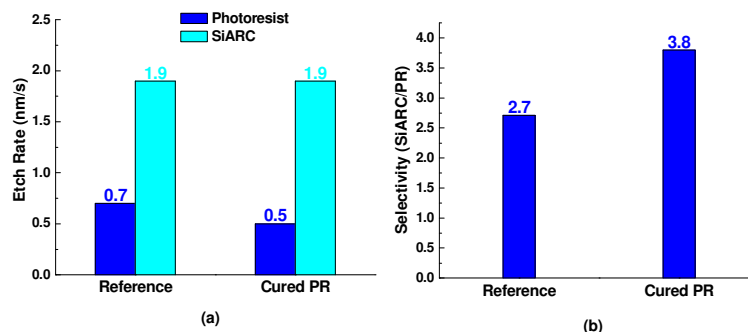
Figure IV-5 (a) Etch rates and (b) selectivity of photoresist (reference and HBr cured) and SiARC layers after exposure to SiARC etch conditions in CF 4 /CH 2 F 2 plasma.
