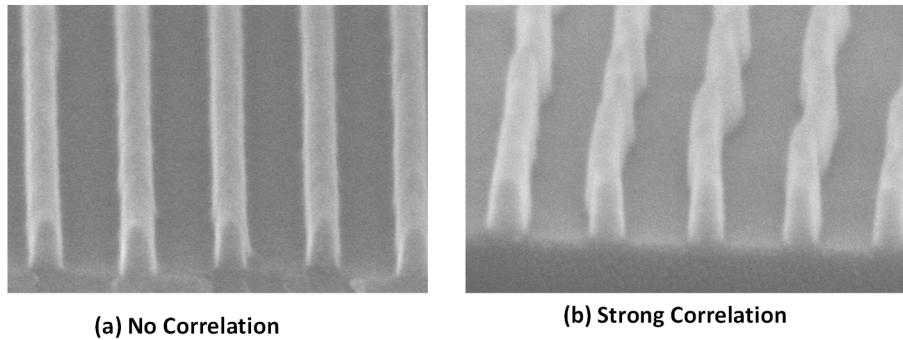
Figure IV-35 SEM Cross-Section images of Silicon gate patterns with (a) No sidewall correlation and (b) Strong sidewall correlation.
