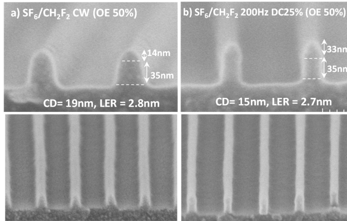
Figure IV-32. SEM Cross-Section images of PR/SiARC stacks exposed to SF 6 /CH 2 F 2 SiARC conditions in a (a) Continuous wave, and (b) Bias pulsing mode.
