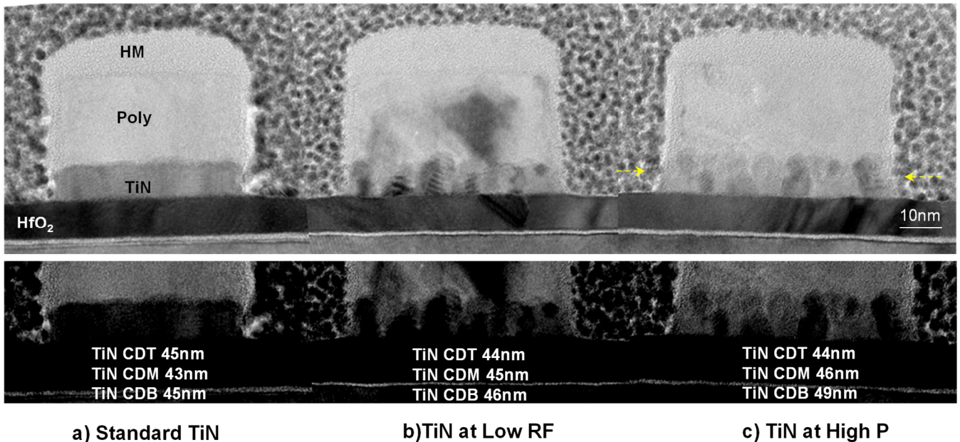
Figure V-19 Full etch TEM images of gate stacks with different TiN layers (Standard TiN, TiN Low RF and TiN High P). Zoomed images of the TiN film with stronger contrast are also shown. For High Pressure TiN films a double TiN layer is observed. Arrows are added to guide the eyes.
