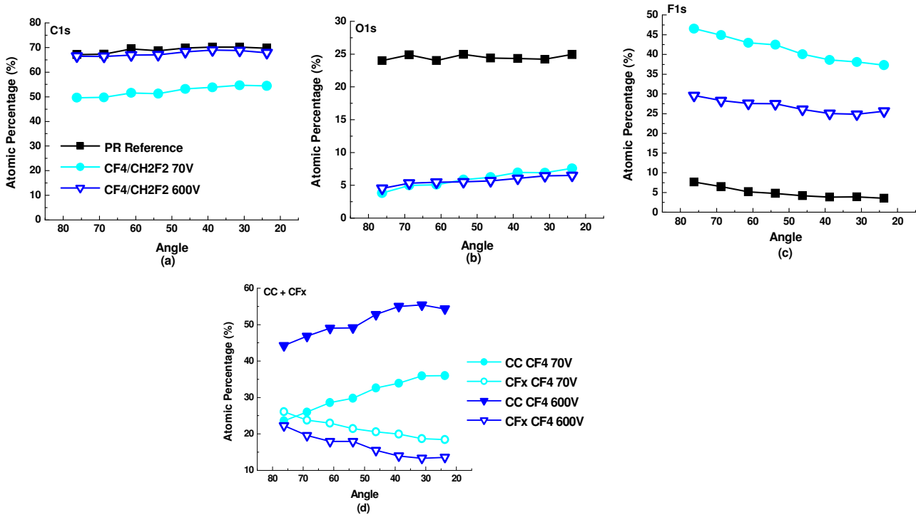
Figure IV-16. Evolution of the elemental composition as a function of the analyzed angle for photoresist before and after exposure to \text{CF}_4/\text{CH}_2\text{F}_2 plasma at 70V and 600V: a) C1s; b) O1s; c) F1; d) CC and CF x contributions. The C-C and C-CF x contributions have been gathered under the label “C-C”, while CF, CF 2 and CF 3 contributions are represented by the label CF x .
