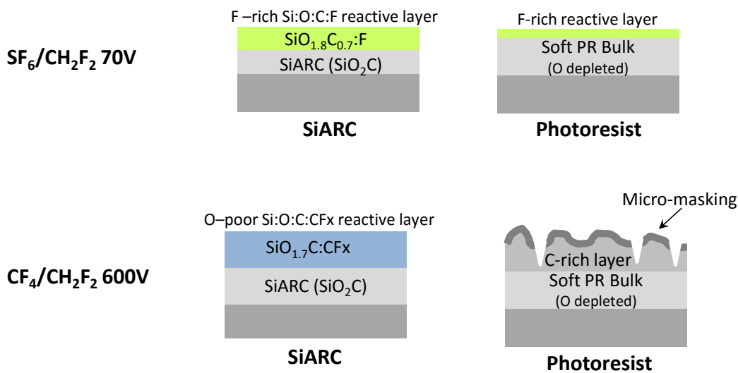
Figure IV-31 Schematic representation of the SiARC and Photoresist etch mechanisms in CF_4/CH_2F_2 and SF_6/CH_2F_2
