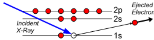
Figure II-14 Photoelectric effect principle
