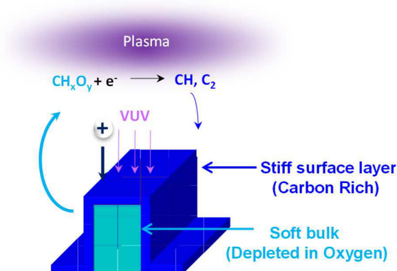
Figure I-23 Schematic illustration of the photoresist cure mechanism
