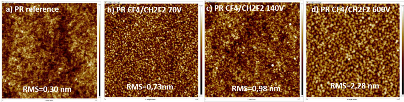
Figure IV-7 AFM images of photoresist layers (a) as deposited and exposed to a \text{CF}_4/\text{CH}_2\text{F}_2 plasmas with (b) 70V (c) 140V and (d) 600V applied bias voltages (std condition).
