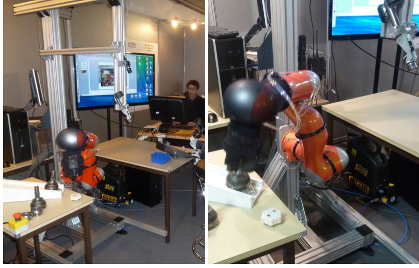
Figure 3.18: The planning setup of the ICARO industrial scenario. Left: a global view of the setup. Right: the start configuration.
