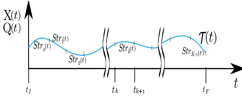
Figure 4.1: A trajectory is composed of K polynomial segments, t_I and t_F are the initial time and final time of the trajectory.
