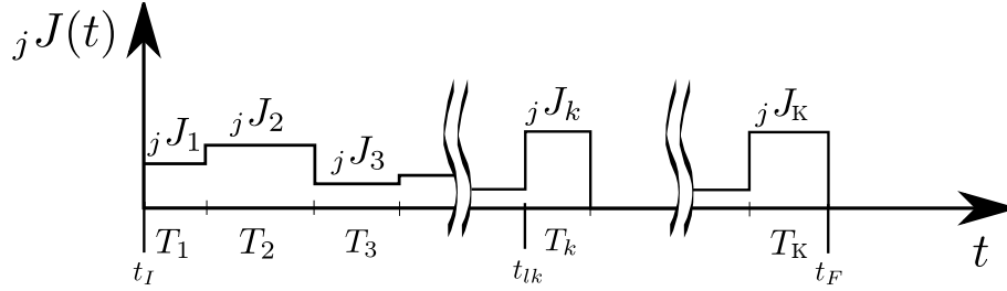
Figure 3.1: The jerk evolution for the j axis of the \mathcal{S}(t) trajectory.
