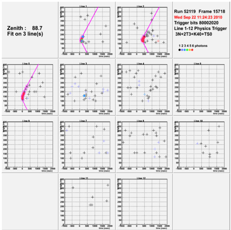
Figure B.4: Alert ANT100922
