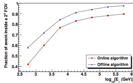
(b) Fraction of events inside a field of view of 2^\circ \times 2^\circ as a function of the energy of the event.
