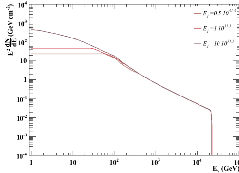
(f) Neutrino spectrum from Pions and Kaons for several jet energies values.
