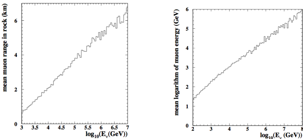
(a) Average range of the muon in standard rock as a function of the initial neutrino energy.
