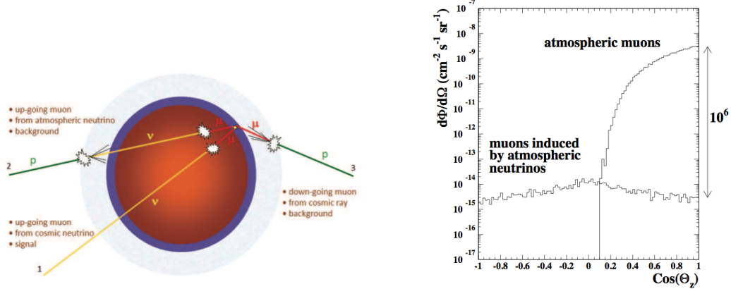
(a) Schematic depiction of signal and background components for a HE neutrino detector. Track 1 is the upward-going signal muon neutrino originating from astrophysical sources. Track 2 is the upward-going muon neutrino originating from the interaction of CRs with the atmosphere. Track 3 is the downward-going atmospheric muon issued from the interaction of CRs in the upper layers of the atmosphere.
