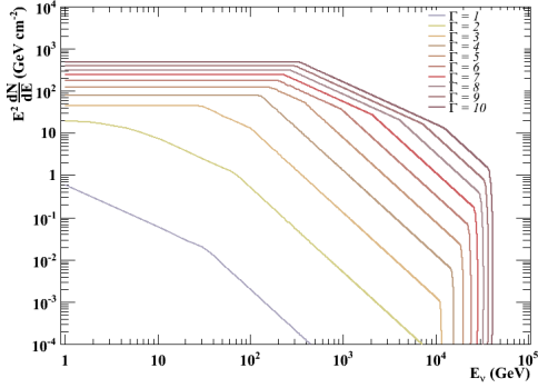
(a) Neutrino spectrum from Pions for several boost factors values.
