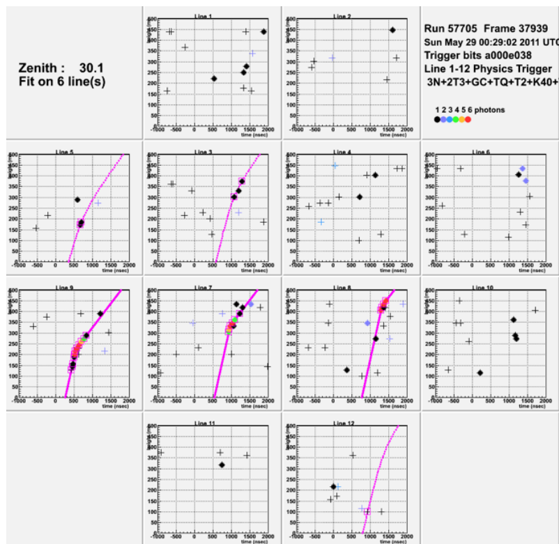
Figure B.7: Alert ANT110529
