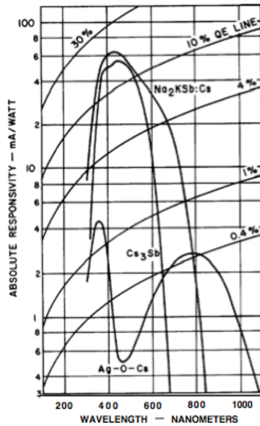
Figure 3.5: Typical spectra-response curves, with 0080 lime-glass window for (a) silver-oxygen-caesium (Ag-O-Cs), (b) caesium-antimony ( \text{Cs}_3\text{Sb} ), (c) multialkali or trialkali ( \text{Na}_2\text{KSb:Cs} )
