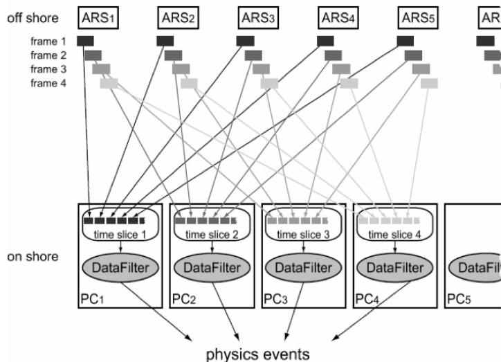
Figure 2.9: Scheme of the data processing based on time slices. All frames belonging to the same time window are sent to a single PC and form a time slice. The DataFilter program running on each PC processes the data in the time slice. All physics events are stored on disk.
