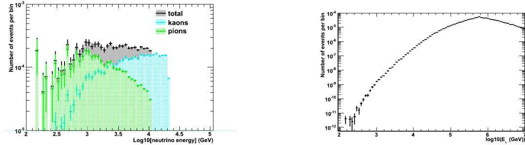
(a) Energy distribution of the expected events from a CCSN at 10 Mpc, with a jet duration of 10s, a jet kinetic energy of 3 \cdot 10^{51} erg and a boost factor of 3 passing the HE filter.
