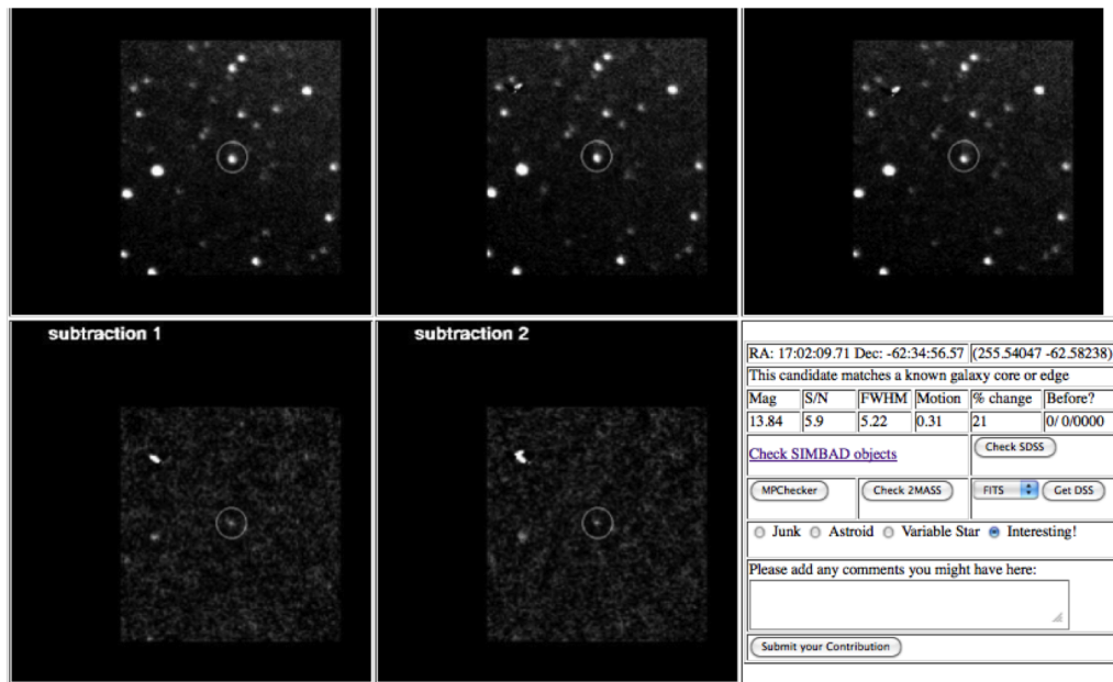
Figure 7.5: A transient candidate from alert ANT100725. The upper left image is NEW1, the upper middle image is NEW2 and the upper right image is REF. The bottom left image is (NEW1 -REF) and the bottom right image is (NEW2 - REF).
