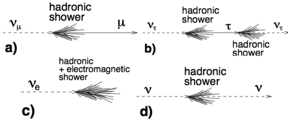
Figure 1.13: Signatures of the event topologies occurring for different types of neutrino interactions [60]. a) Charged current interaction of a \nu_\mu produces a muon and a hadronic shower; b) Charged current interaction of a \nu_\tau produces a \tau that decays into a \nu_\tau , tracing the double bang event signature. c) Charged current interaction of \nu_e produces both an electromagnetic and a hadronic shower; d) a neutral current interaction produces a hadronic shower.
