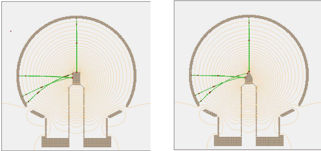
(a) Equipotentials (yellow) and electron trajectories (green) in a spheric shape device with a cylindric anode. Red dots mark the position of the electrons at each nano-second.
