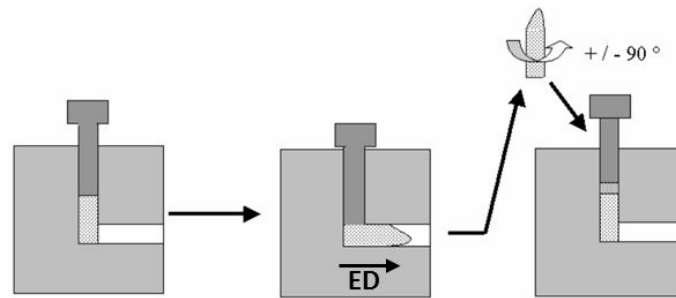
Figure 36: Specific introduction of the billet for each pass [141] and description of the extrusion direction (ED).
