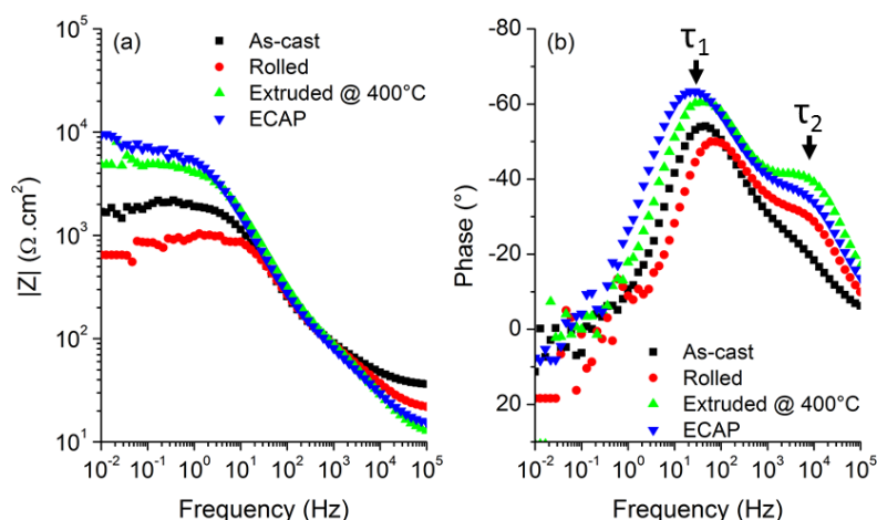
Figure 41: Bode plots of the as-cast and the thermomechanically processed samples at the initial state.
