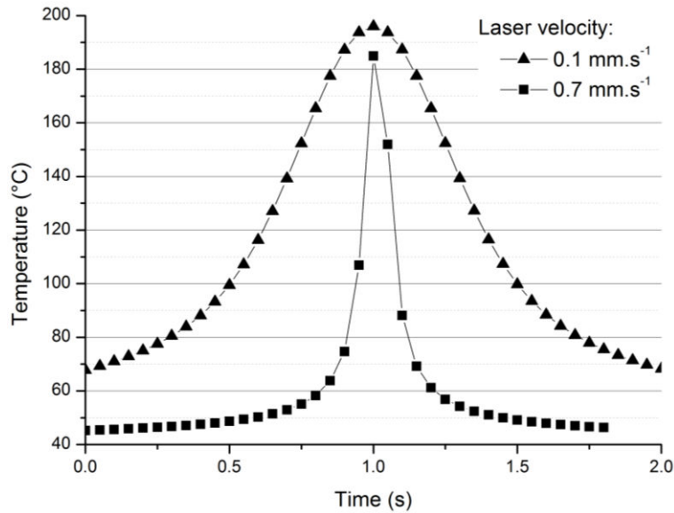
Figure 90: Temperature profile during sintering of a point on the top surface of the silver deposition with ( \beta_S = 0.23; \beta_D = 0.23 ) and for different velocities: 0.1 \text{ mm.s}^{-1} and 0.7 \text{ mm.s}^{-1} .
