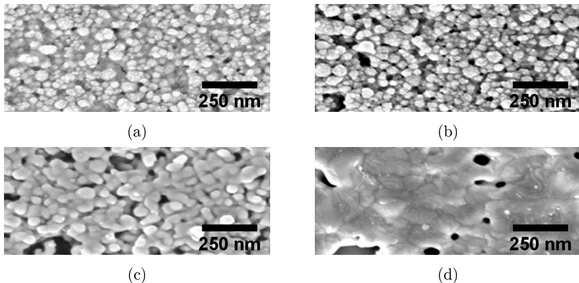
Figure 66: SEM images of an ink containing nanoparticle mixture of copper deposited by spin-coating on a glass substrate: (a) un-sintered, (b) organics partly removed, (c) nanoparticles necking takes place and (d) grain growth, i.e. extensive sintering – Images adapted from [183].
