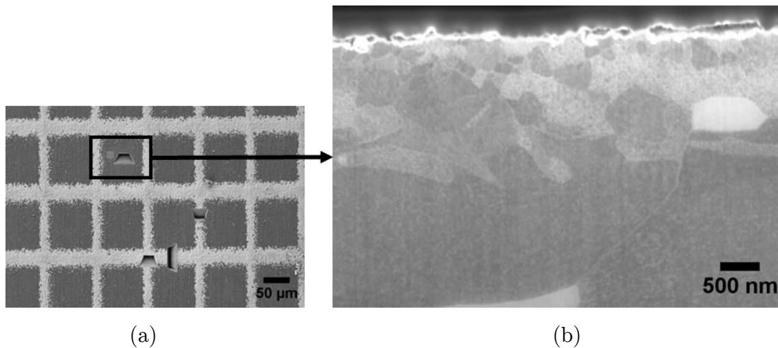
Figure 81: (a) Location of the FIB cross sections and (b) SEM image of a cross section of a laser treated sample extruded at 400 \text{ }^\circ\text{C} obtained using a laser beam with 8 W power, 85 \mu\text{m} spot size and 0.1 \text{ mm}\cdot\text{s}^{-1} beam velocity.
