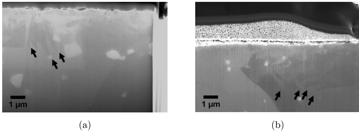
Figure 83: SEM image of a cross section of a laser treated sample extruded at 400 °C with 8 W power, 85 \mu\text{m} spot size and 0.1 \text{mm}\cdot\text{s}^{-1} laser beam velocity; twins pointed by arrows.
