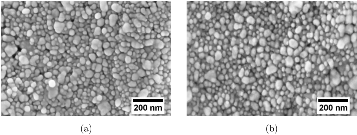
Figure 75: SEM images of deposited lines of silver nanoparticles after laser sintering with 8 W power and different velocity: (a) 0.1 \text{ mm.s}^{-1} and (b) 0.7 \text{ mm.s}^{-1} .
