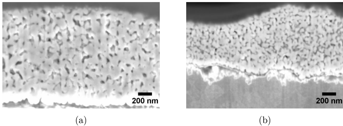
Figure 77: SEM micrographs of a cross section of sintered deposition of silver nanoparticles with 8 W power, 85 \mu\text{m} spot size and (a) 0.1 \text{ mm}\cdot\text{s}^{-1} , (b) 0.7 \text{ mm}\cdot\text{s}^{-1} .
