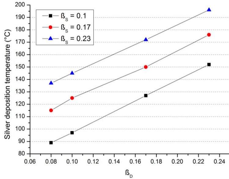
Figure 88: Maximum temperature in a silver deposition as function of the sets of absorbance coefficients ( \beta_S, \beta_D ) and with a laser beam velocity of 0.1 \text{ mm}\cdot\text{s}^{-1} .
