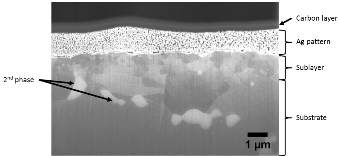
Figure 80: SEM image of a cross section of a sintered surface deposition obtained using a laser beam with 8 W power, 85 \mu\text{m} spot size and 0.1 \text{ mm}\cdot\text{s}^{-1} beam velocity.
