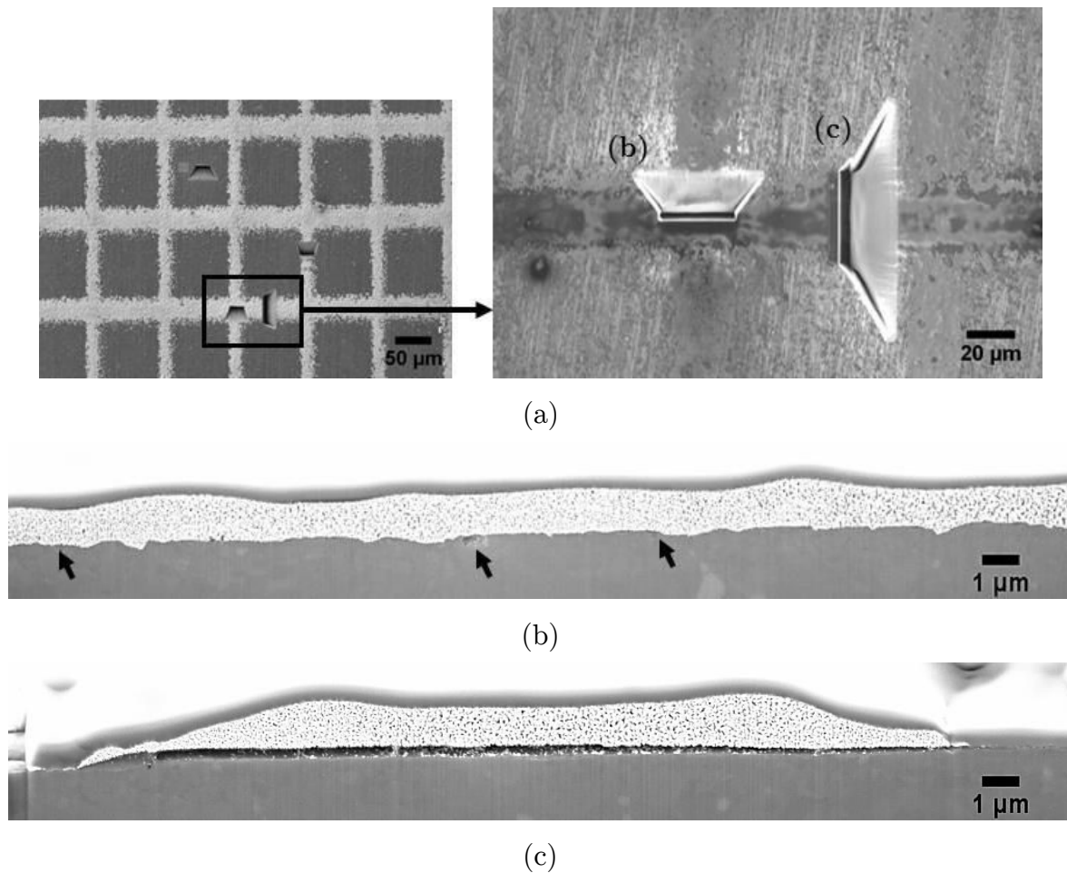
Figure 78: (a) SEM image of the location of FIB sections and the associated cross sections of sintered deposition of silver nanoparticles with 8 W power, 85 \mu\text{m} spot size and 0.1 \text{ mm}\cdot\text{s}^{-1} : (b) intersection of 2 lines and (c) transverse direction to a deposited.
