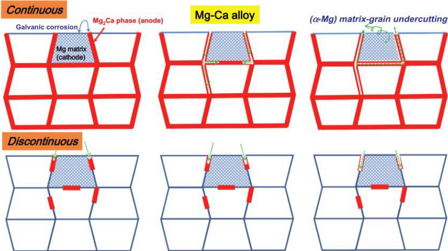
Figure 56: Schematic illustration of the morphologic impact of Mg_2Ca phases in Mg-Ca alloys [33].
