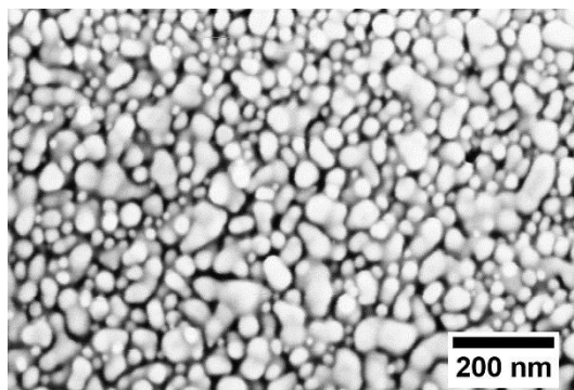
Figure 72: SEM micrograph of silver nanoparticles deposition after laser sintering with 8 W power, 0.3 \text{ mm}\cdot\text{s}^{-1} laser velocity and 85 \text{ }\mu\text{m} laser beam spot size.
