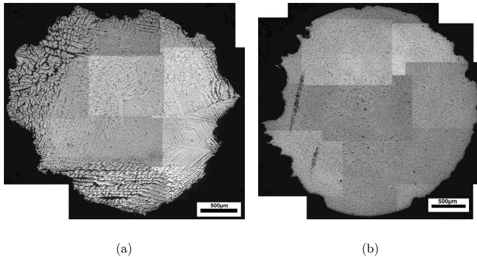
Figure 57: Optical observation of the cross sections of the corroded samples after 7 days of immersion in Hanks solution: (a) as-cast and (b) extruded at 400 °C. Note that the interdendritic zones appearing with a black contrast are empty.
