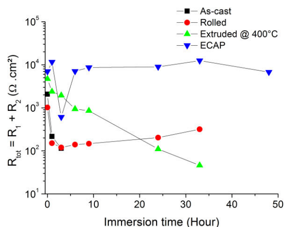
Figure 43: Evolution of the total resistance, R_{tot} , with immersion time in Hanks solution of the as-cast and thermomechanically processed materials.
