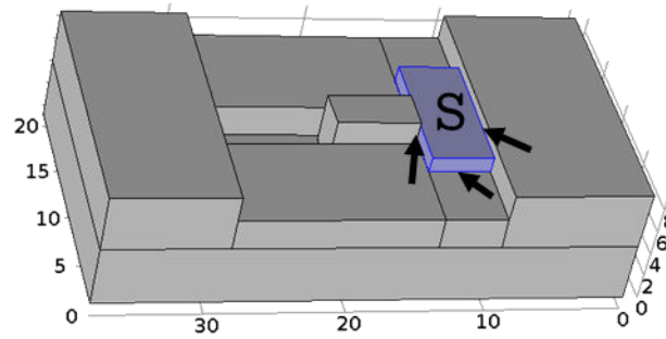
Figure 86: Sample (S) mounted on the holder: surfaces with thermal contact are pointed by black arrows.
