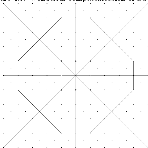
Figure 4.3: Wonderful compactification of SO_5(\mathbb{C})
