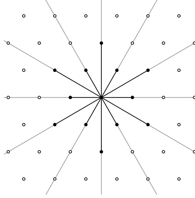
Figure 3.3: Root system G_2
