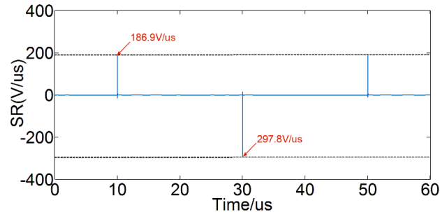
Fig.6.54 Simulated slew rate of the designed OTA.
