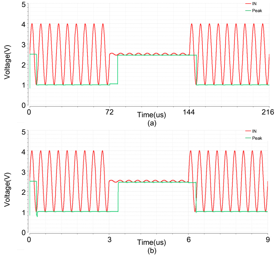
Fig.6.55 Post-layout simulation results of the proposed peak detector with different input signals ( \text{Max}(V_{p-p})=3 \text{ V} , \text{Min}(V_{p-p})=0.1 \text{ V} ): (a) f=125 \text{ kHz} . (b) f=3 \text{ MHz} .
