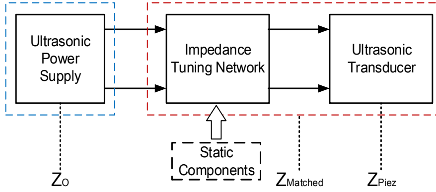
Fig.2.10 Simplified diagram of the static impedance tuning network ultrasonic transducer.
