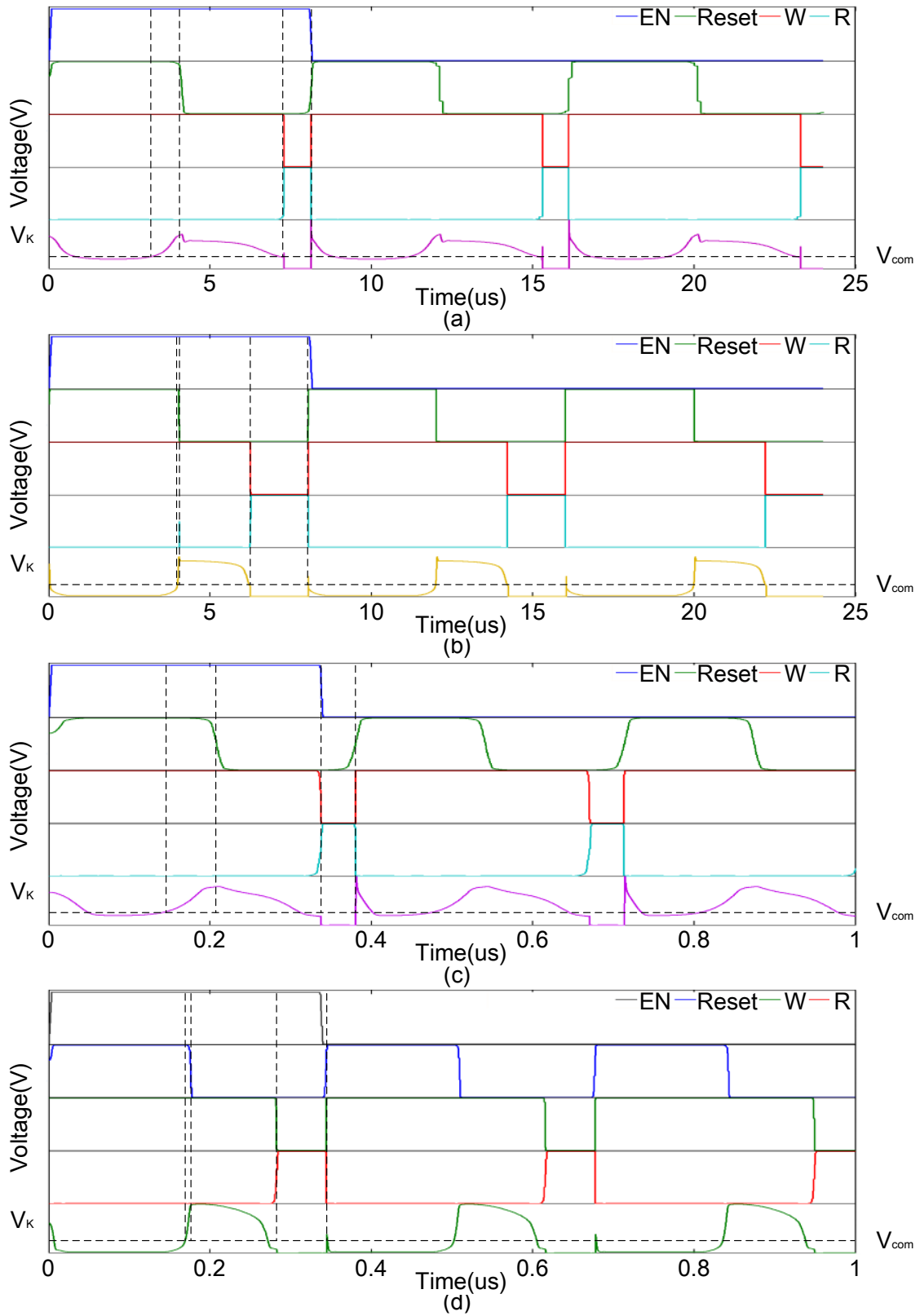
Fig.6.39 Simulation results of the switch control signal generator with different input signals: (a)
