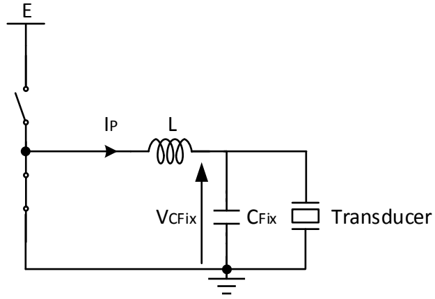
Fig.3.24 Equivalent circuit of the amplifier during the second cycle ( \pi/\omega \leq t < 2\pi/\omega ).
