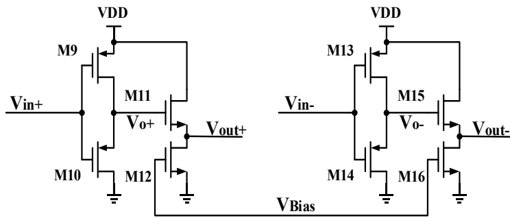
Fig.6.4 Schematic of the attenuation block.
