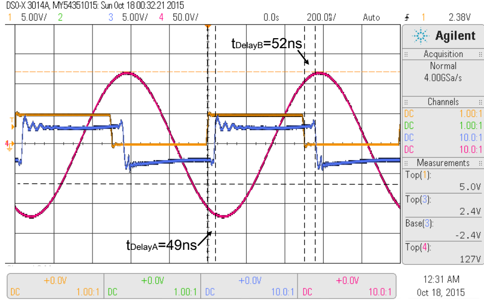
Fig.3.33 Chronograms of the half-bridge output signal V_{HB} and the output of the power amplifier with a 1.25 MHz, 5V input signal.
