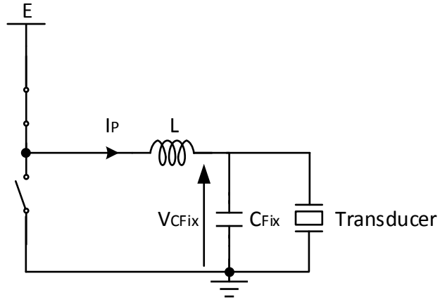
Fig.3.23 Equivalent circuit of the amplifier during the first operating cycle ( 0 \leq t < \pi/\omega ).
