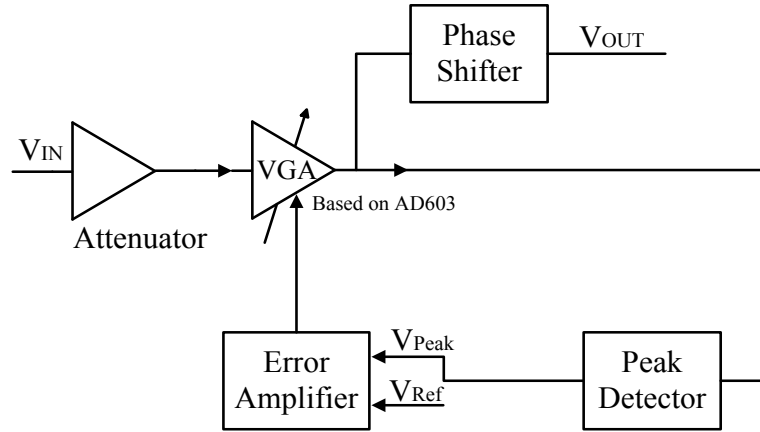
Fig.5.3 Diagram of the proposed automatic gain congrol amplifier.
