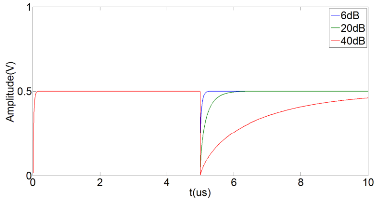
Fig.5.6 Time response of linear AGC for diffrent stepwise functions.
