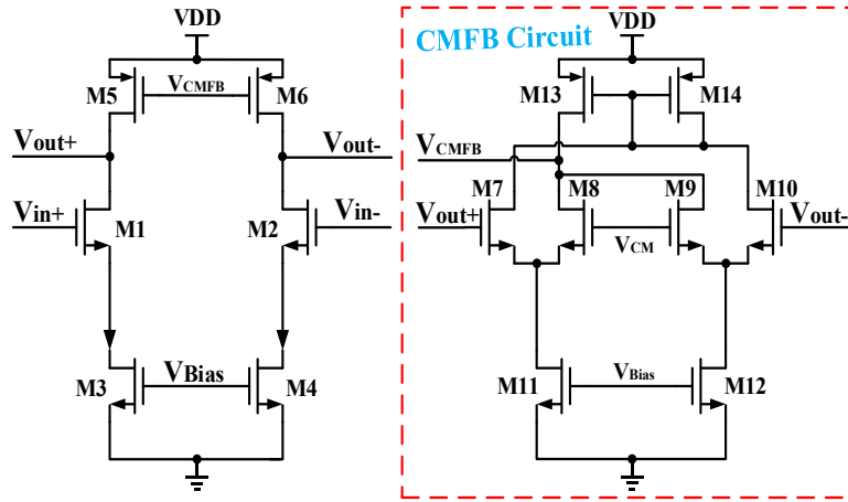
Fig.6.7 Schematic of the differential-transconductance amplifier used in the DC-offset cancellation circuit.
