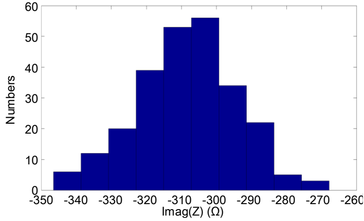
Fig.4.5 Histogram of the measured imaginary impedances.
