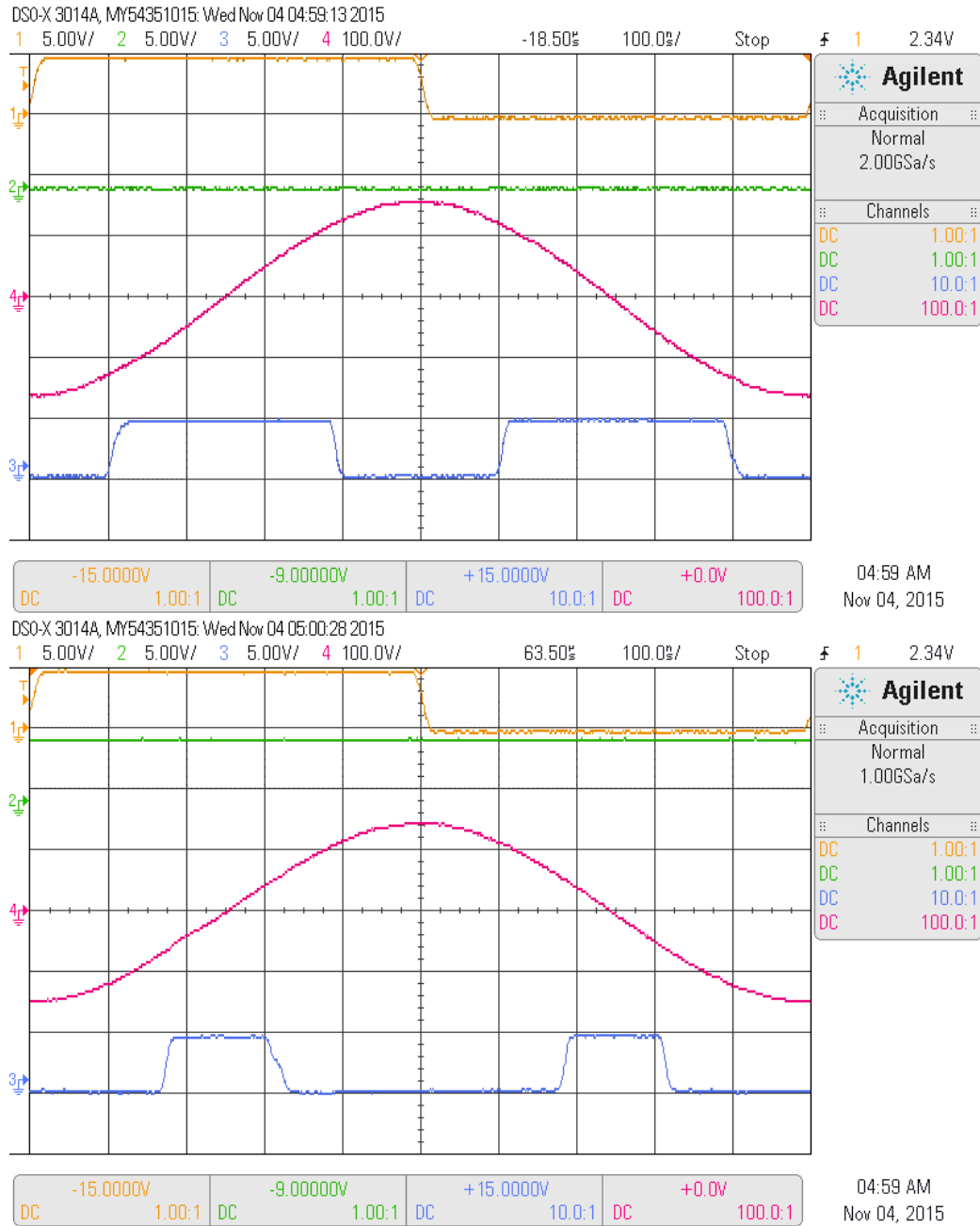
Fig.7.3 Zoomed views of the simulation results of ultrasonic generator with the proposed printed circuit board auto-tuning circuit.
