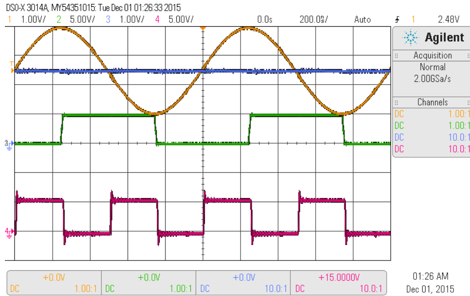
Fig.5.40 Test results of the phase-error detector.
