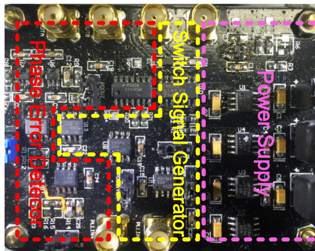
Fig.5.38 Prototype of the phase-error detector combined with switch signal generator.
