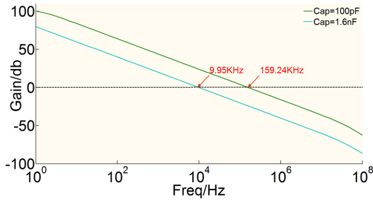
Fig.6.40 Frequency responses of the error amplifier designed for the AGC.
