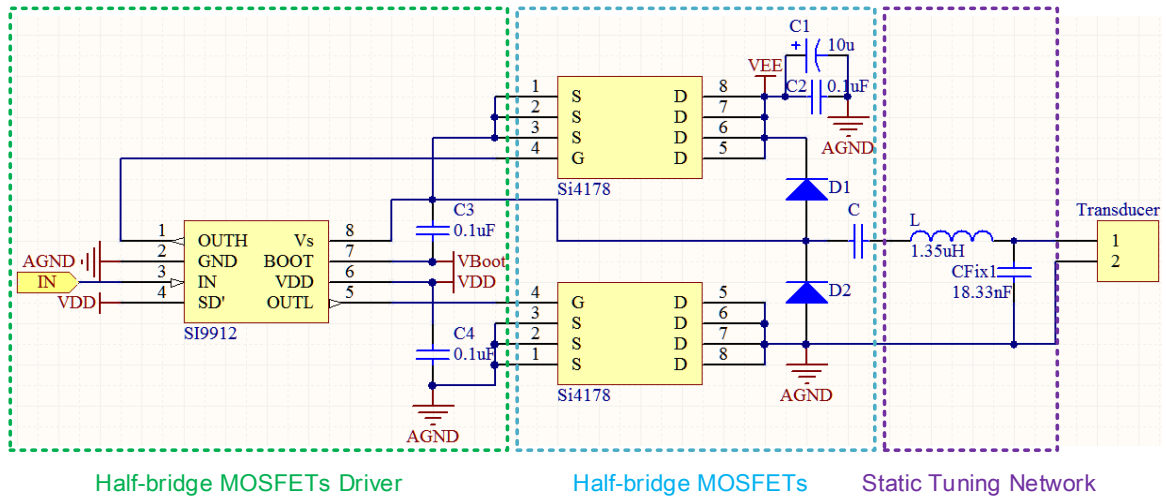
Fig.3.29 Schematic of the proposed class D power amplifier with a static L-type tuning network.
