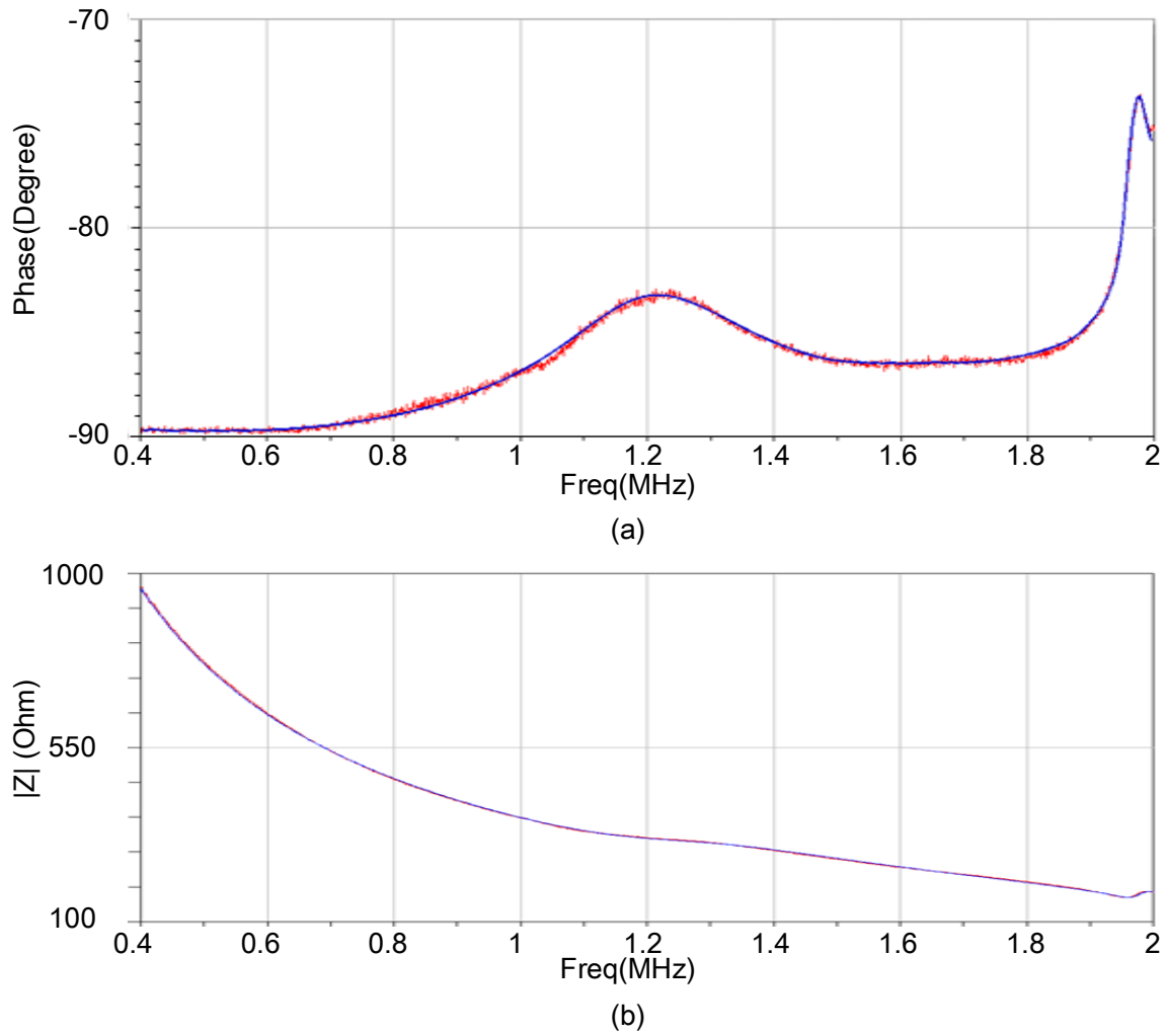
Fig.2.9 (a) Phase curves of the measured impedance (Red) and the equivalent impedance (Blue).
