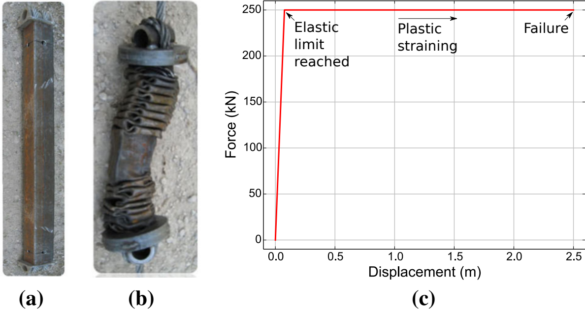
Figure 4.3: Energy dissipators: (a) Before the impact, (b) At the end of the impact (after Bertrand et al., 2012 ), (c) The force:displacement response of the energy dissipators considered in our DEM model
