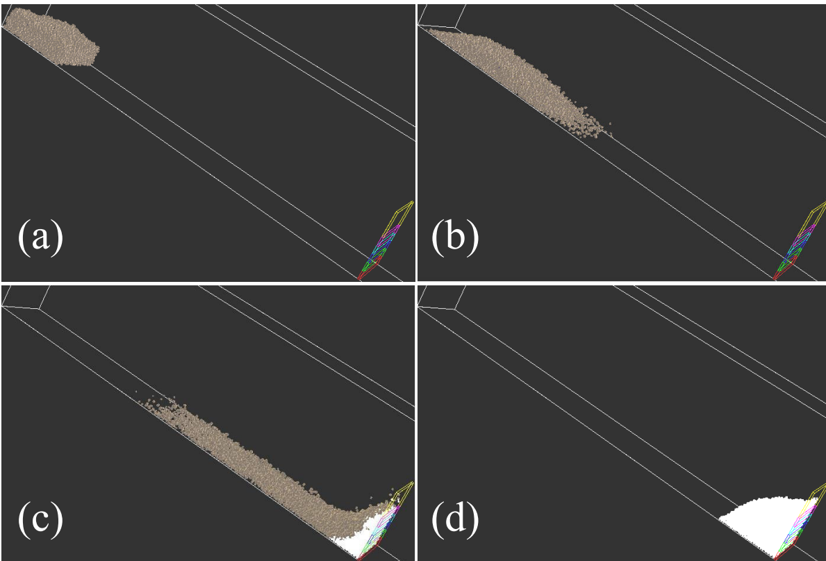
Figure 3.15: Snapshots of the 3D view of the evolution of the calibrated flow through time (test L44-H15- \alpha 40°), along with the evolution of dead particles (colored in white): (a) at time = 2300 ms, (b) at time = 2793 ms, (c) at time = 3583, (d) at time = 4400 ms
