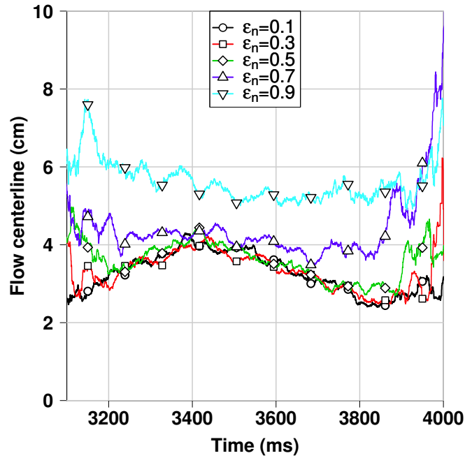
Figure 3.10: Variation of average flow thickness (flow centerline) with time using different normal restitution coefficient values (test L44-H15- \alpha 40°)
