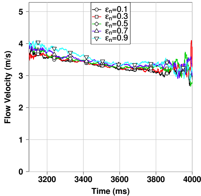
Figure 3.12: Variation of average particles velocity with time, for particles in the upper half of the flow (test L44-H15- \alpha 40°)
