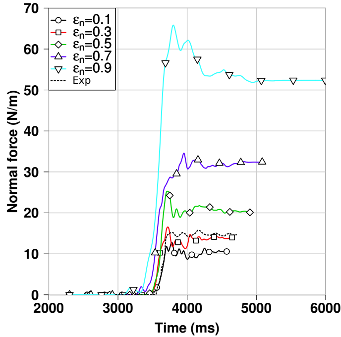
Figure 3.11: Variation of normal force on the sixth segment of the wall with time using different normal restitution coefficient values (test L44-H15- \alpha 40°)
