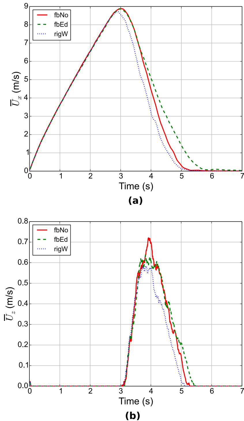
Figure 5.6: Average flow velocity component for three structures: a flexible barrier without energy dissipators (fbNo) and a flexible barrier with energy dissipators (fbEd) and a rigid wall (rigW): (a) in the direction of the flow, (b) perpendicular to the channel base
