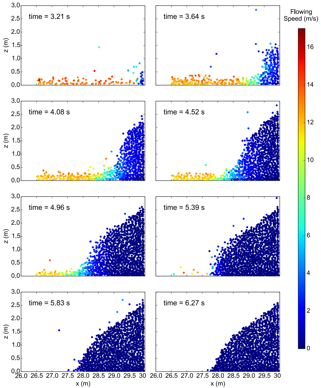
Figure 5.5: Snapshots at given times of the velocity map of particles that lie in the middle of the channel
