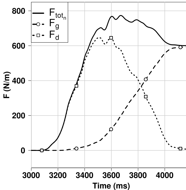
Figure 3.25: Variation of total normal force components with time (test L44-H15- \alpha 40^\circ )
