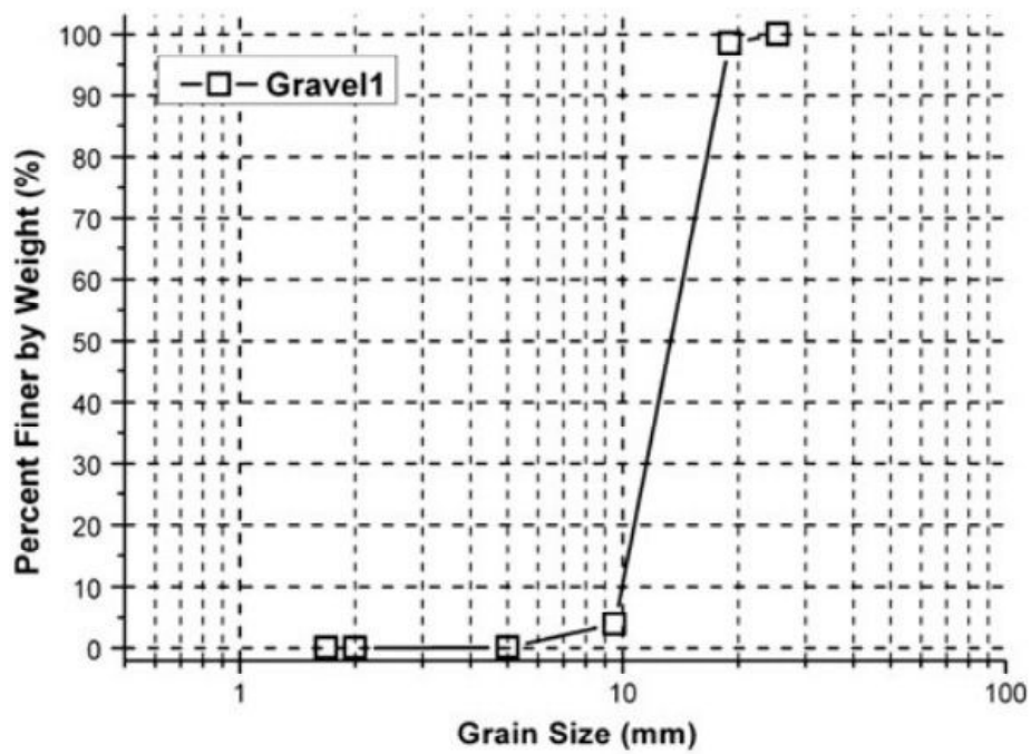
Figure 3.1: (a) Shape of gravel particles, (b) Grain size distribution of the particles (after Jiang and Towhata, 2013)
