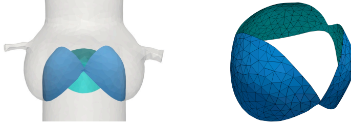
Figure 3.5: Position in the sinus of the aortic root and mesh of the aortic valve in the open configuration.
