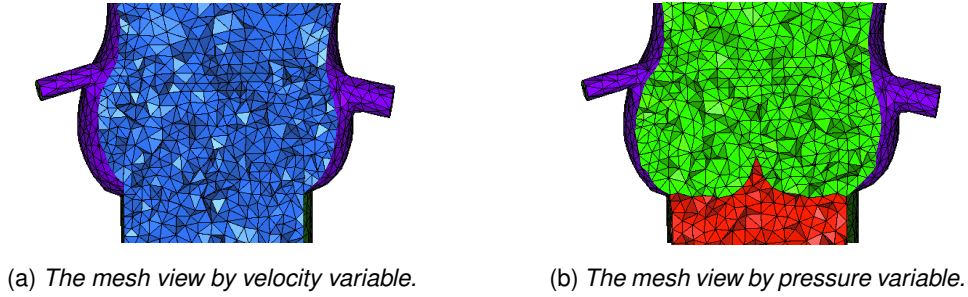
Figure 4.4: Fissured computational domain.
