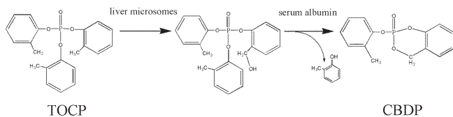
Scheme 1. Metabolic Activation of TOCP to CBDP
