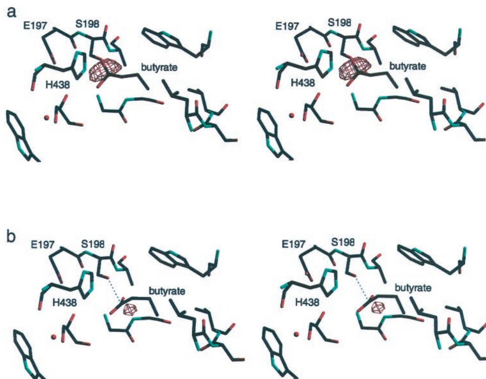
FIG. 3. Difference Fourier electron density maps for bonded and non-bonded butyrate. a , tetrahedral model. Despite the restraints applied the C–O distance is 1.47 Å, and there is a residual negative electron density peak at -5.7\sigma between these two atoms. The average B -factor for the butyrate moiety is 44\text{ \AA}^2 and that of the tetrahedral C atom is 51.1\text{ \AA}^2 (comparable values for the model with a 2.16-Å-long C–O bond depicted in Fig. 2 are 41.7 and 41.4 Å, respectively). b , non-bonded butyrate model. The C–O distance refines to 2.6 Å, and there is a negative peak at -3.7\sigma below the carboxylate carbon atom. The average B -factor for the butyrate moiety is 41.7\text{ \AA}^2 and that of the carboxylate carbon atom is 45.8\text{ \AA}^2 .
