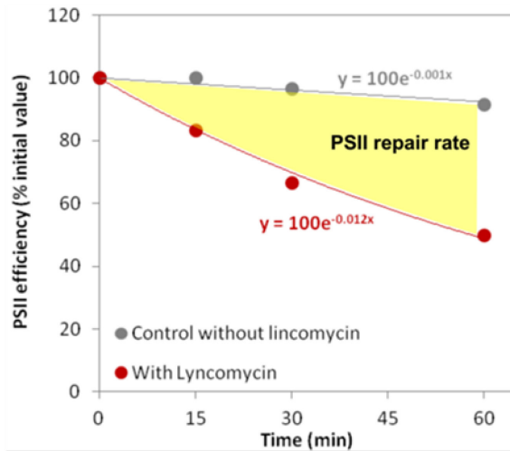
Figure 69 | Calculation of photosystem II repair rate. The photosystem II repair rate is calculated as the difference of photosystem II efficiency between cultures with active photosystem II repair and cultures with inhibited PSII repair (lincomycin treated).
