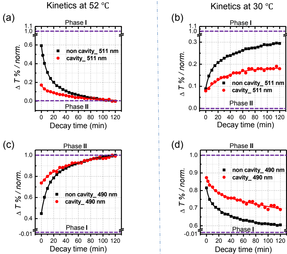
Figure 7.6: Kinetics of the evolution between phase I and II (indicated by violet dashed line) at 52 °C (a) and (c) in the warming cycle and at 30°C (b) and (d) in the cooling cycle, monitored by transmission intensity change at 490 nm for (c) and (d) and at 511 nm for (a) and (b). Figure is from reference. [157]
