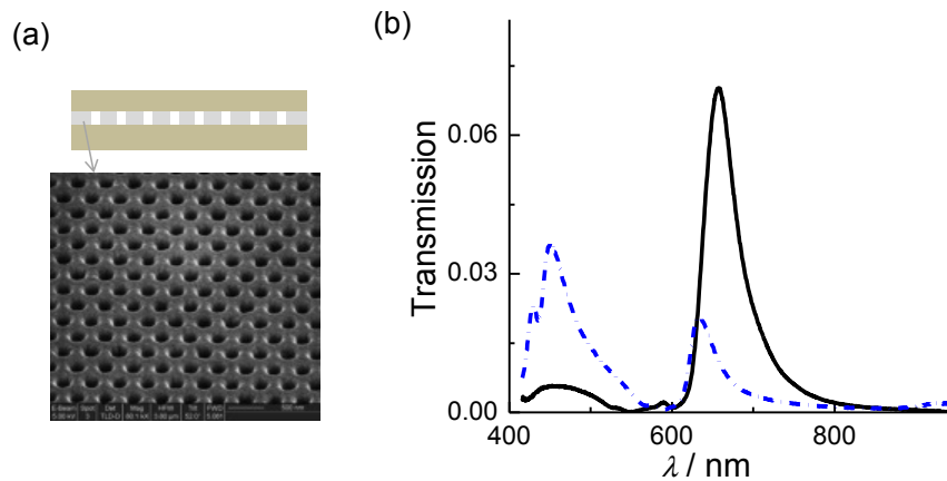
Figure 4.8: (a) The hexagonal hole array shown in the SEM image with period P = 420 \text{ nm} and diameter D = 150 \text{ nm} is milled in 250 nm thick silver film. The schematic picture shows the symmetric structure, in which the hole array is bonded with a 2 mm thick piece of PDMS. (b) Normal incidence transmission spectra of the hole array shown in (a) without (blue dashed curve) and with (black curve) bonding to the PDMS.
