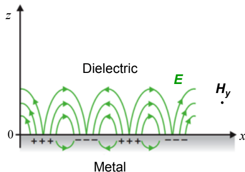
Figure 4.1: Electric field ( E ) and surface charge distributions associated with surface plasmon propagation a metal-dielectric interface.
