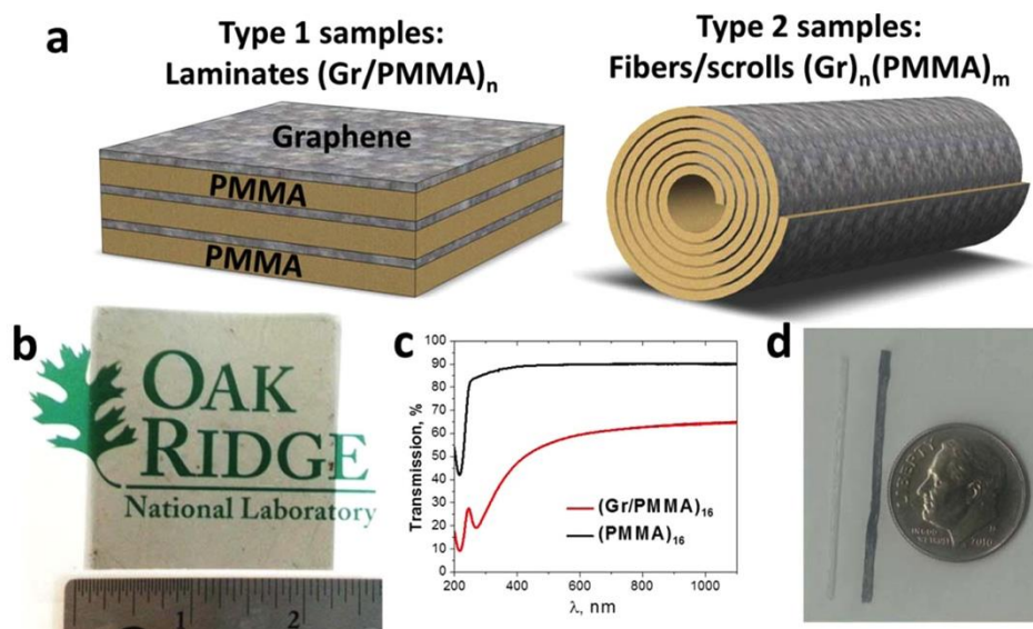
Figure 2.9. a) Scheme of laminates and fibers/scrolls. b) (Gr/PMMA) 16 laminate. c) UV/ vis spectra of (Gr/PMMA) 16 and (PMMA) 16 laminates. d) Photograph of (PMMA) 1 fiber (left) and (Gr) 6 /(PMMA) 1 fiber (right). 93
