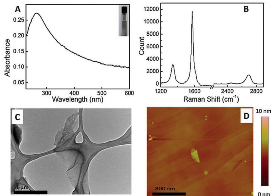
Figure 3.3. a) UV-Vis spectrum of exfoliated graphene in a NaOH solution (pH = 11). Inset: photographic image of the exfoliated graphene, b) Raman spectrum of exfoliated graphene, c) TEM micrograph of a graphene flake and d) AFM image of a graphene flake on an HOPG substrate. 10
