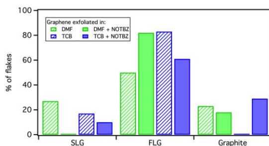
Figure 9.7. Statistical analysis, based on Raman spectroscopy, on the thickness distribution of the flakes in DMF and TCB before and after adding NOTBZ.
