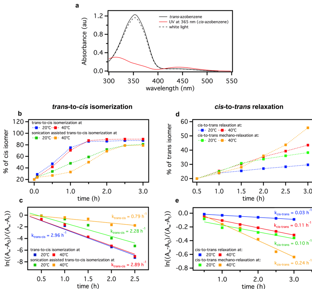
Figure 10.5. Spectroscopic characterization of trans -to- cis isomerization and cis -to- trans relaxation. a) UV-vis spectra of 4-(decyloxy)azobenzene in NMP (1.62 mM) showing the disappearance of the 353 nm band and an increase of the 442 nm band upon irradiation with UV-light ( \lambda = 365 nm). The solid black line corresponds to the parent trans -azobenzene spectrum, the red line represents typical spectrum of solution irradiated with UV-light ( cis -azobenzene), the black dashed line – cis -azobenzene irradiated with visible light (thus re-transformed in trans -azobenzene), b) Difference in percentage of conversion from trans to cis isomer as a function of UV irradiation time at 20 and 40 °C, c) First-order kinetic plots and rate constants ( k_{trans-cis} ) for the trans -to- cis isomerization of at 20 and 40 °C, d) Difference in percentage of conversion from cis to trans isomer as a function of time at 20 and 40 °C, e) First-order kinetic plots and rate constants ( k_{cis-trans} ) for cis -to- trans relaxation of at 20 and 40 °C. b-e) Blank samples, i.e. samples prepared without sonication: blue (20 °C) and red (40 °C); sonicated samples: green (20 °C) orange (40 °C).
