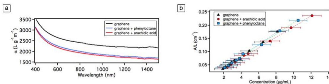
Figure 6.6. a) Absorption spectra for graphene flakes dispersed in NMP, in the presence and absence of dispersion-stabilizing compounds; b) Optical absorbance (at \lambda = 660 nm) divided by cell length ( A/l ) as a function of concentration for graphene in the three samples, showing Lambert – Beer behavior. The x-axis error bars are due to the uncertainty in measuring the mass of graphene/graphite in solution.
