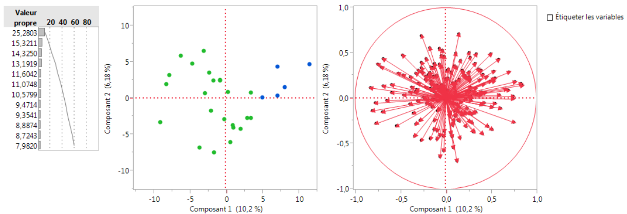
Figure 5: PCA of samples composition of uncontaminated half core. Surface samples (green dot), 6cm depth samples (blue dot).
