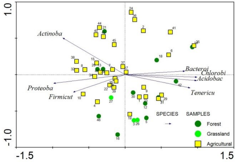
Figure 4: Principal component analysis of the microbial taxonomy at the phylum level based on phylogenetic microarray results
