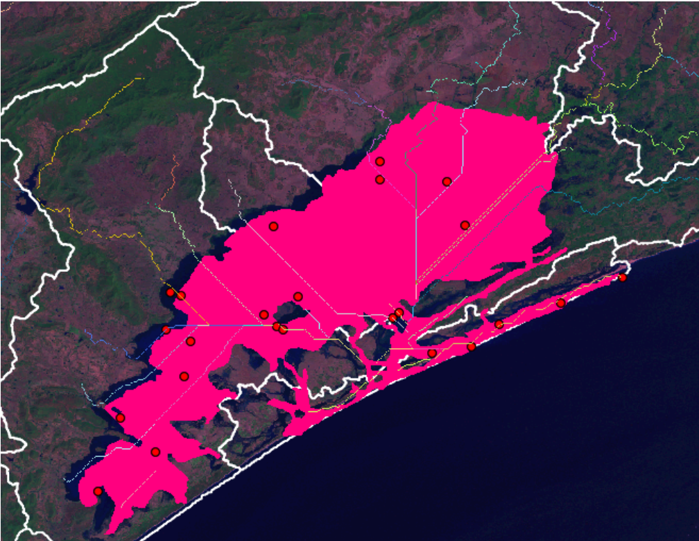
Large Watershed
