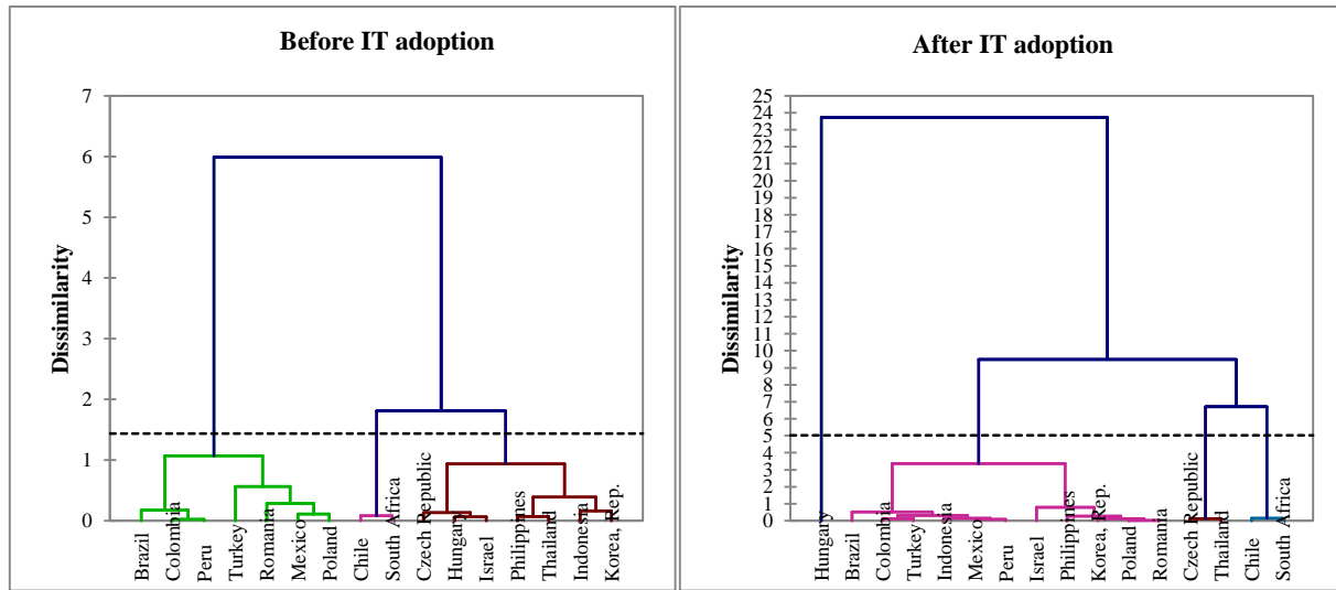
Clustering analysis for emerging market inflation targeters, based on macroeconomic conditions (Ward's agglomerative algorithm). The dotted lines allow determining the optimal number of cluster.
