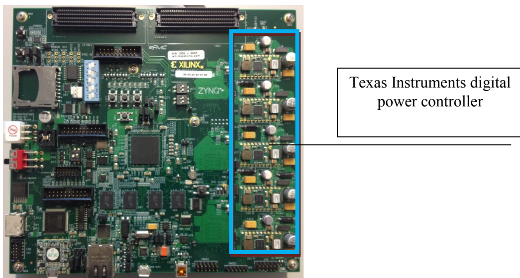
Figure 3.5-Integrated Texas Instruments digital power controller on Zynq-7000 Ap SoC
