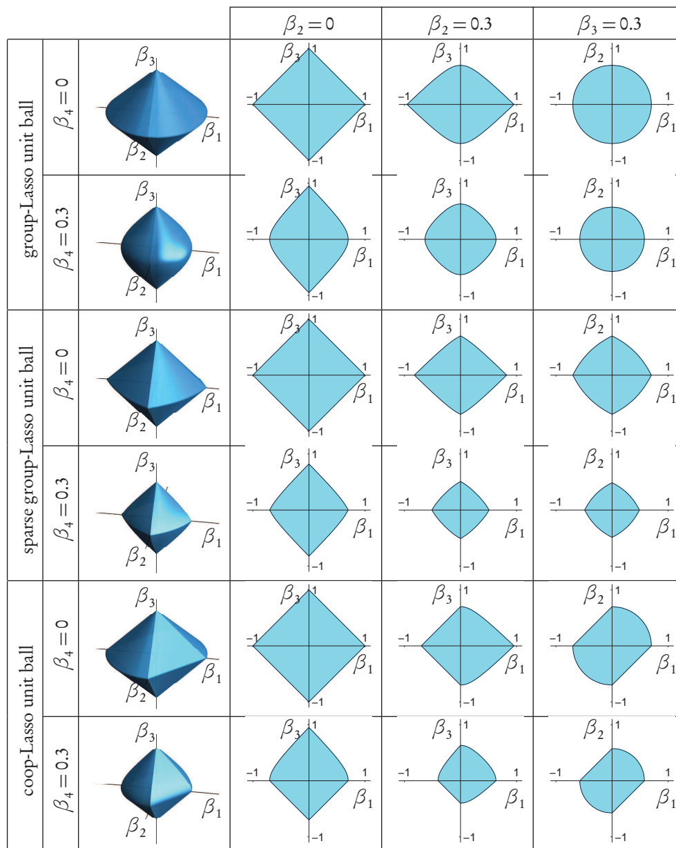
Figure 3.9 – Feasible sets for the coop-Lasso, group-Lasso and sparse group-Lasso penalties. First column: cuts through (\beta_1, \beta_2, \beta_3) at \beta_4 = 0 and \beta_4 = 0.3 : (\beta_1, \beta_2) span the horizontal plane and \beta_3 is on the vertical axis; second and third columns: cuts through (\beta_1, \beta_3) at various values of (\beta_2, \beta_4) ; last column: cuts through (\beta_1, \beta_2) at various values of (\beta_3, \beta_4) .
