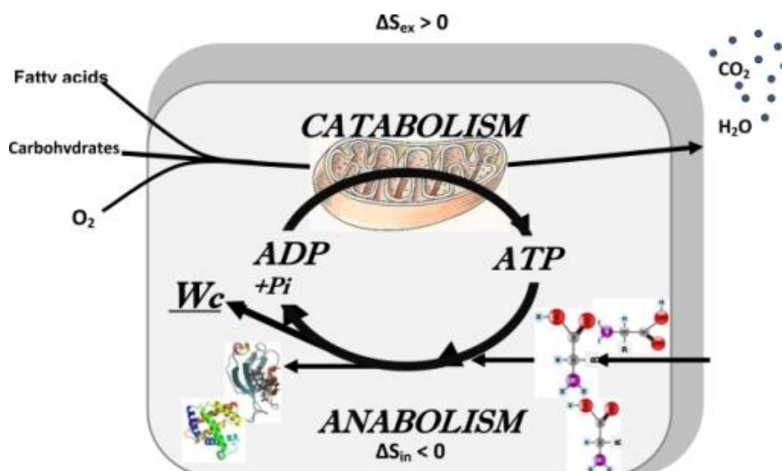
Figure 1. General scheme describing the cellular integrated metabolism as an open system exchanging both energy and mass with surrounding medium (Saks et al., 2007).
