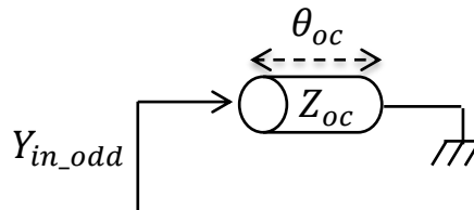
Figure III-2. Odd mode equivalent circuit.
