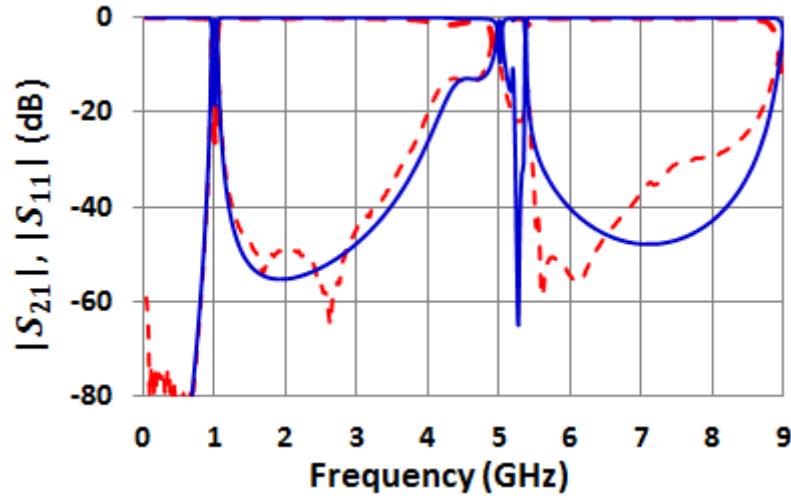
Figure III-23. S parameters of PC-SLR bandpass filter with non-optimized U corner: measurements (red dashed line) and circuit simulations (blue solid line), (a) Narrow band, (b) large band.
