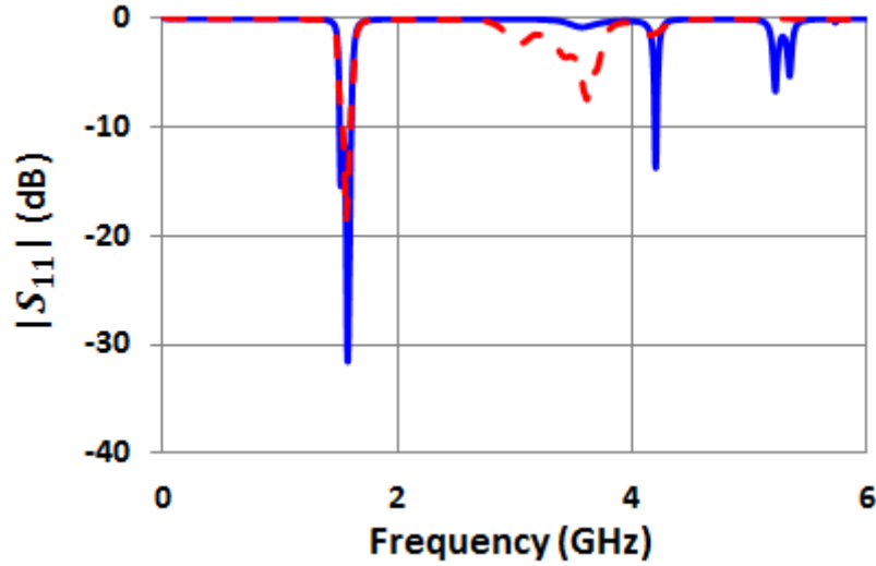
Figure IV-20. S -parameters of the “filter 2”: measurements (red dashed line) (for V_1 = 16.5 V, V_2 = 22 V), and circuit simulations (blue solid line).
