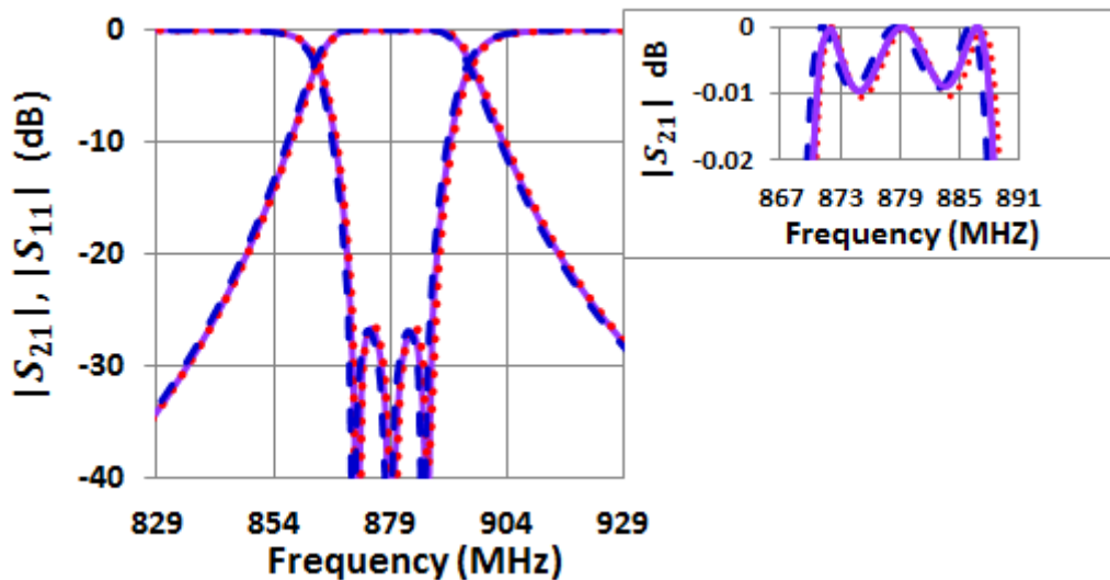
Figure II-11. Comparison of S-parameters simulation of the PC-SLR filters for R_Z = 0.2, \theta_{oc} = 12.3^{\circ} (red dotted line), R_Z = 0.4, \theta_{oc} = 16.7^{\circ} (blue dashed line), and R_Z = 0.6, \theta_{oc} = 19.8^{\circ} (dotted mallow line), for a 2 % relative bandwidth.
