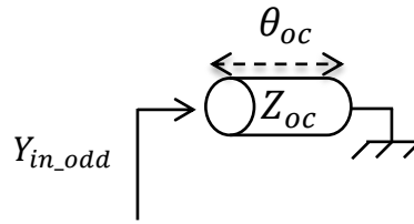
Figure IV-6. Odd-mode equivalent circuit.
