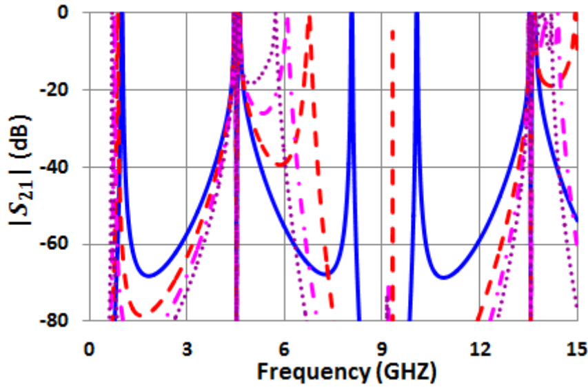
Figure IV-8. S parameters of the PC-SLR bandpass filter based on classical SLR (blue solid line) and compared with three capacitor loaded SLR bandpass filters: for capacitance values, 1 pF (red dashed line), 2 pF (pink dashed dotted line, 3 pF (dotted mallow line)) (a) narrow band (fundamental mode (even-mode)), (b) wide band .
