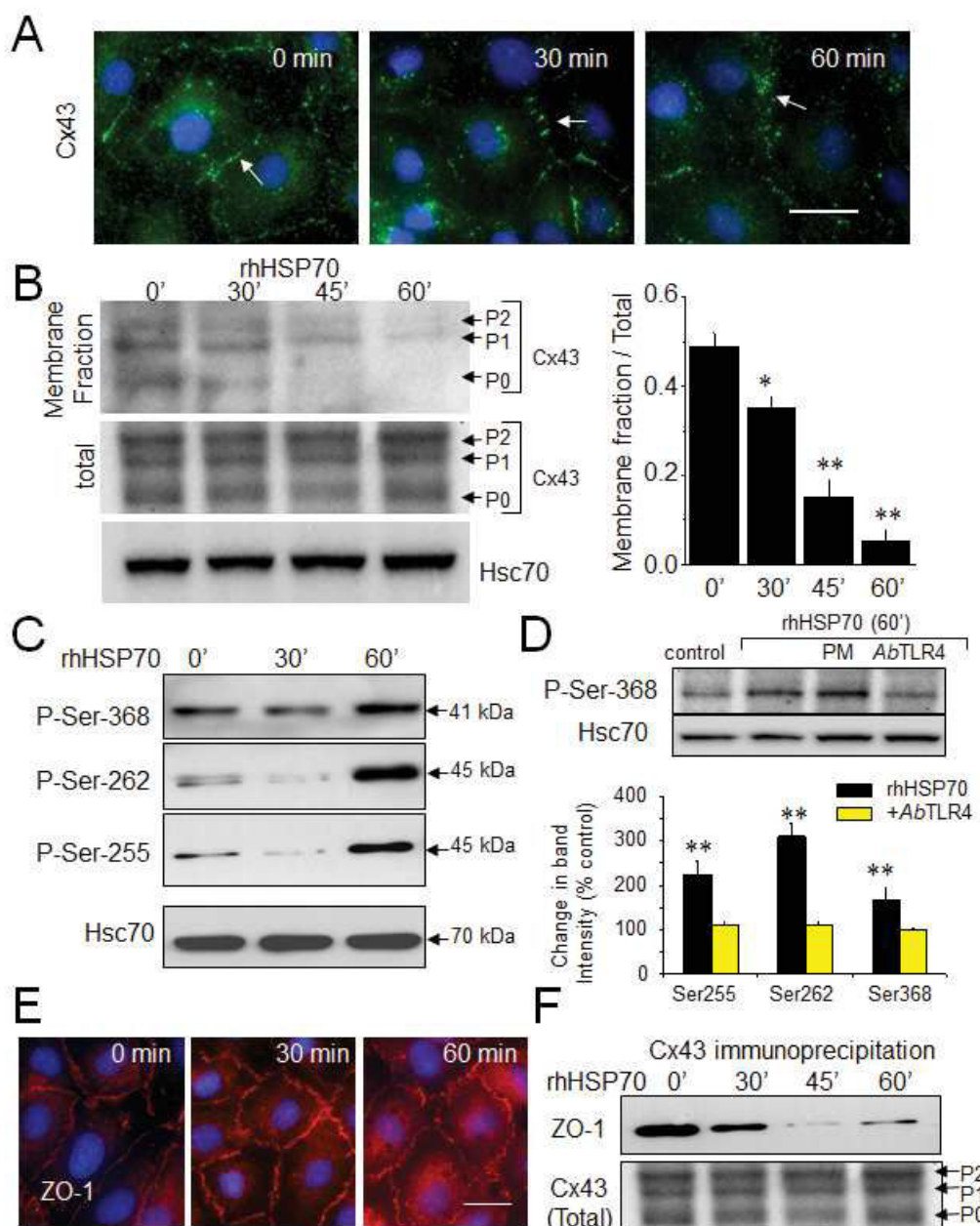
Fig 2: Extracellular rhHSP70 modulates membrane level and phosphorylation of Cx43. A. Immunofluorescence detection of Cx43 (green) in HMEC after treatment with 5 \mu g/ml rhHSP70 for indicated times (DAPI staining of nuclei). Arrows indicate Cx43 plaques. Representative of 5 experiments. Bar 20 \mu m. B. Western blot of the total and membrane fraction (Triton X-100 insoluble) of Cx43. P0, P1 and P2 denotes the three major Cx43 migration bands. Cell membrane lysates immunoblotted for Cx43, after treatment with rhHSP70 for time periods as indicated (Hsc70 as loading control). Right panel shows changes in band intensity of the membrane fraction related to the total Cx43 expression level (mean \pm SD, n=5; **P<0.01, *P<0.05 vs control [t=0 min] in all cases). C. Effect of rhHSP70 on Cx43 phosphorylation pattern. Western blots using three different antibodies against the carboxy terminal part of Cx43 to detect phosphorylation on serine at position Ser262, Ser255 and Ser368 (representative of 5 experiments). D. rhHSP70 leads to phosphorylate Cx43 in a TLR4-dependent manner. Western blot showing phosphorylation on Ser368. When indicated, cells were pre-treated for 60 min with polymyxin B (PMB10 \mu M) or the neutralising anti-TLR4 (AbTLR4 10 \mu g/ml). rhHSP70 was (or not) added for 60 min (representative of 5 experiments). Histogram shows changes in the phosphorylated status of Cx43 in response to 60 min of cell treatment with rhHSP70 (black) or rhHSP70 plus AbTLR4 (grey), expressed as percentage of control (mean \pm SD, n=5; **P<0.01, *P<0.05 vs control). E. Immunofluorescence detection of ZO-1 in HMEC after exposure to rhHSP70 for indicated times. Representative of 5 experiments. Cell nuclei stained with DAPI. Bar 20 \mu m. F. Coimmunoprecipitation of Cx43 and ZO-1 in HMEC, stimulated or not by rhHSP70 for time periods as indicated. The total Cx43 shows slight variations in the unphosphorylated form P0 and the phosphorylated forms P1 and P2 (Hsc70 as loading control; representative of 4 experiments).
