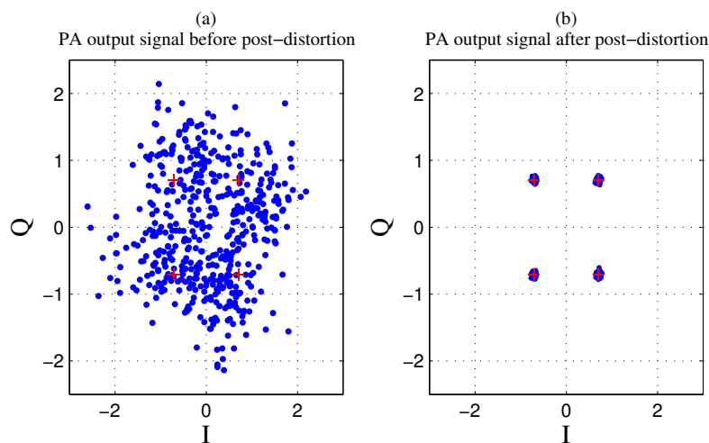
Figure 3.18: Volterra model output signal constellation comparison before and after post-distortion.
