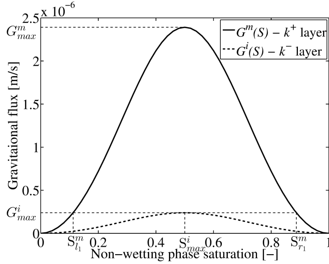
Figure 3.11 – Gravitational flux functions of inclusion and matrix in the case k^i/k^m = 1/10 . G_{max}^i and G_{max}^m are respectively the maximal gravitational flux in the inclusion and the matrix. S_{max}^i is the saturation in the inclusion so that G^i(S_{max}^i) = G_{max}^i . The saturations S_{l_1}^m and S_{r_1}^m satisfy G^m(S_{l_1}^m) = G^m(S_{r_1}^m) = G_{max}^i .
