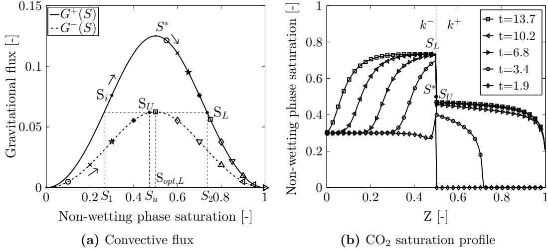
Figure 3.8 – CO 2 migration in a vertical column filled with a piecewise homogeneous porous medium : Case (2b) the lower sub-domain is more permeable than the upper sub-domain with a high imposed saturation
