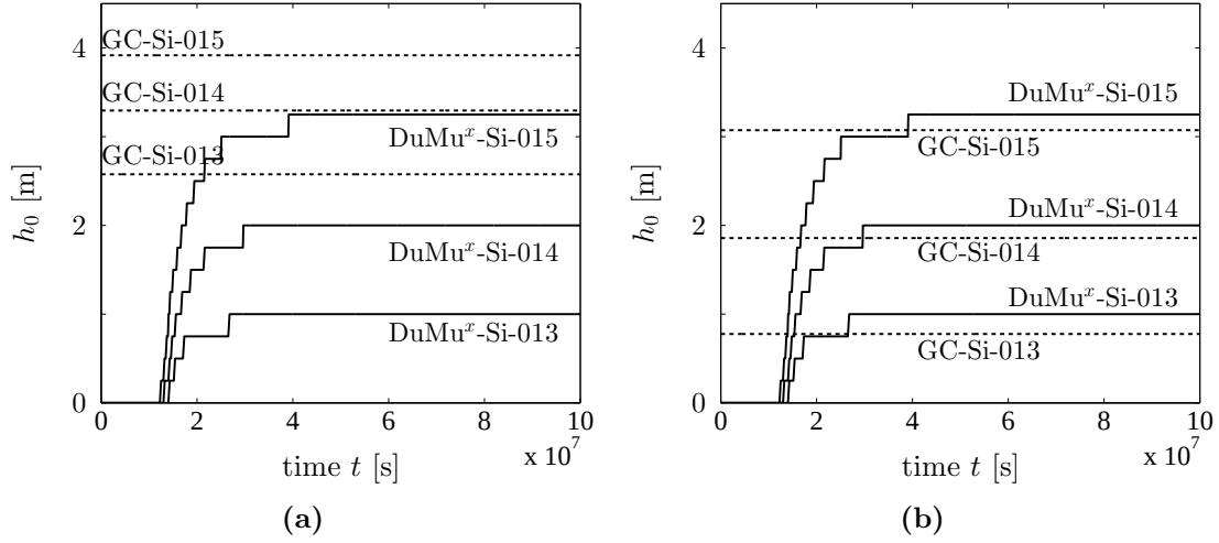
Figure 3.15 – Case 3 - Capillary-free case : maximal gravity current height at the origin h_0 . Comparison between numerical simulation result obtained with DuMu x (continuous lines) and analytical gravity current models without (a) and with (b) the total velocity fluctuation.
