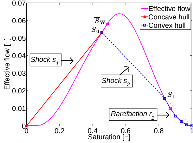
Figure 2.10 – Balance case - imposed CO 2 saturation at the bottom of the column : construction of the concave and convex hull for effective flux function with N_c = \varepsilon and k^-/k^+ = 1/2
