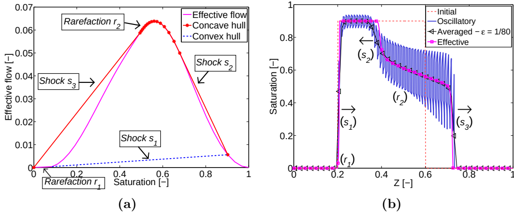
Figure 2.11 – Balance case - CO 2 plume : (a) Construction of the concave and convex hull for effective flux function. (b) Evolution of CO 2 plume in stratified medium and the equivalent homogeneous medium at t=1 .
