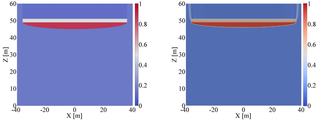
Figure 3.13 – Case 3 - Capillary-free case : CO 2 distribution from z = 0 [m] to the observation surface z = 60 [m] reconstructed using gravity current method (left) and simulated with DuMu x (right). A moderate influx associated with S_i = 0.15 is imposed at the medium inlet.
