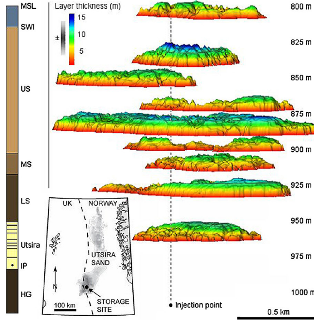
Figure 2.1 – The Sleipner plume profile, viewed from the southeast, circa July 2002. The Figure shows the distribution of injected CO 2 after 5 Mt of injected CO 2 (Bickle et al., 2007). The nine plume layers are well defined aerally, having ponded beneath intra-formational shales within the Utsira Sand. (after Cavanagh and Haszeldine (2014))
