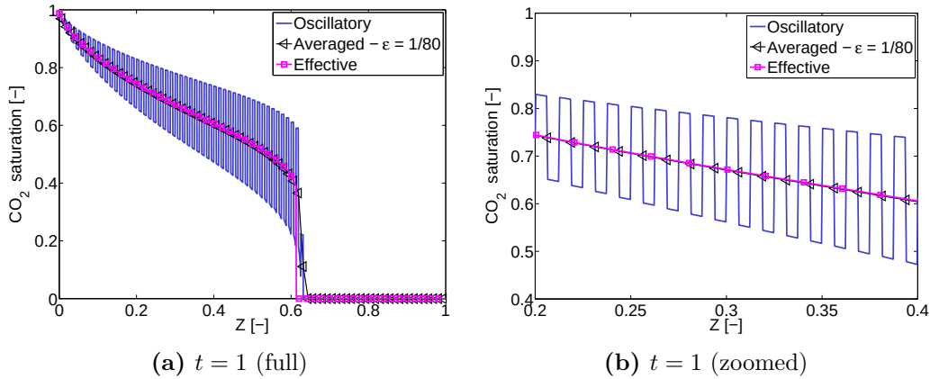
Figure 2.8 – Capillary dominant case - CO 2 injection : CO 2 saturation distribution at time t = 1 , full (a) and zoomed view (b).
