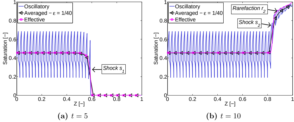
Figure 2.9 – Balance case - imposed \text{CO}_2 saturation at the bottom of the column : \text{CO}_2 saturation distribution at time t = 5 (a) and t = 10 (b).
