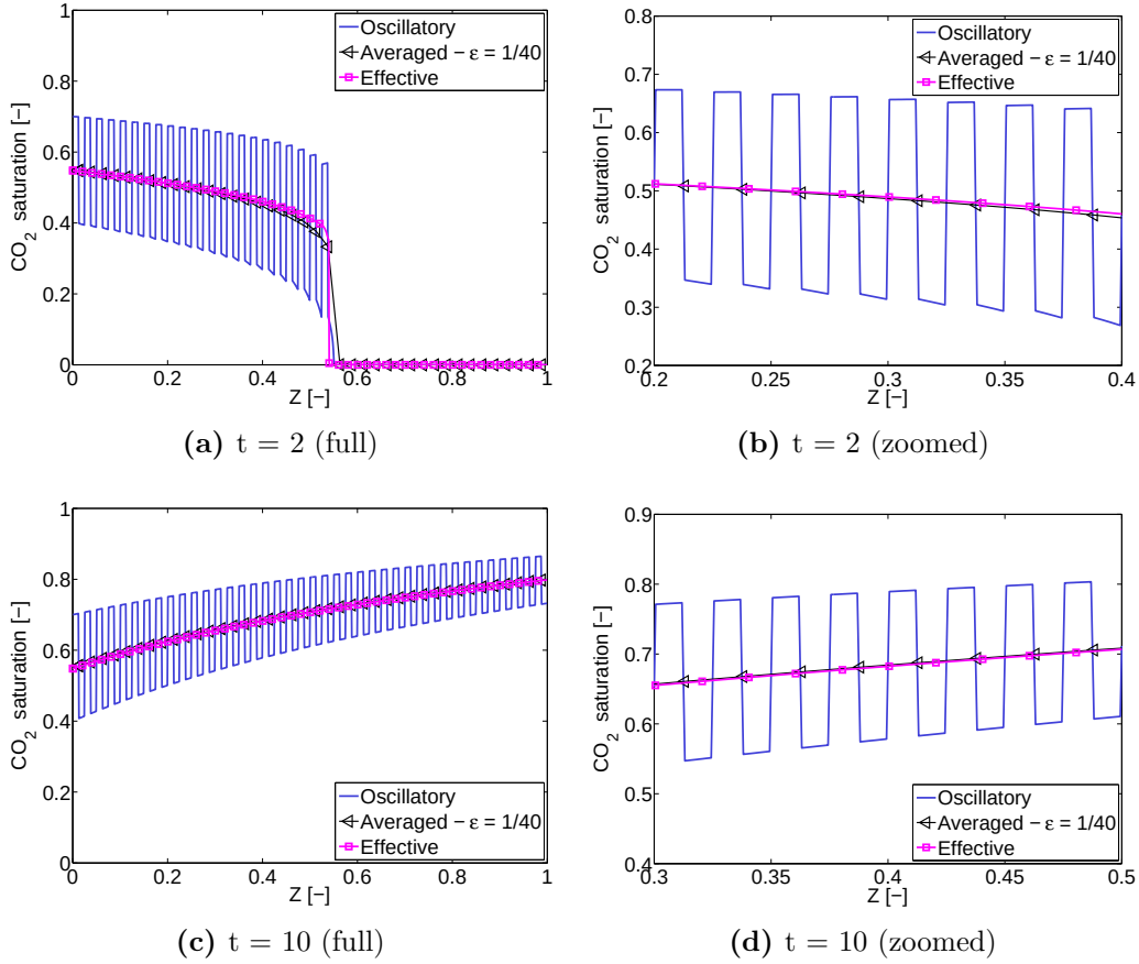
Figure 2.6 – Capillary-dominant case - imposed CO 2 saturation at the bottom of the column : CO 2 saturation distribution at time t = 2 (top) and t = 10 (bottom) with \varepsilon = 1/40 , full (left) and zoomed view (right).
