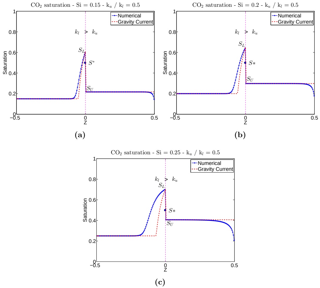
Figure 3.19 – CO 2 saturation profile at steady state for the case k_u/k_l = 0.50 with S_i = 0.15 (a), S_i = 0.20 (b) and S_i = 0.25 (c)
