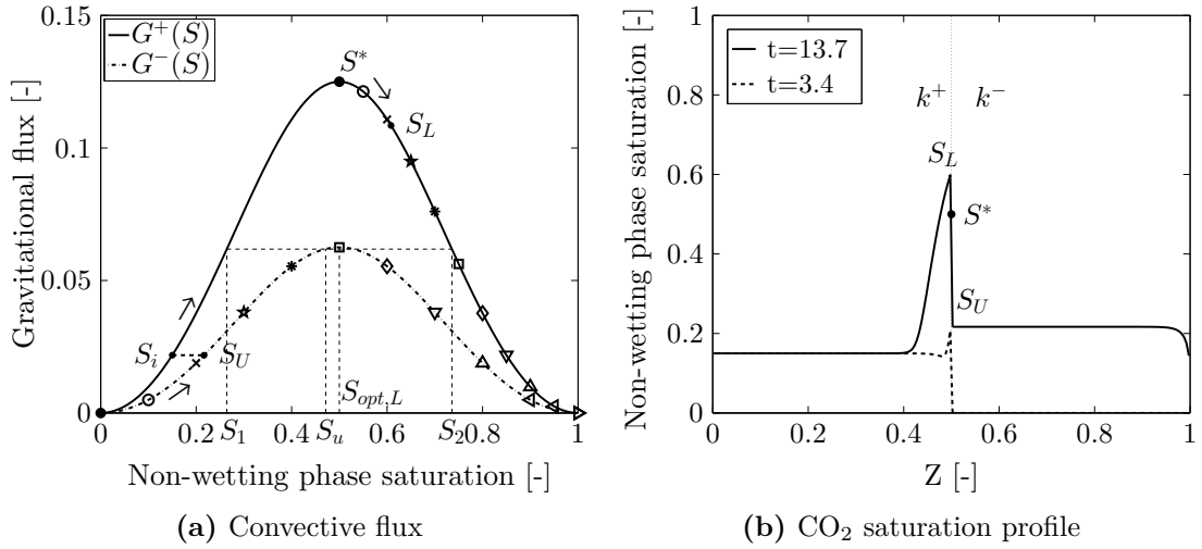
Figure 3.7 – CO 2 migration in a vertical column filled with a piecewise homogeneous porous medium : Case (2a) lower sub-domain is more permeable than upper sub-domain with a low inflow
