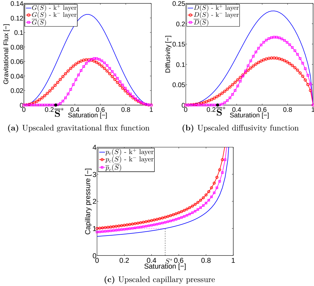
Figure 2.3 – Capillary-dominant case N_c = \mathcal{O}(1) : the upscaled gravitational function \bar{G}(\bar{S}) , the diffusivity function \bar{D}(\bar{S}) and the upscaled capillary pressure function \bar{P}_c(\bar{S}) in the case k^-/k^+ = 1/2 , the threshold saturation is \bar{S}^* = 0.25 .
