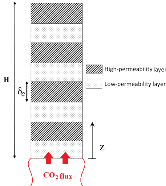
Figure 2.2 – Vertical periodic stratified porous medium.
