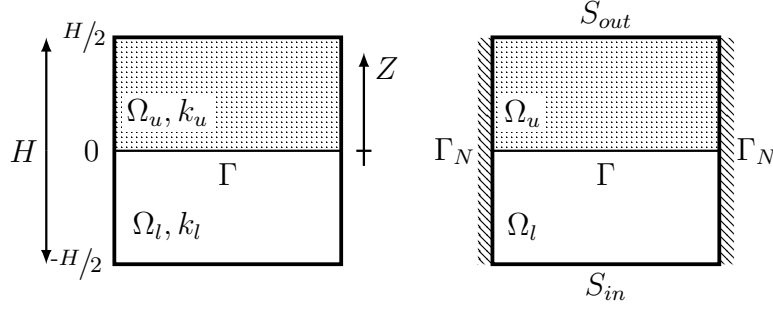
Figure 3.1 – Sketch of the piecewise homogeneous porous medium (left) and boundary conditions (right). The z -axis points upwards.
