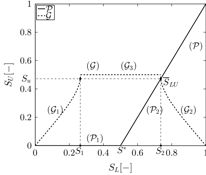
Figure 3.5 – The monotone graph \mathcal{P} (continuous line) is defined by the equation (3.27) from the extended capillary pressure functions \bar{p}_{c_{l,u}} . The curve \mathcal{P} contains two segments : \mathcal{P}_1 for S_L \leq S^* and \mathcal{P}_2 for S_L \geq S^* . The graph \mathcal{G} (dashed line) is defined by equation 22 from the convective flux functions G_{l,u} . The curve \mathcal{P} consists of three segments : \mathcal{G}_1 (from the equation (3.29)), \mathcal{G}_2 (from the equation (3.29) ) and the horizontal segment \mathcal{G}_3 in the case G_l(S_L) \geq \max \{G_u(S_U), S_U \in [0, 1]\} . The intersection point defines the solution of the problem at the steady state, when k^-/k^+ = 1/2 \rightarrow \mathcal{P} \cap \mathcal{G}_2 \equiv \bar{S}_{LU} = (S_2, S_u) . The solution of Buckley-Leverett problem is indeed the optimal entropy solutions S_{opt,U} where G'_u(S_{opt,U}) = 0 (Adimurthi et al., 2004; Andreianov and Cances, 2013).
