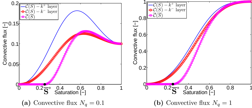
Figure 2.4 – Capillary-dominant case N_c = \mathcal{O}(1) : the effective convective flux function in the case k^-/k^+ = 1/2 , the threshold saturation is \bar{S}^* = 0.25 for N_q = 0.1 (a) and N_q = 1 (b)
