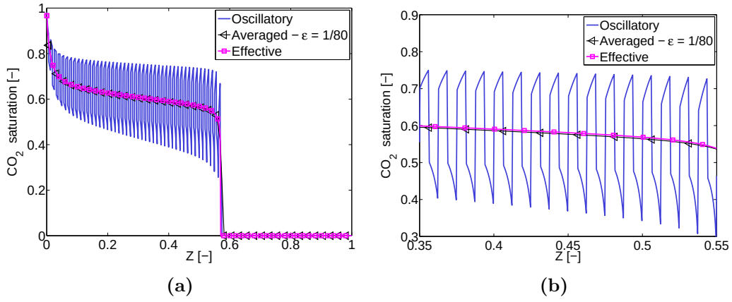
Figure 2.12 – Balance case - low \text{CO}_2 injection : \text{CO}_2 saturation distribution at time t = 2.5 , full (left) and zoomed view (right).
