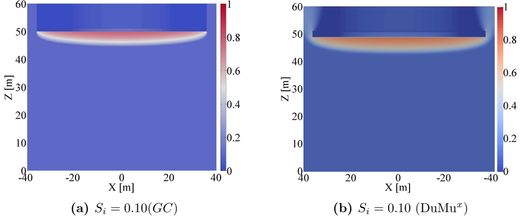
Figure 3.17 – Case 4 - Gravity-dominant case with k^i/k^m = 0.25 and N_c = 0.1 : CO 2 distribution from z = 0 [m] to the observation surface z = 60 [m] reconstructed using gravity current method (left) and simulated with DuMu x (right). A moderate influx S_i = 0.10 is imposed at the bottom of the system.
