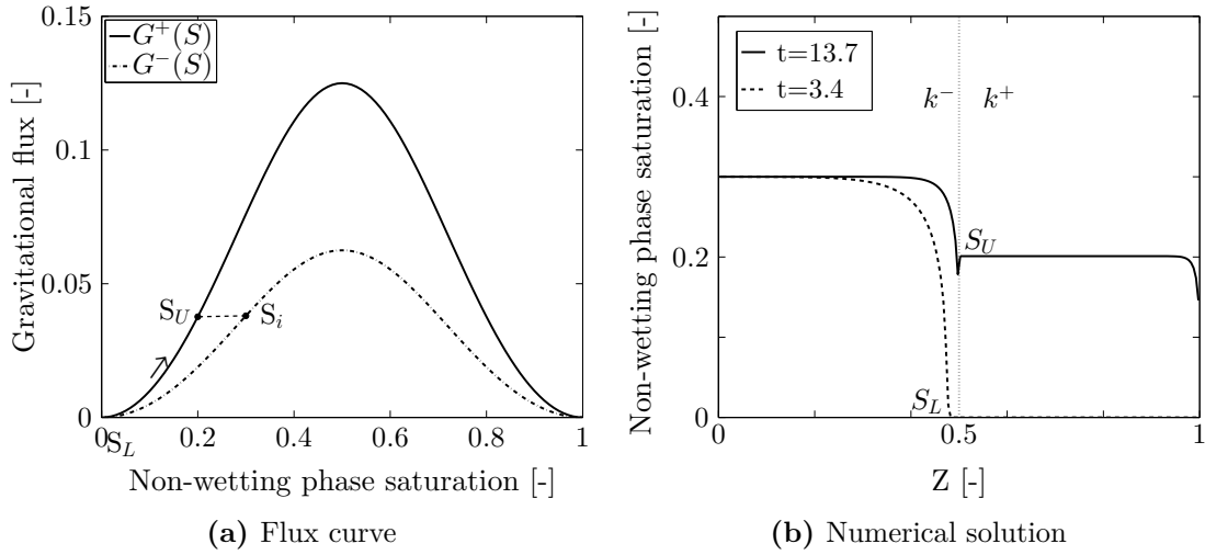
Figure 3.4 – CO 2 migration in a vertical column filled with a piecewise homogeneous porous medium : Case (1) upper sub-domain is more permeable than lower sub-domain.
