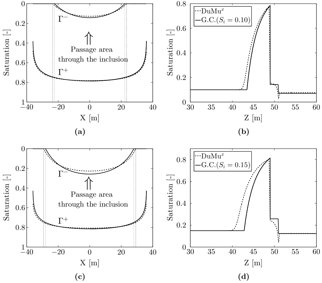
Figure 3.18 – Case 4 - Gravity-dominant case with k^i/k^m = 0.25 and N_c = 0.1 : CO 2 saturation along the horizontal interface \Gamma on the lower matrix side \Gamma_m^- and on the upper inclusion side \Gamma_i^+ (a,c) and along the vertical central axis x=0 from z=0 to the inclusion location (b,d) for the case S_i = 0.10 [m] (top) and S_i = 0.15 [m] (bottom). DuMu x results are represented by dotted lines and the gravity current model by solid lines.
