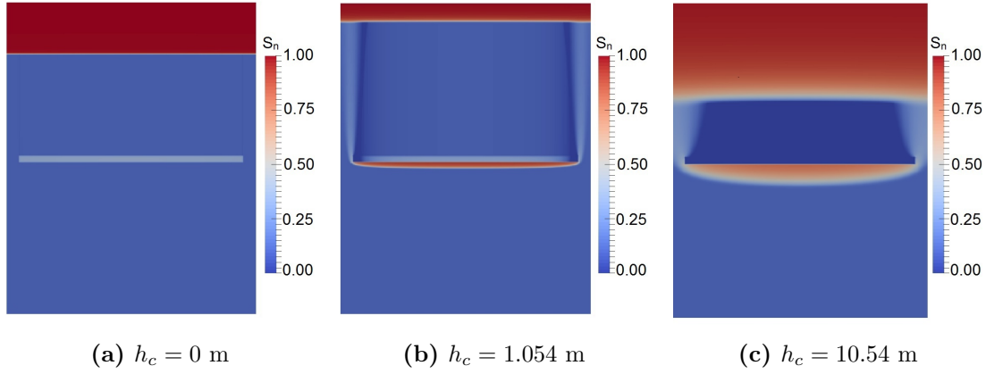
Figure 3.16 – Case 4 - Gravity-dominant case with k^i/k^m = 0.10 and S_i = 0.10 - CO 2 saturation distribution after a long time when CO 2 has reached the upper boundary of the domain. Simulation results are obtained with DuMu x for different values of capillary number : N_c = 0 (left), N_c = 0.01 (medium), N_c = 0.1 (right). The corresponding threshold height of gravity current in the equation (3.45) are h_c = 0, 1.054 and 10.54 respectively.
