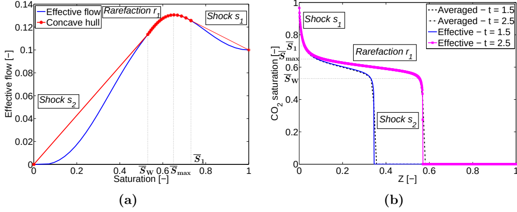
Figure 2.13 – Balance case - CO 2 injection : construction of the concave hulls (a) and CO 2 saturation profile on macroscale at t = 1.5 and t = 2.5 .
