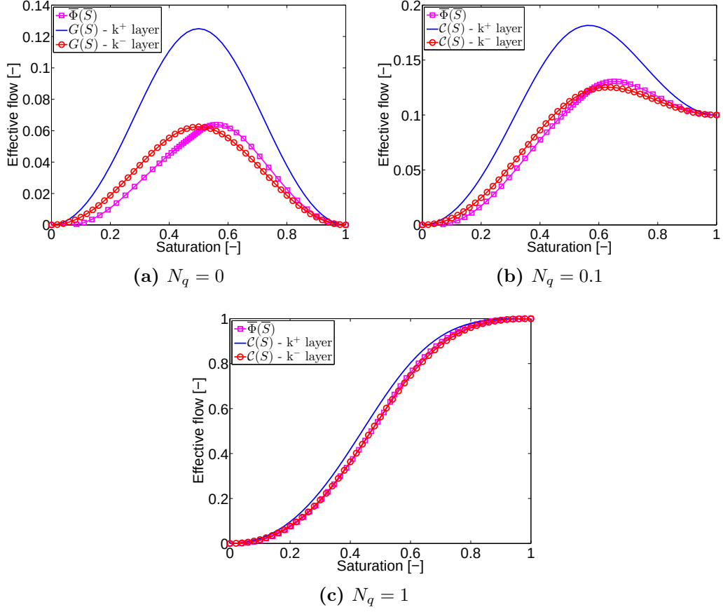
Figure 2.5 – Balance case N_c = \mathcal{O}(\varepsilon) : the effective flux function in the case k^-/k^+ = 1/2 with three values of N_q : N_q = 0 (a), N_q = 0.1 (b) and N_q = 1 (c).
