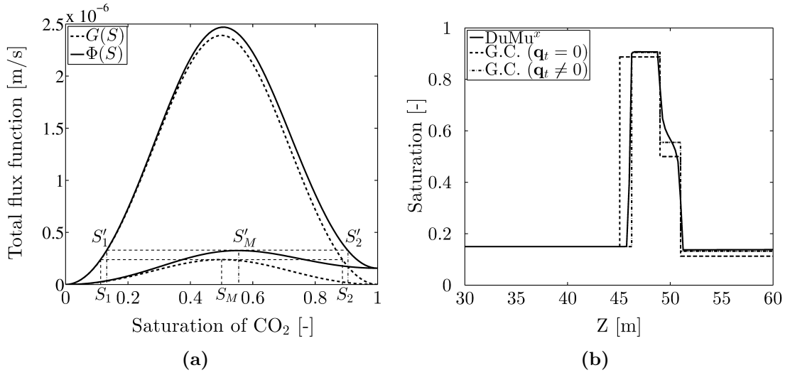
Figure 3.14 – Case 3 - Capillary-free case : (a) Vertical total flux function \Phi(S) and vertical gravitational flux function G(S) along the middle axis at the interface between the matrix and the inclusion ; (b) \text{CO}_2 saturation profile along the middle vertical axis - Comparison between numerical simulation result obtained with DuMu x , analytical gravity current models with and without total velocity fluctuation for the case S_i = 0.15 .
