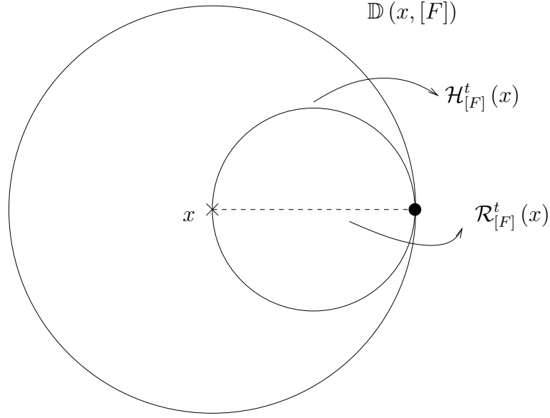
Figure 4.1: The Teichmüller disc \mathbb{D}(x, [F]) . Points of the circle passing through x are horocyclic deformations of x directed by [F] and the dotted segment represents the Teichmüller deformation of x directed by [F] .
