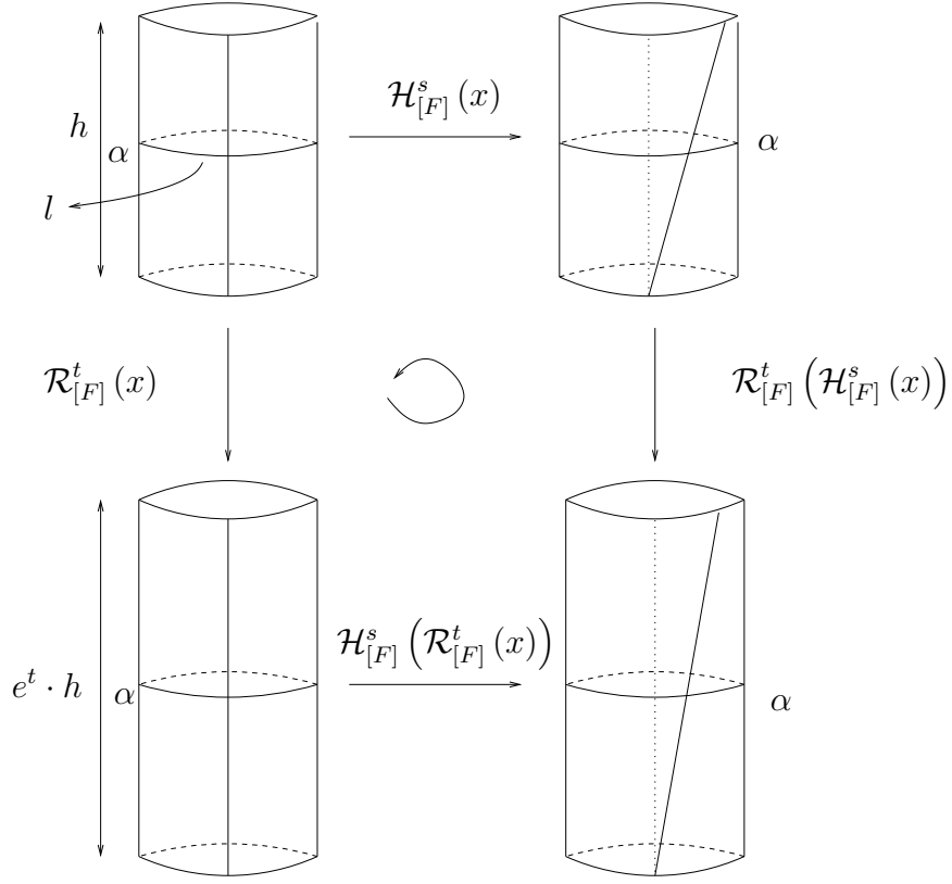
Figure 3.1: Geometric description of a Teichmüller deformation and a horocyclic deformation directed by \alpha \in \mathcal{S} . We have to consider the maximal cylinder of core curve \alpha which gives \text{Ext}_x(\alpha) . The way we identify boundary components depends on the topology of the underlying surface.
