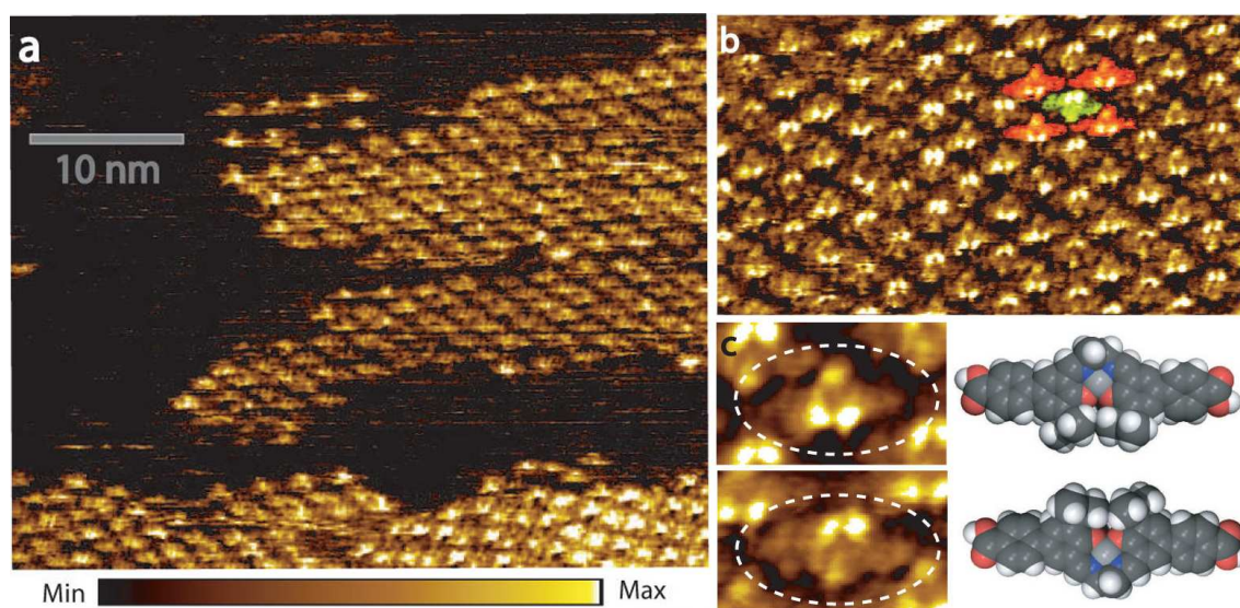
Figure 5.2: (a) Large-scale STM image of the self-assembled structure of molecule 1 on graphite, 45×38nm 2 ; V_s = 0.8 V, I_t = 25 pA. Bottom: color scale bar. (b) High resolution STM image 20×11nm 2 ; V_s=0.8 V, I_t=35 pA. Red and green colored molecules show the two orientations of the molecular building block in the organic layer. (c) Observed molecular orientation. Left: STM images of complex 1 (surrounded by white dotted ellipse). Right: Model of complex 1 . Carbon atoms are dark gray, hydrogen atoms are white, oxygen atoms are red, nitrogen atoms are blue, and nickel atom is light gray, respectively [143].
