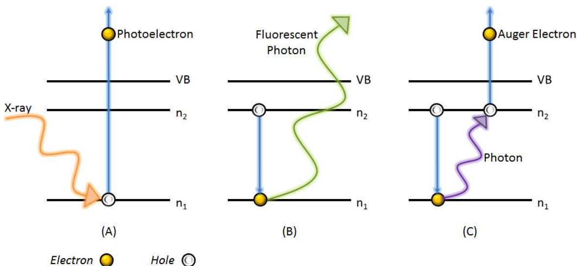
Figure 2.15: The basic principle of NEXAFS spectroscopy: (a) The X-ray absorption followed by the emission of a photoelectron; (b) The fluorescence decay process; (c) The Auger decay process.
