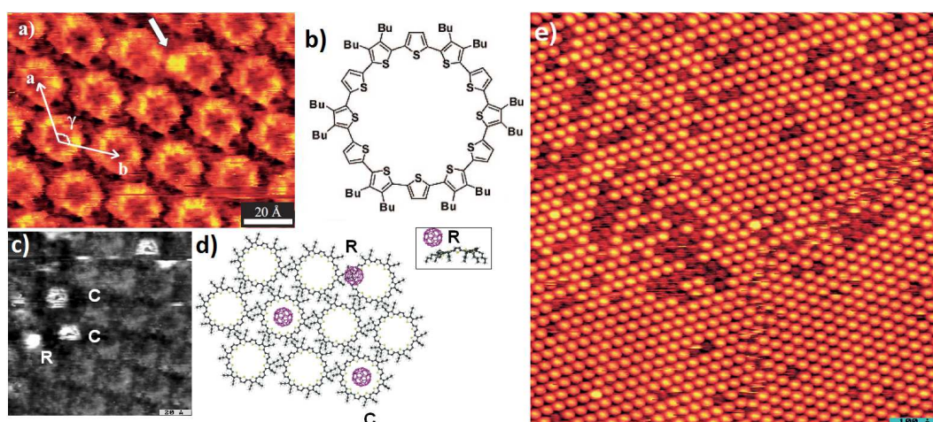
Figure 1.14: a) STM image of a monolayer of C[12]T on HOPG(001), including a C[12]T-C 60 complex (white arrow). Image area: 11.6nm×8.7nm; tunneling conditions: bias voltage V_s=-700 mV, tunneling current I_t=44 pA; b) Scheme of the conjugated macrocycle C[12]T; c) STM image of a monolayer of C[12]T on HOPG and C 60 -fullerenes adsorbed at different sites. Image area: 20nm×20nm; tunneling conditions: V_s=-705 mV, I_t=57 pA. Fullerenes at different adsorption sites are labeled C (cavity) and R (rim). d) Calculated model for the different adsorption sites of the fullerenes on the macrocycle-modified surface (inset, upper right); e) STM image of C[12]T-C 60 complexes, including some non-complexed macrocycles (deep red). Image area: 79nm×79nm; tunneling conditions: V_s=-500 mV, I_t=7 pA, [41].
