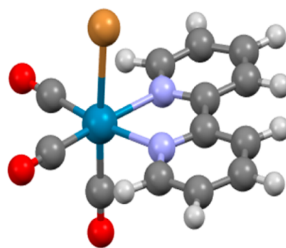
Figure 1. General structure of [\text{Re}(\text{X})(\text{CO})_3(\text{bpy})] (1: X = \text{Cl} ; 2: X = \text{Br} ; 3: X = \text{I} ) complexes.
