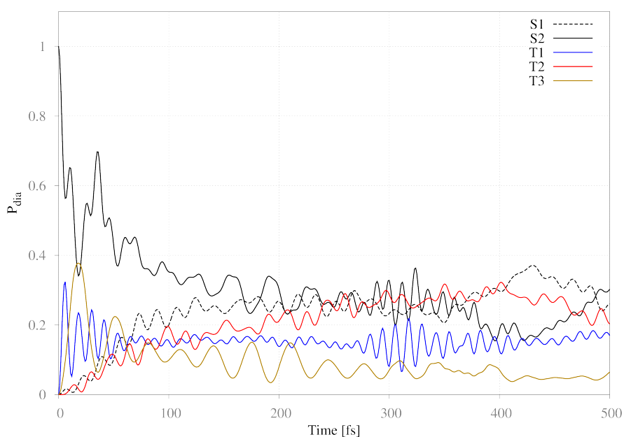
Figure 6.20: Evolution of the diabatic populations as function of time after initial excitation in S2 for the [Re(Br)(CO)_3(bpy)] complex including vibronic coupling (for convenience the population in all spin components of each triplet state are summed over).
