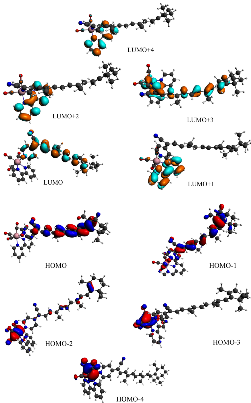
Figure 5.4: Kohn-Sham orbitals of \text{cis-}[\text{Re}(\text{CO})_3(\text{bpy})(\text{L})]^+ 1c conformer in acetonitrile.
