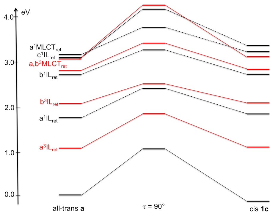
Figure 5.6: TD-DFT states correlation diagrams connecting the low-lying singlet and triplet excited states of all- trans [Re(CO)_3(bpy)(L)]^+ a to the corresponding states of the cis 1c isomer. (energies are reported in APPENDIX TAB. A.12.)
