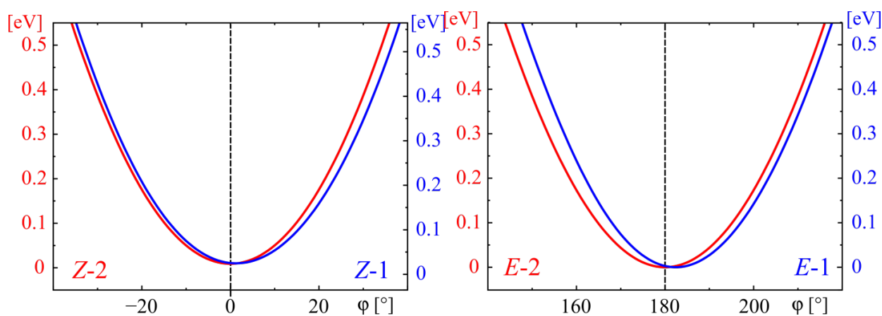
Figure S7. S_0 potential energy curves computed as a function of the torsion angle with all other coordinates fixed at their FC values, for the chiral (1, blue) and achiral (2, red) and compounds. Left: Z isomers; Right: E isomers.
