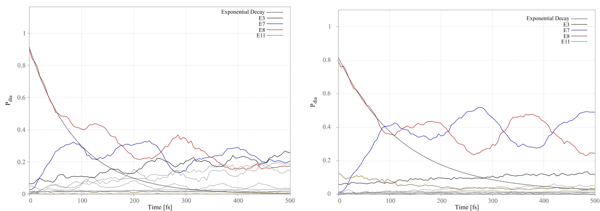
Figure 6.24: Evolution of the adiabatic populations as function of time after initial excitation in the diabatic S2 state for: [\text{Re}(\text{F})(\text{CO})_3(\text{bpy})] (on the left), and [\text{Re}(\text{Cl})(\text{CO})_3(\text{bpy})] (on the right) (low populated states in gray).
