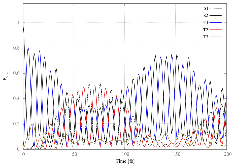
Figure 6.25: Evolution of the diabatic populations as function of time after initial excitation in S2 state for: [\text{Re}(\text{I})(\text{CO})_3(\text{bpy})] .
