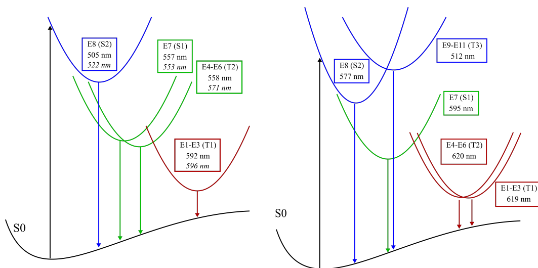
Figure 6.10: Qualitative representation of the mechanism of decay after absorption of [\text{Re}(\text{Cl})(\text{CO})_3(\text{bpy})] , [\text{Re}(\text{Br})(\text{CO})_3(\text{bpy})] (left) and [\text{Re}(\text{I})(\text{CO})_3(\text{bpy})] (right). The color code used is the same as in FIG. 6.8. In blue, states involved in the first emission band; in green, those involved in the second band and in red, states involved in the third emission band.
