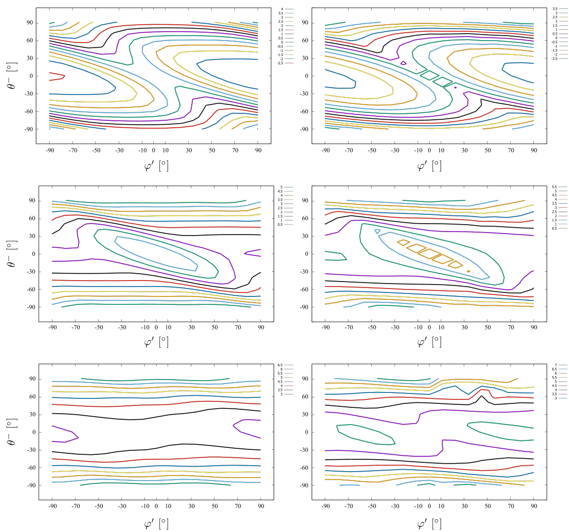
Figure 3.27: Left: fitted adiabatic PES, from top to bottom: S0, S1, S2. Right: computed adiabatic PES, from top to bottom: S0, S1, S2.
