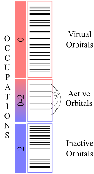
Figure 1.4: The CASSCF subdivision of the total orbital space.
