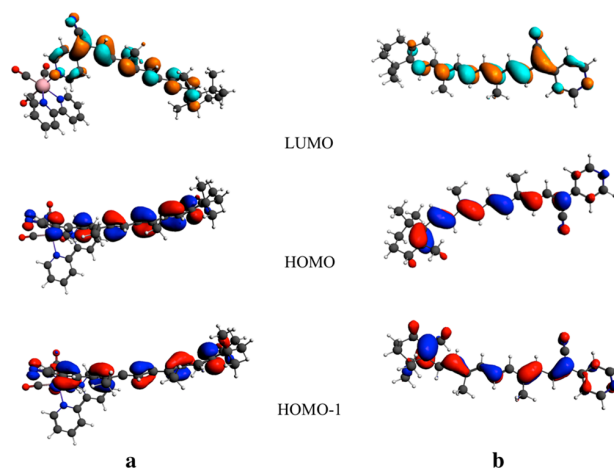
Scheme 4. Comparison between the Frontiers Kohn–Sham Orbitals of the All- trans - [\text{Re}(\text{CO})_3(\text{bpy})(\text{L})]^+ and of the Isolated Retinal-Like Ligand b
