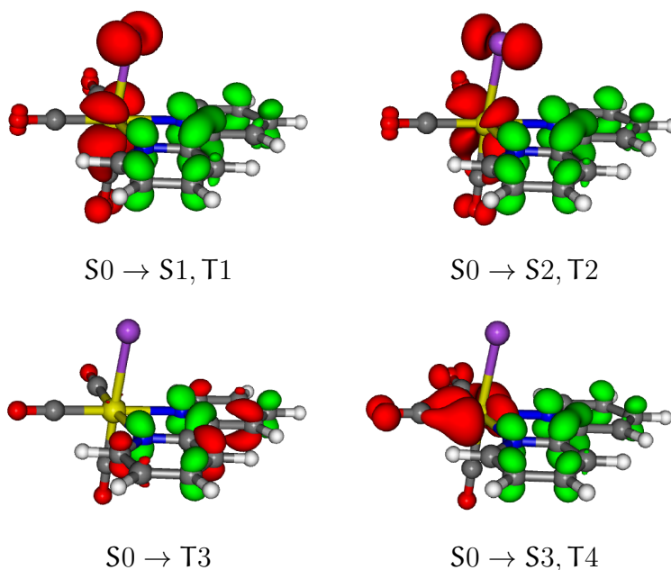
Figure 6.5: Differences in electronic densities between the electronic ground state and the lowest electronic excited "SOC-free" states of [Re(Br)(CO) 3 (bpy)]. (In green: increase of electronic density; in red: decrease.)
