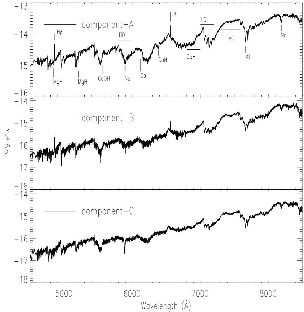
Figure 4.2 – Optical Spectra of all the components of LHS 1070 system obtained with the Faint Object Spectrograph (FOS) on HST. The atomic and molecular features visible in all three components are shown in the upper panel.
