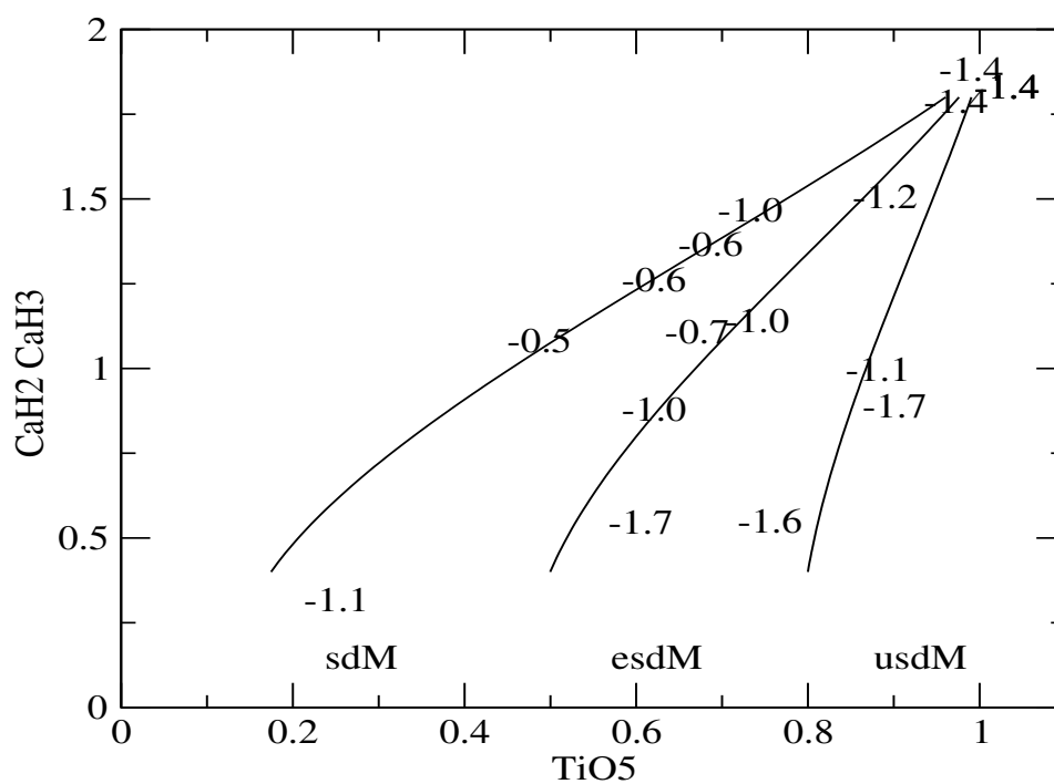
Figure 6.10 – CaH2+CaH3 versus TiO5 diagram for our sample. The labels indicate our metallicity determination. The lines are defined by Lépine et al. (2007). They show the different regions in the diagram where sdM, esdM, and usdM stars are expected.
