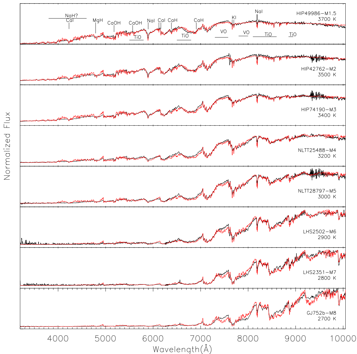
Figure 5.4 – Optical to red SED of M dwarfs from M1 to M8 observed with the SSO 2.3 m at a spectral resolution of 1.4 \text{ \AA} compared to the best fitting (chi-square minimization) BT-Settl synthetic spectra (red lines). The models displayed have a surface gravity of \log g = 5.0 to 5.5 . At blue wavelengths ( < 5000 \text{ \AA} ) the instrumental noise dominates the late-type M dwarfs.
