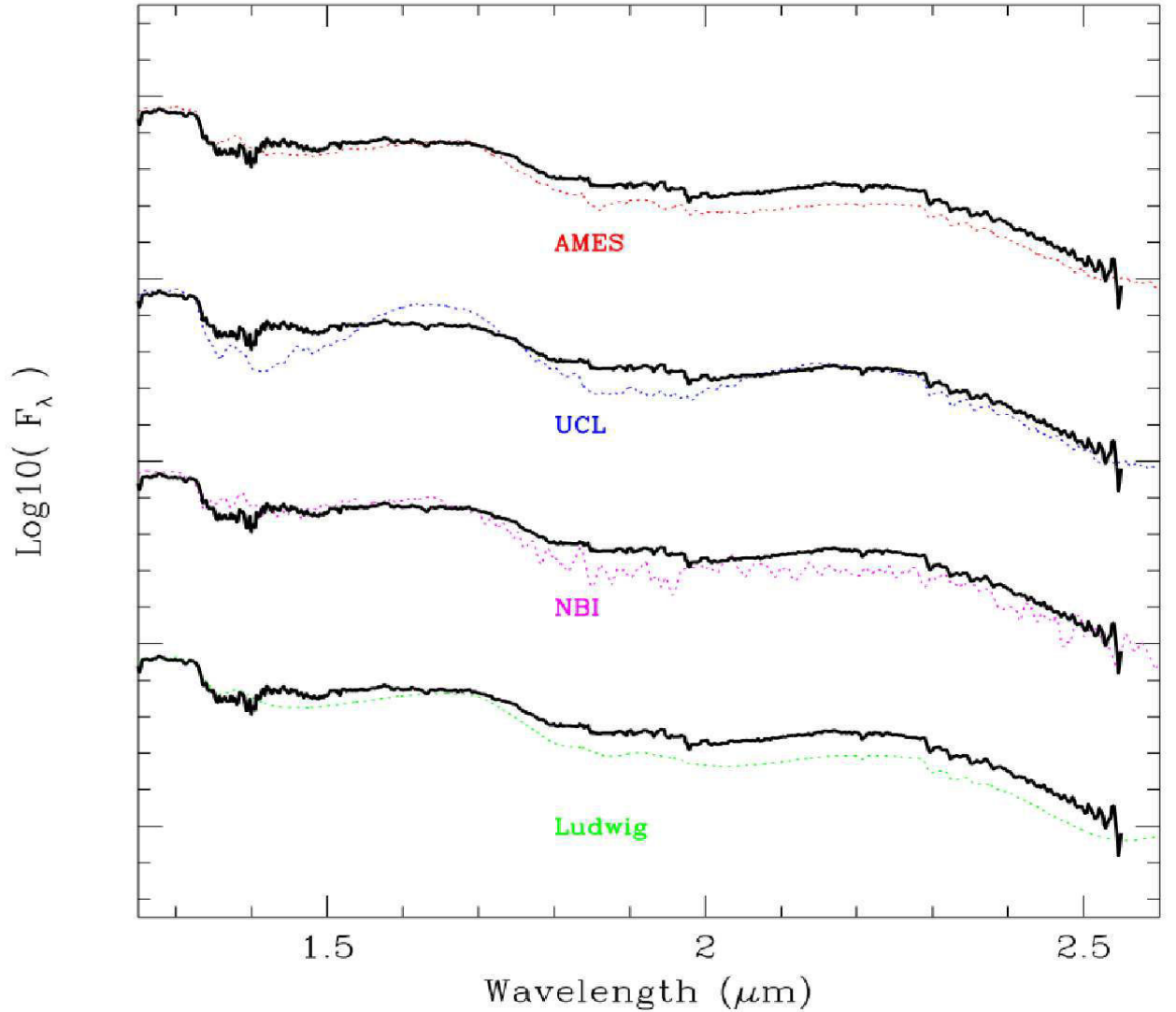
Figure 3.1 – Fig. 1 of the review article by Allard et al. (2012a). The near-infrared SED of VB10 is compared with the synthetic spectra ( T_{\text{eff}} = 2800 \text{ K} , \log g = 5.0 , [M/H] = 0.0 ) from diverse model grids published through the years. All models (except the NextGen / UCL case) underestimate the flux in the K bandpass by 0.1 to 0.2 dex
