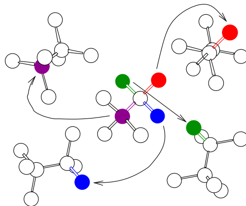
Figure 2.5: Look up configurations, from [Martin-Bragado & Sklenard 2012]. The center shows the substrate configuration surrounded by its twins. The twins are formed by the 60^\circ rotation around one bond of the tetrahedron, and are displayed with different colors.
