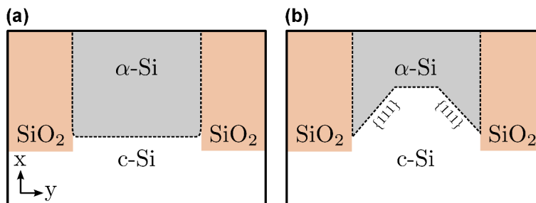
Figure 2.17: Schematic cross-section of the regrowth of a trench-bounded amorphous region: (a) after amorphization by ion-implantation and (b) after an incomplete recrystallization leading to the formation of \{111\} planes.
