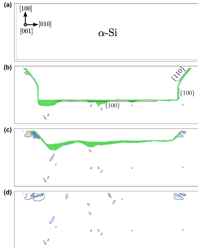
Figure 2.29: Simulation snapshots of recrystallization of \langle 100 \rangle -aligned box-shaped amorphized regions in Si(001) at different stages of the anneal at 550 °C: (a) initial structure, (b) after 100 s, (c) after 200 s, and (d) after 480 s (complete regrowth has been achieved).
