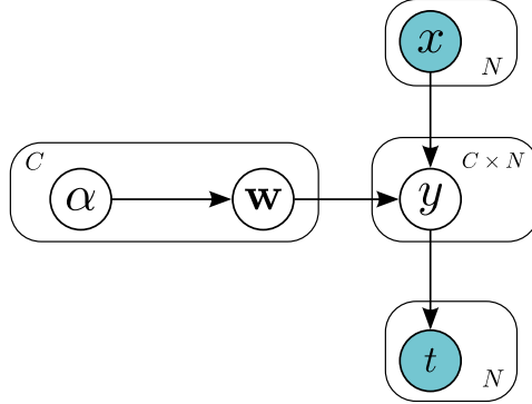
Figure 5.4: Graphical representation of the mRVM. Note that \alpha and w are (N + 1) -dimensional.
