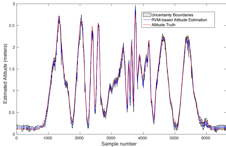
Figure 6.15: Altitude estimation with heteroscedastic noise models and mRVM based measurement selection.
