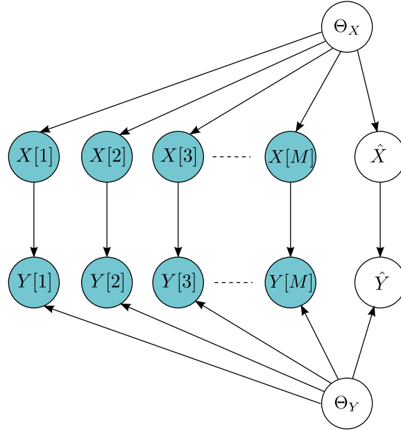
Figure 2.6: Ground Bayesian Network of a two-variable model: each instance \{X[i], Y[i]\} within the training set is depicted as an independent sample, along with the predicted samples \{\hat{X}, \hat{Y}\} . Note that the parameters \Theta = \{\Theta_X, \Theta_Y\} are shared by all instances of X and Y .
