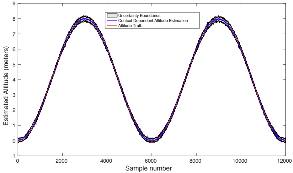
Figure 5.8: Estimated altitude on the validation dataset for the refined model (5 observation functions corresponding to \{[y^1], [y^3], [y^1y^2], [y^2y^3], [y^1y^2y^3]\} ).
