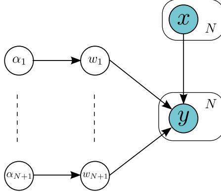
Figure 5.1: Graphical representation of the RVM regression model.
