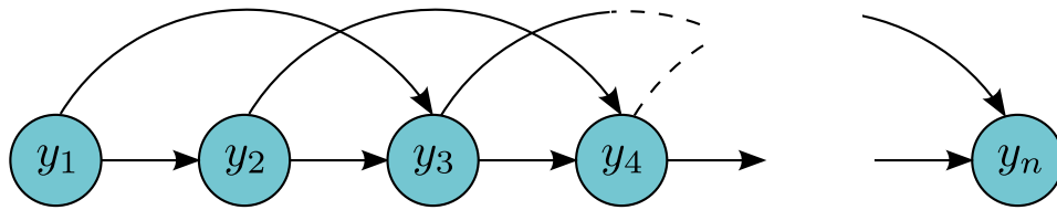
Figure 2.5: Second-order Markov chain graphical model.
