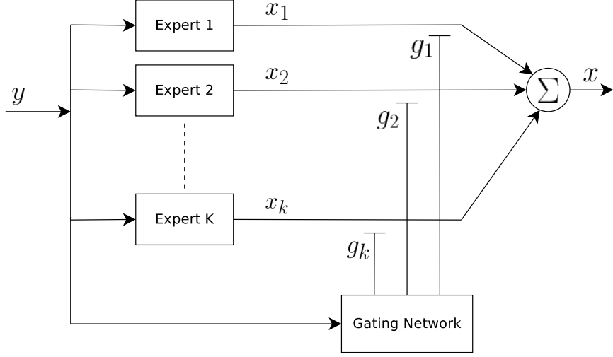
Figure 4.4: The basic mixture of experts framework.
