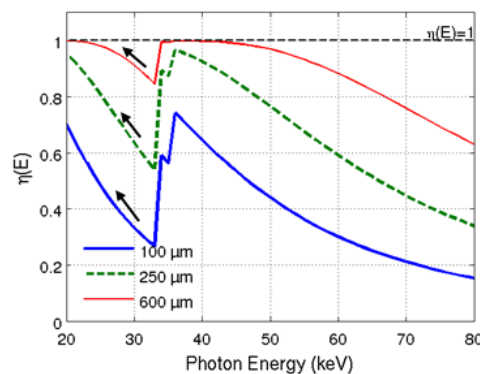
Figure 5-21: Absorption efficiency \eta(E) as function of incident photon energy E for 100, 250 and 600 \mu\text{m} CsI thicknesses
