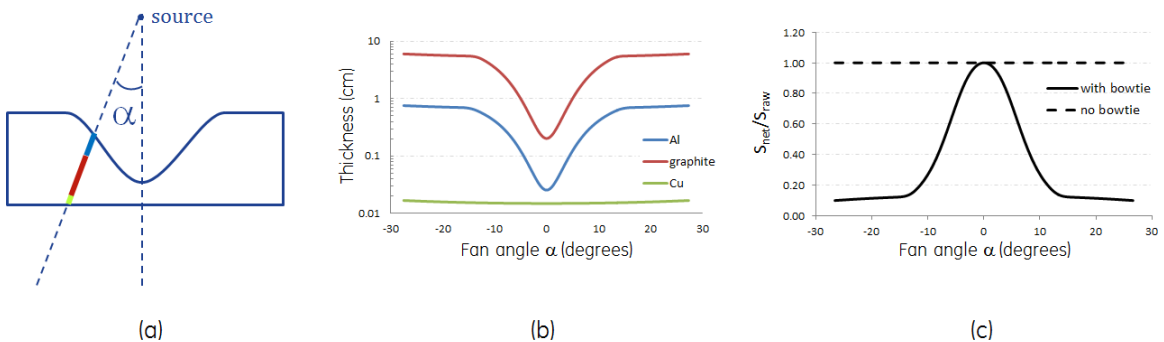
Figure 2-3: (a) Bowtie filter illustration combining three materials (aluminum, graphite and copper); (b) a given thickness profile for the three materials as function of the fan angle \alpha , as well as the (c) resulting transmission factor for a given beam energy
