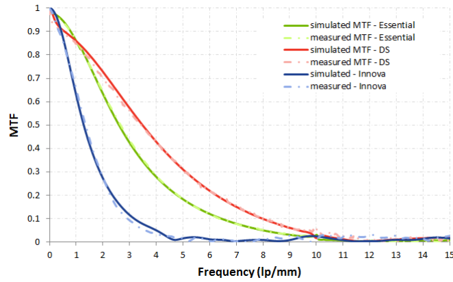
Figure 3-18: Measured and simulated Modulation Transfer Function (MTF) for the three considered X-ray systems
