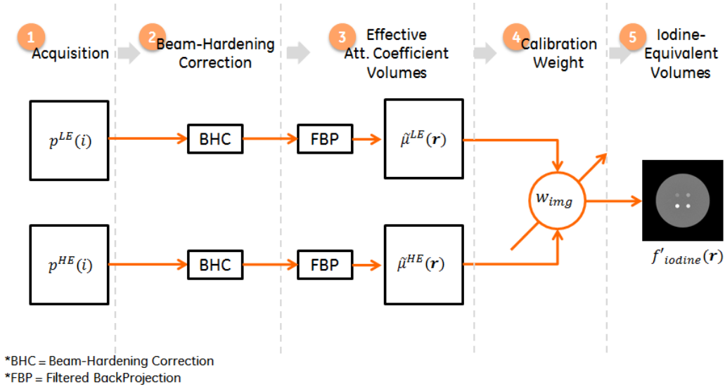
Figure 4-2: Flowchart of image-based decomposition
