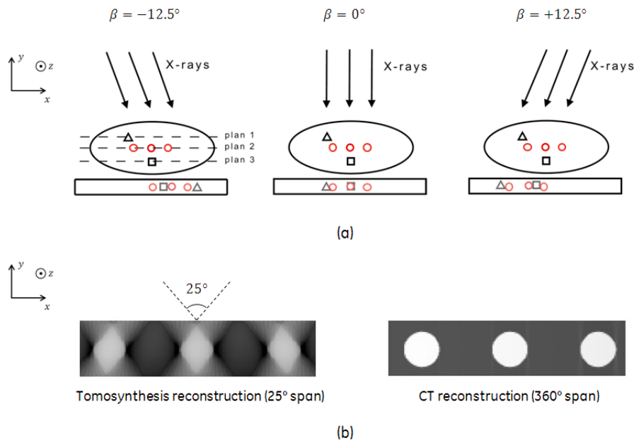
Figure A-8: (a) Illustration of tomosynthesis reconstruction with Shift-and-Add algorithm; (b) example of geometric deformation in the y-axis when the spheres in plane 2 are reconstructed using 25^\circ angular span, when compared to a full 360^\circ circular orbit
