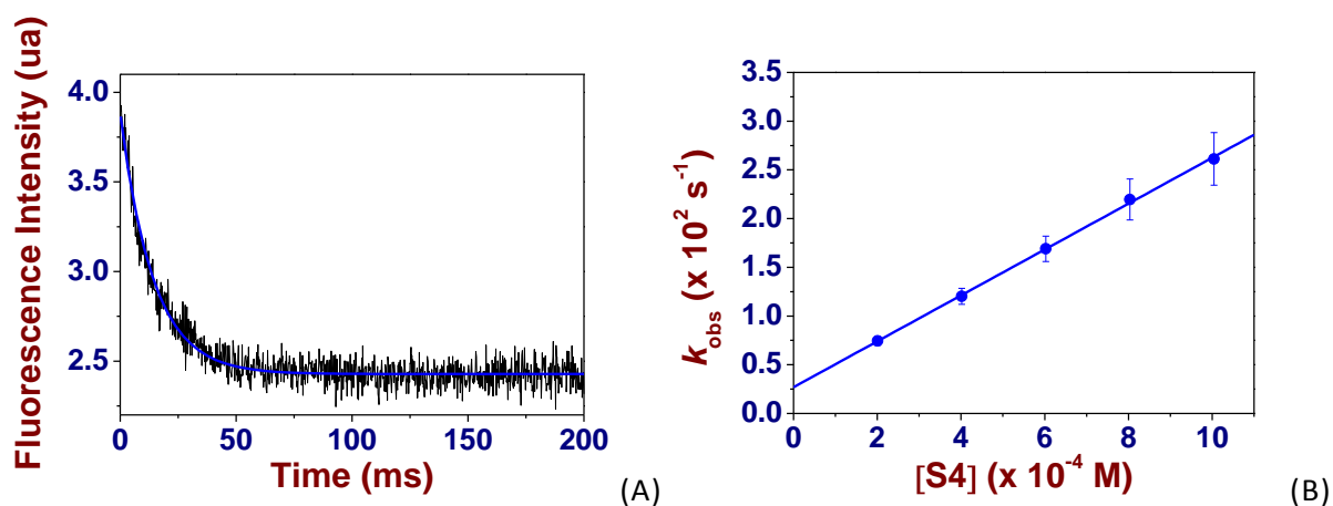
Figure 12. (A) Variation of the luminescence intensity versus time for the formation of \text{ZnL}^1\text{.ABI} complex. Solvent: 1,2-dichloroethane; T = 25.0(2) \text{ }^\circ\text{C} ; l = 1 \text{ cm} ; [\text{ZnL}^1] = 1.07 \times 10^{-5} \text{ M} ; [\text{ABI}]_0/[\text{ZnL}^1]_0 = 10.43 . \lambda_{\text{exc}} = 554 \text{ nm} ; set of band pass filter ( \lambda > 550 \text{ nm} ). (B) Variation of the pseudo-first order constants k_{\text{obs}} ( \text{s}^{-1} ) for the formation of \text{ZnL}^1\text{.ABI} complex versus [\text{ABI}]_{\text{tot}} . Solvent: 1,2-dichloroethane; T = 25.0(2) \text{ }^\circ\text{C} ; [\text{ZnL}^1] = 1.07 \times 10^{-5} \text{ M} .
