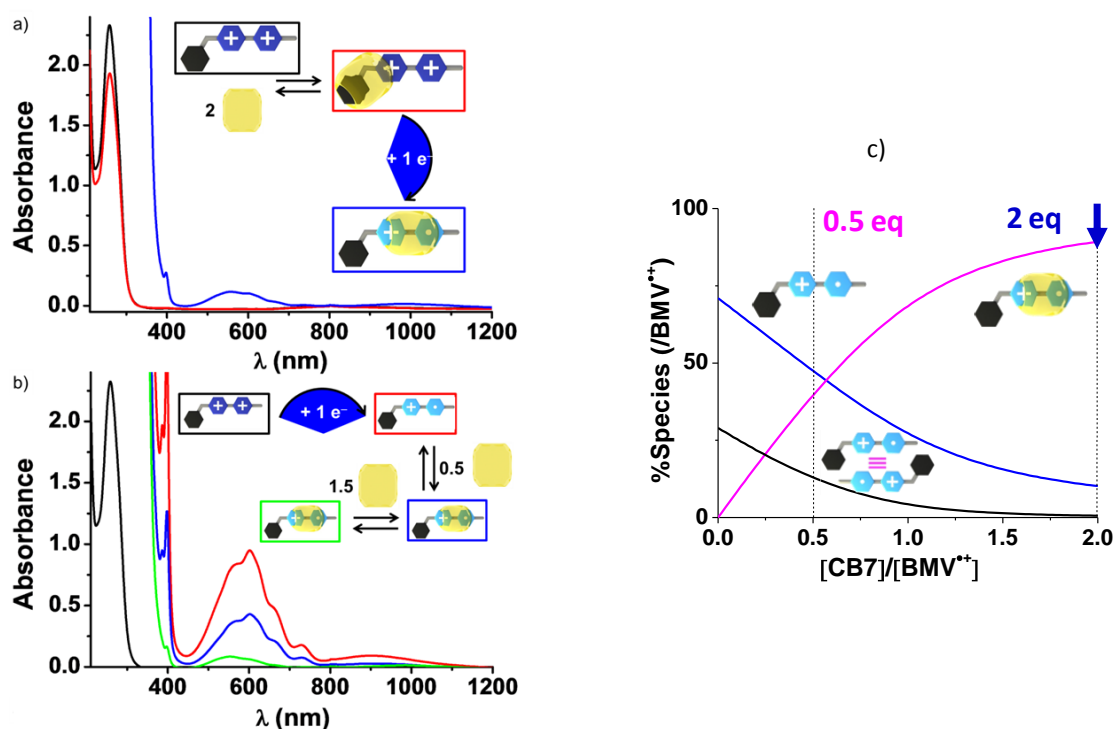
Figure 20. (A) UV-Vis-NIR spectra of \text{BMV}^{2+} ( [\text{BMV}^{2+}]_0 = 10^{-4} M, black line) and of its \text{BMV}^{2+}\text{CB}[7] complex ( [\text{BMV}^{2+}]_0 = 10^{-4} M and [\text{CB}[7]]_0 = 2 \times 10^{-4} M, red line). (B) UV-Vis-NIR spectra of \text{BMV}^{2+} ( [\text{BMV}^{2+}]_0 = 10^{-4} M, black line), of its monoradical cationic species \text{BMV}^{\bullet+} (red line, addition of freshly prepared and \text{O}_2 -free sodium dithionite) and upon addition of \text{CB}[7] ( [\text{CB}[7]]_0 = 5 \times 10^{-5} M, blue line and [\text{CB}[7]]_0 = 2 \times 10^{-4} M, green line). (C) Distribution diagrams of the \text{BMV}^{\bullet+}/\text{CB}[7] system. Solvent: water buffered at pH 7.0 with 0.1 M \text{Na}_2\text{HPO}_4/\text{NaH}_2\text{PO}_4 ; l = 1 cm; T = 25.0(1) °C. In each of the solutions considered, the \text{BMV}^{\bullet+} species was generated from \text{BMV}^{2+} using freshly prepared sodium dithionite solution at ca. 10^{-2} M under \text{O}_2 free conditions.
